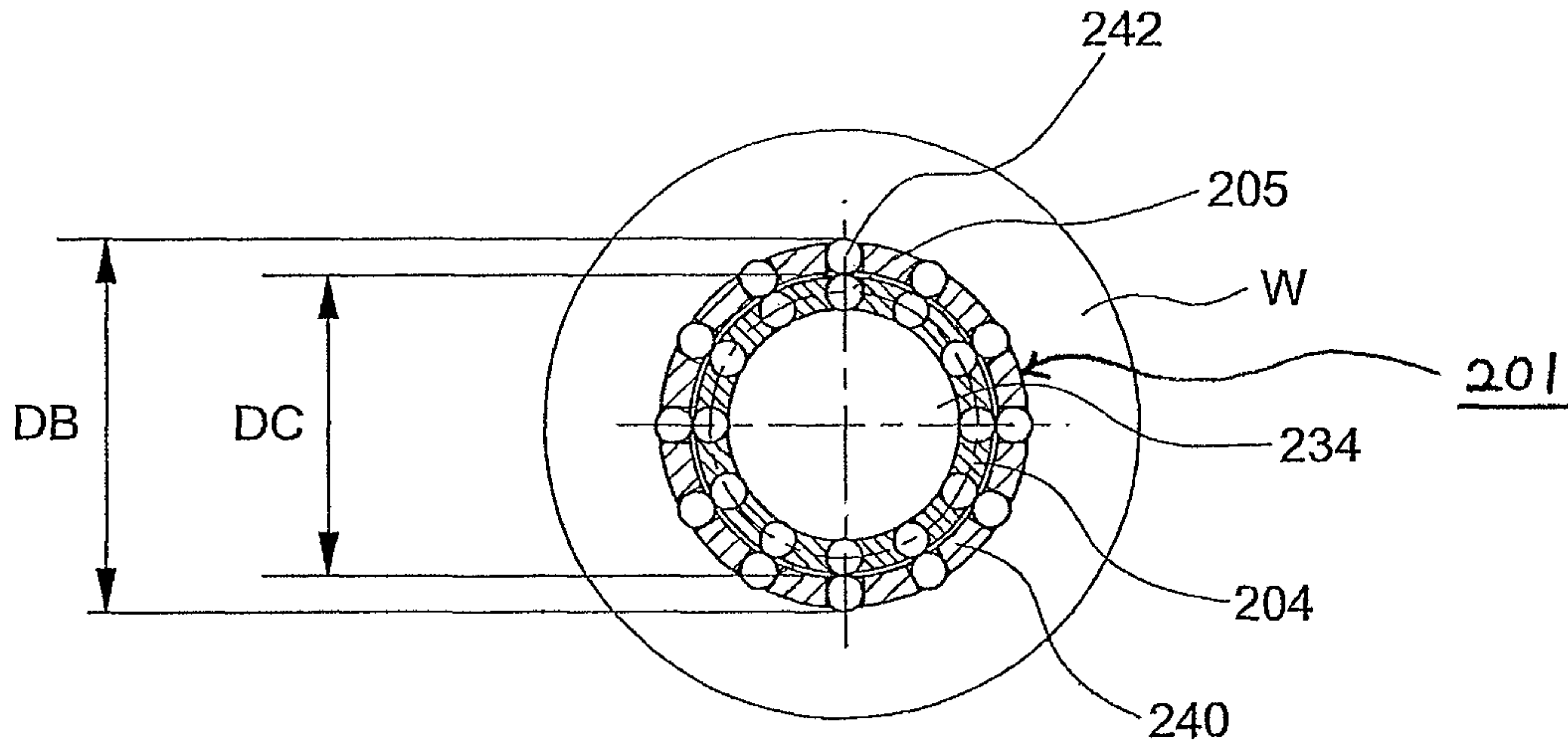
SECTION ALONG LINE D—D
