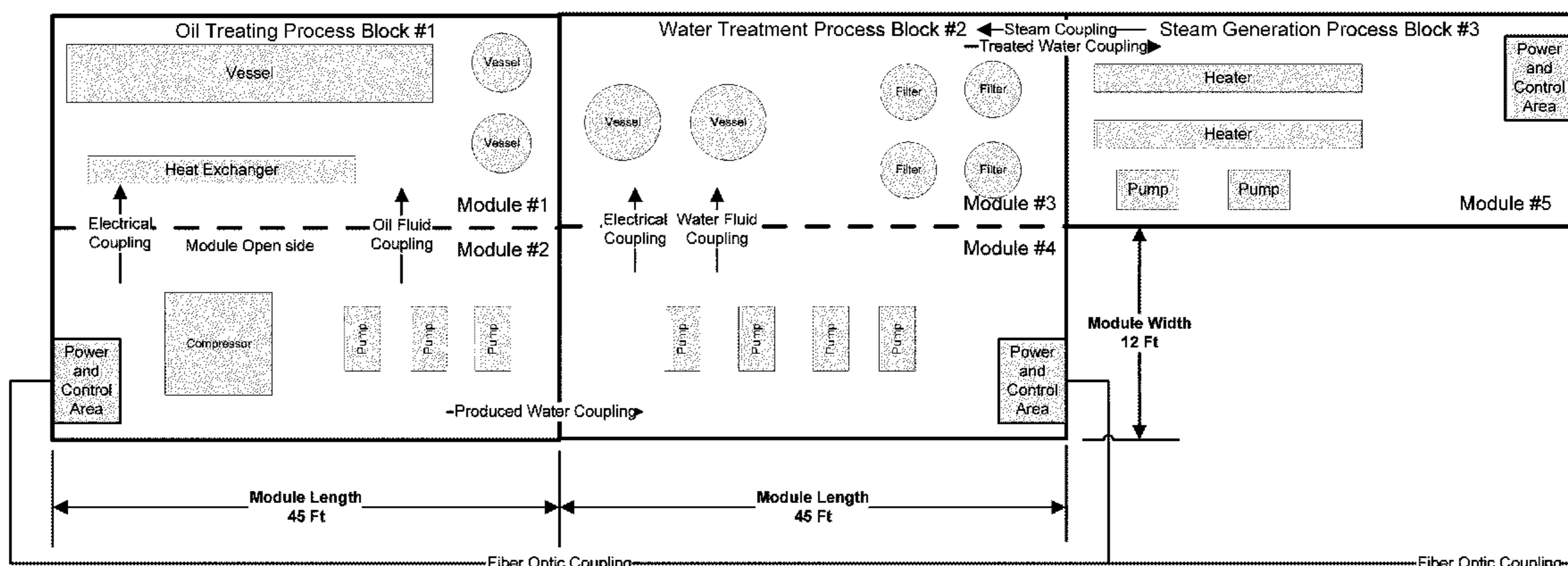
Process Block, Module and Equipment Layout Plan View
