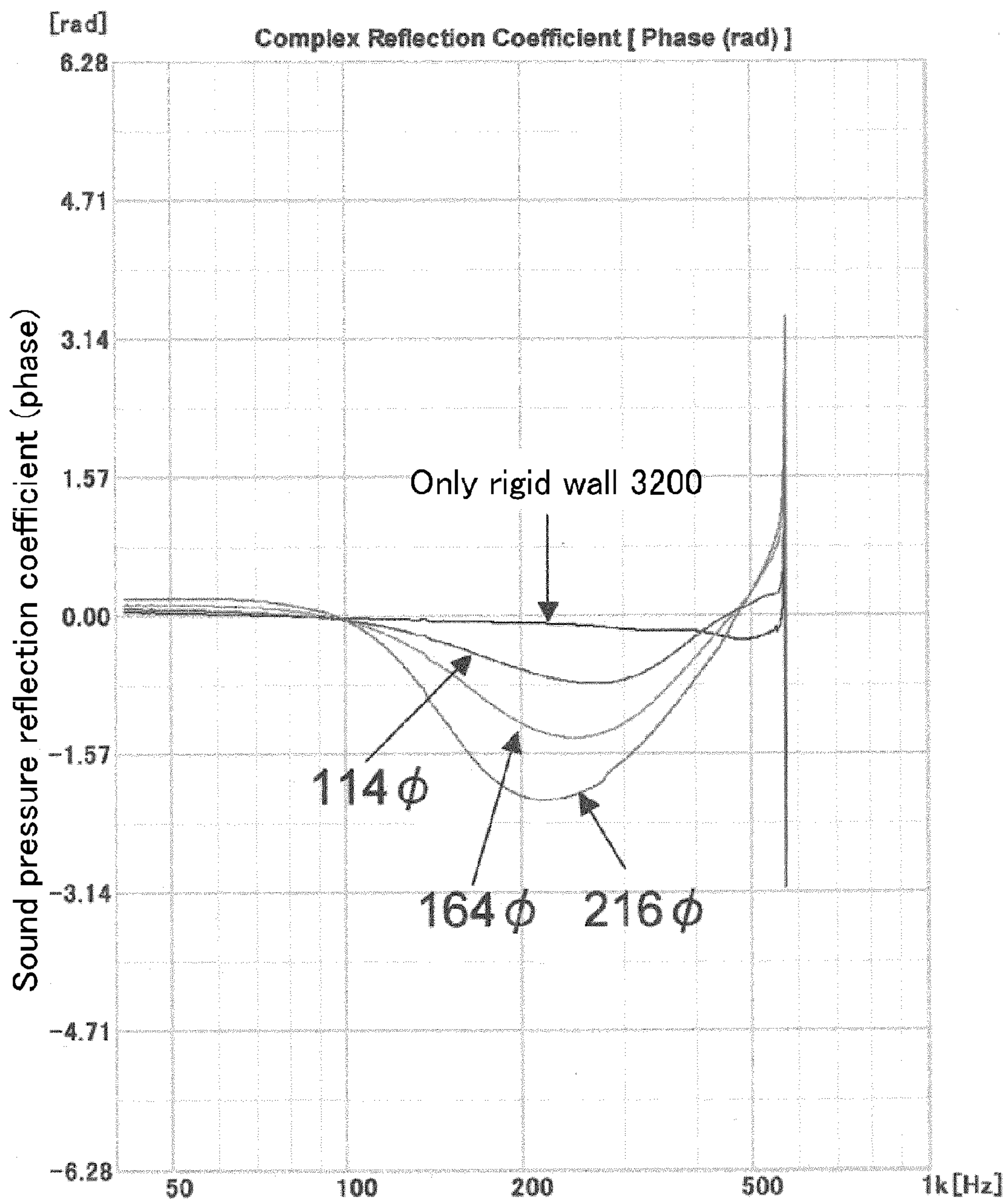
Acoustic material parameter measurement result
