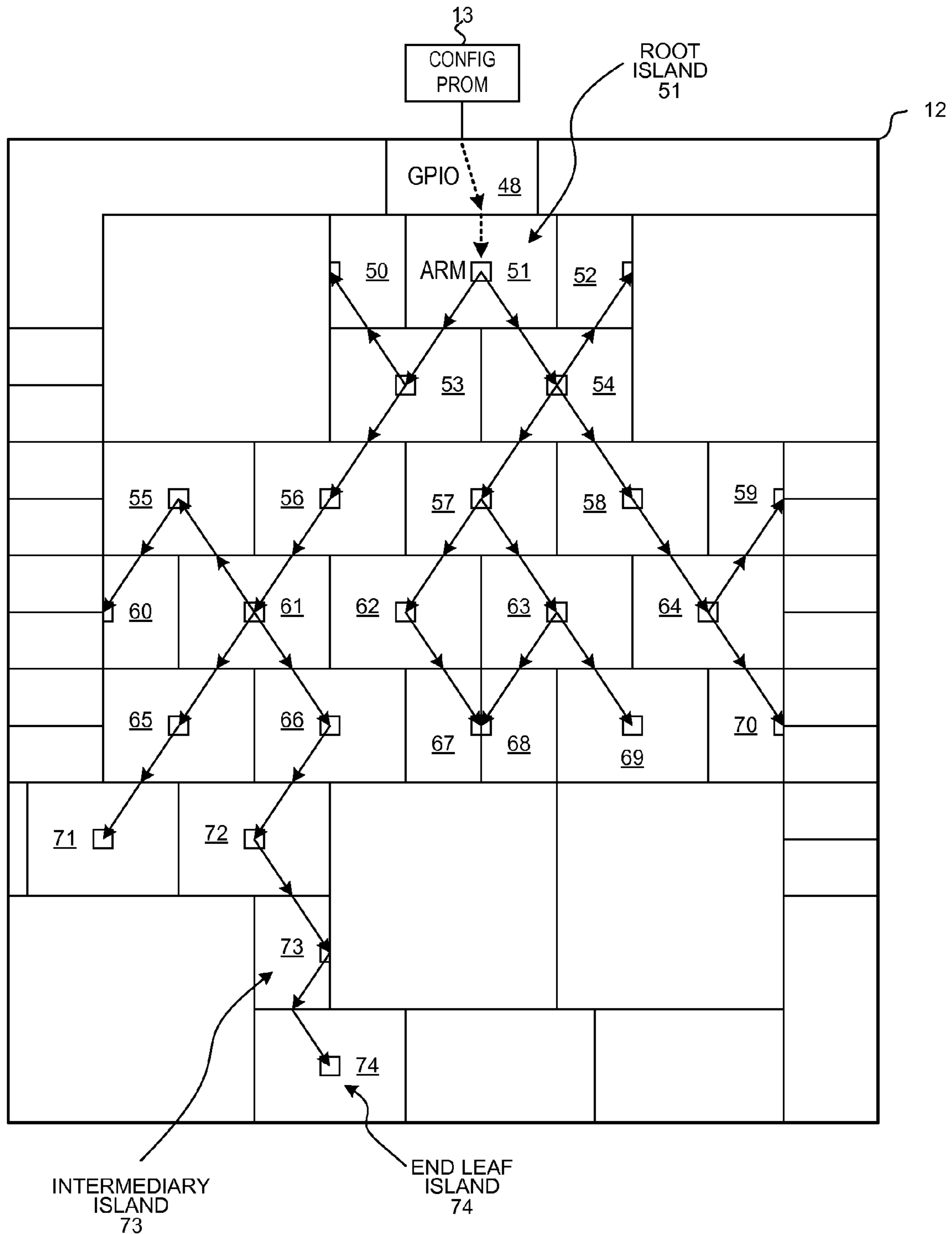
CONFIGURED CONFIGURABLE MESH CONTROL BUS
