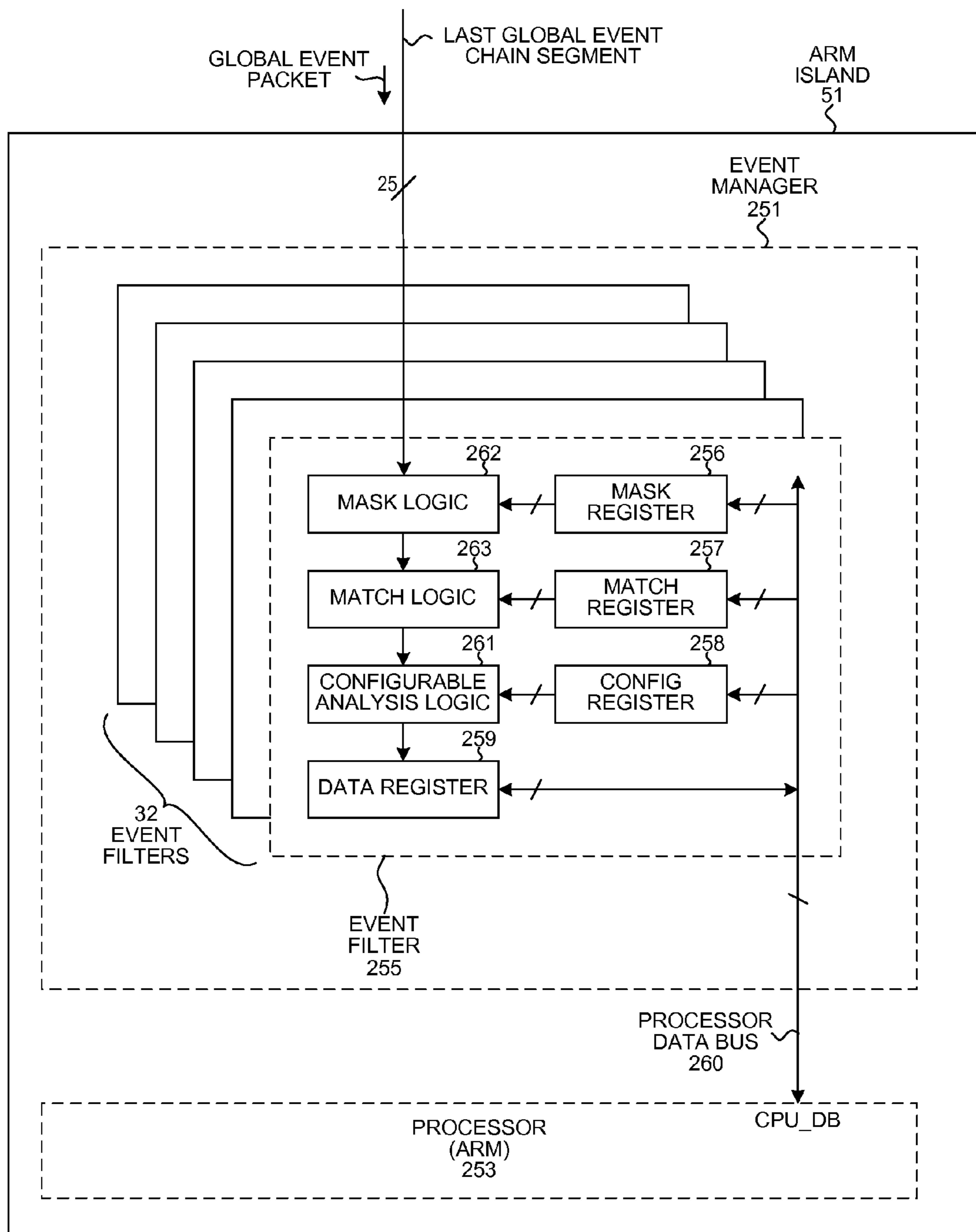
EVENT MANAGER FIG. 42
