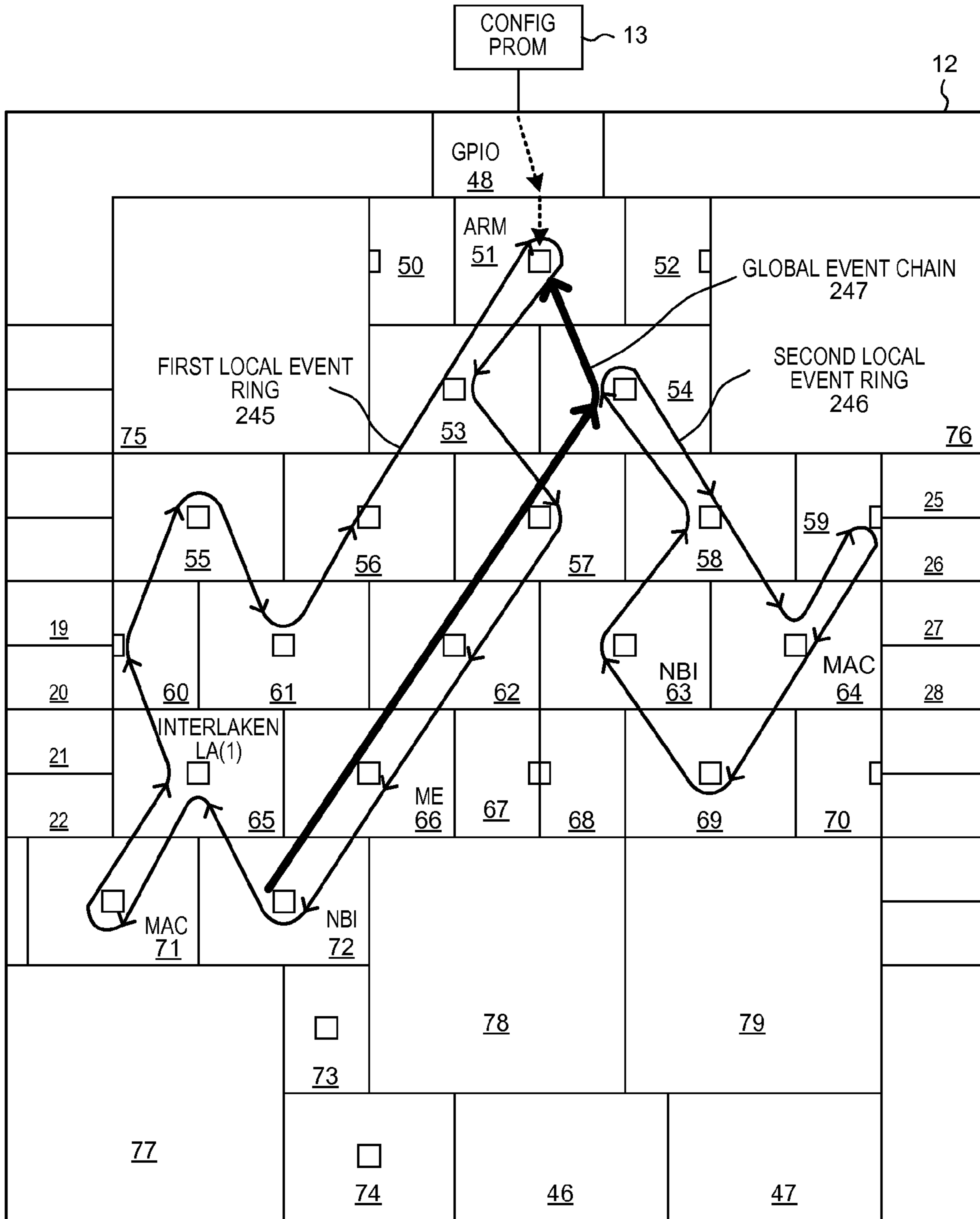
CONFIGURED CONFIGURABLE MESH EVENT BUS
