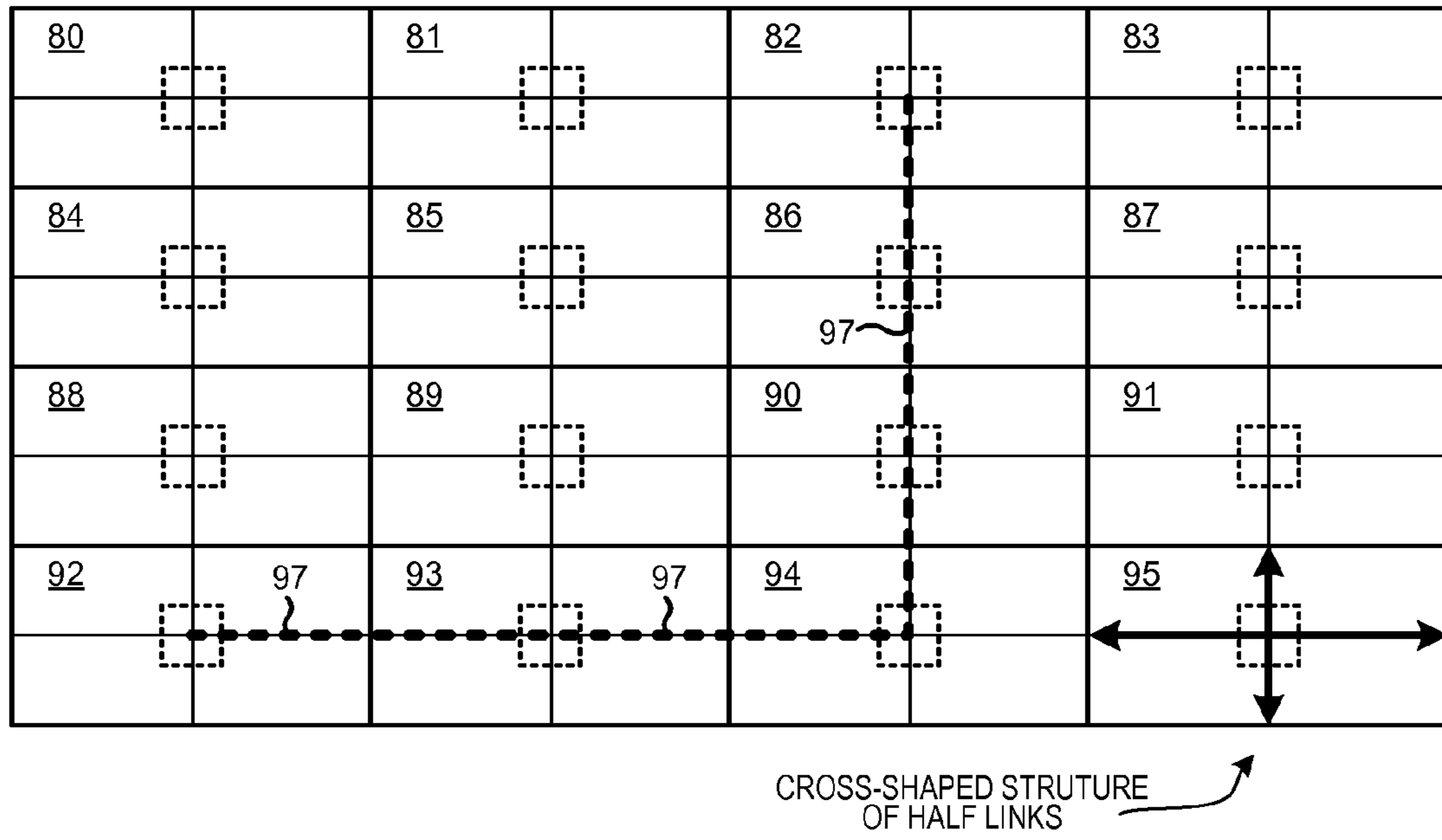
MANHATTAN-PATTERN ISLANDS
