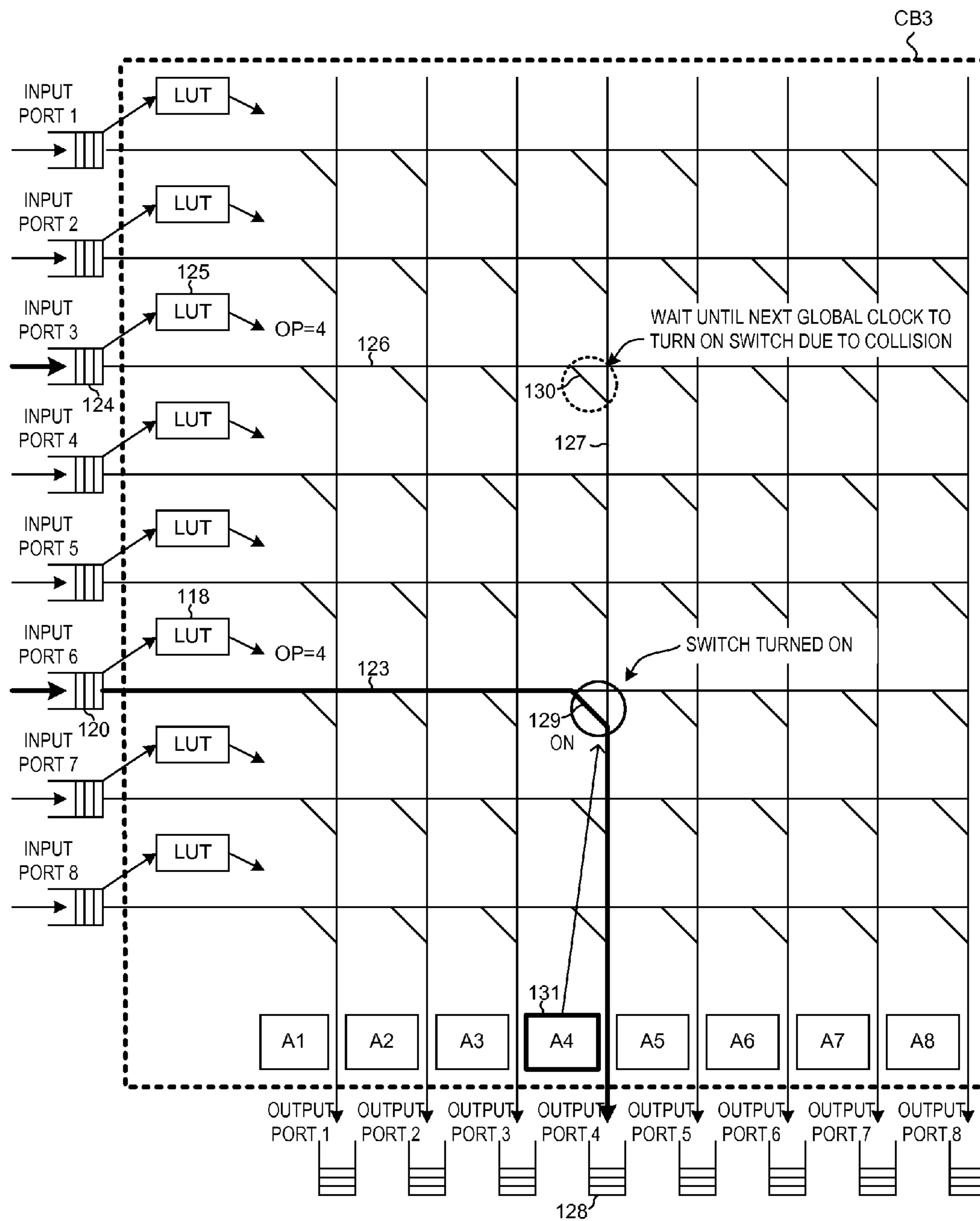
8-WAY CROSSBAR SWITCH FIG. 13
