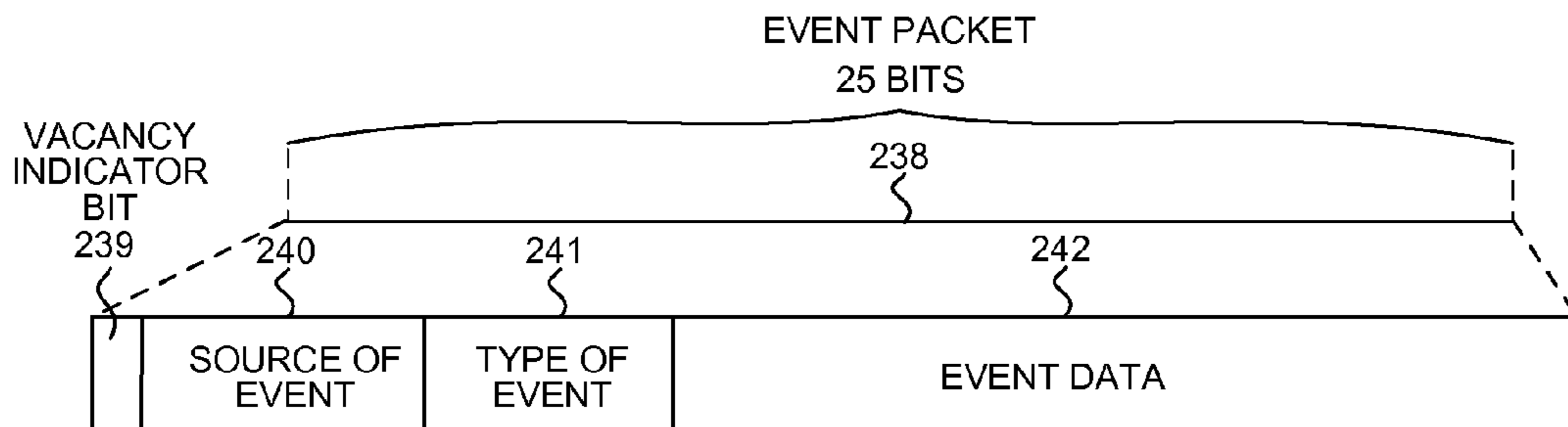
EVENT PACKET BIT SEQUENCE FIG. 38A
