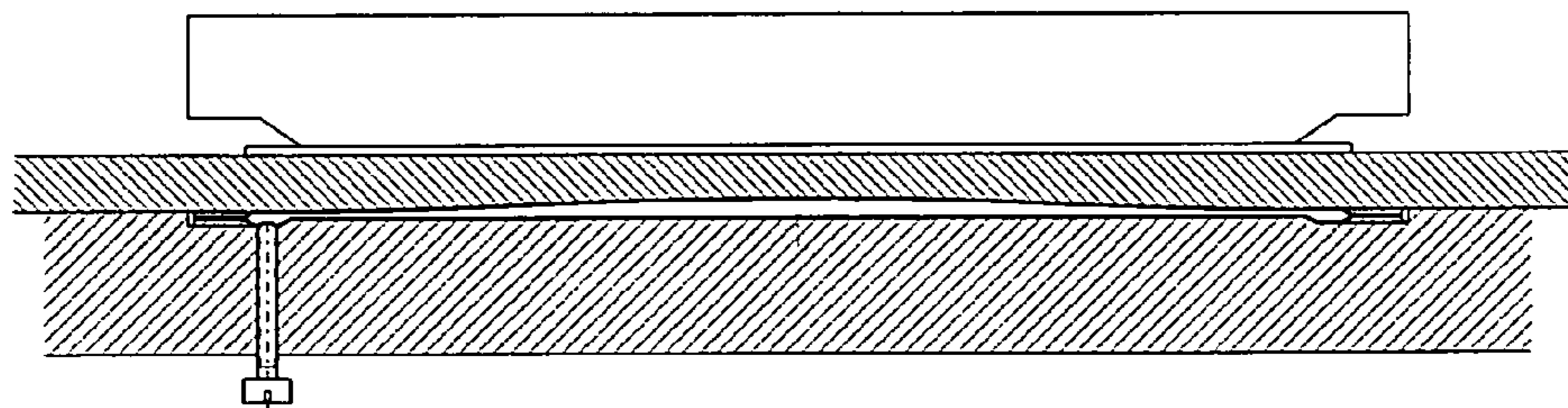
VOLUME & PRESSURE ADJUSTMENT SCREW (70)
