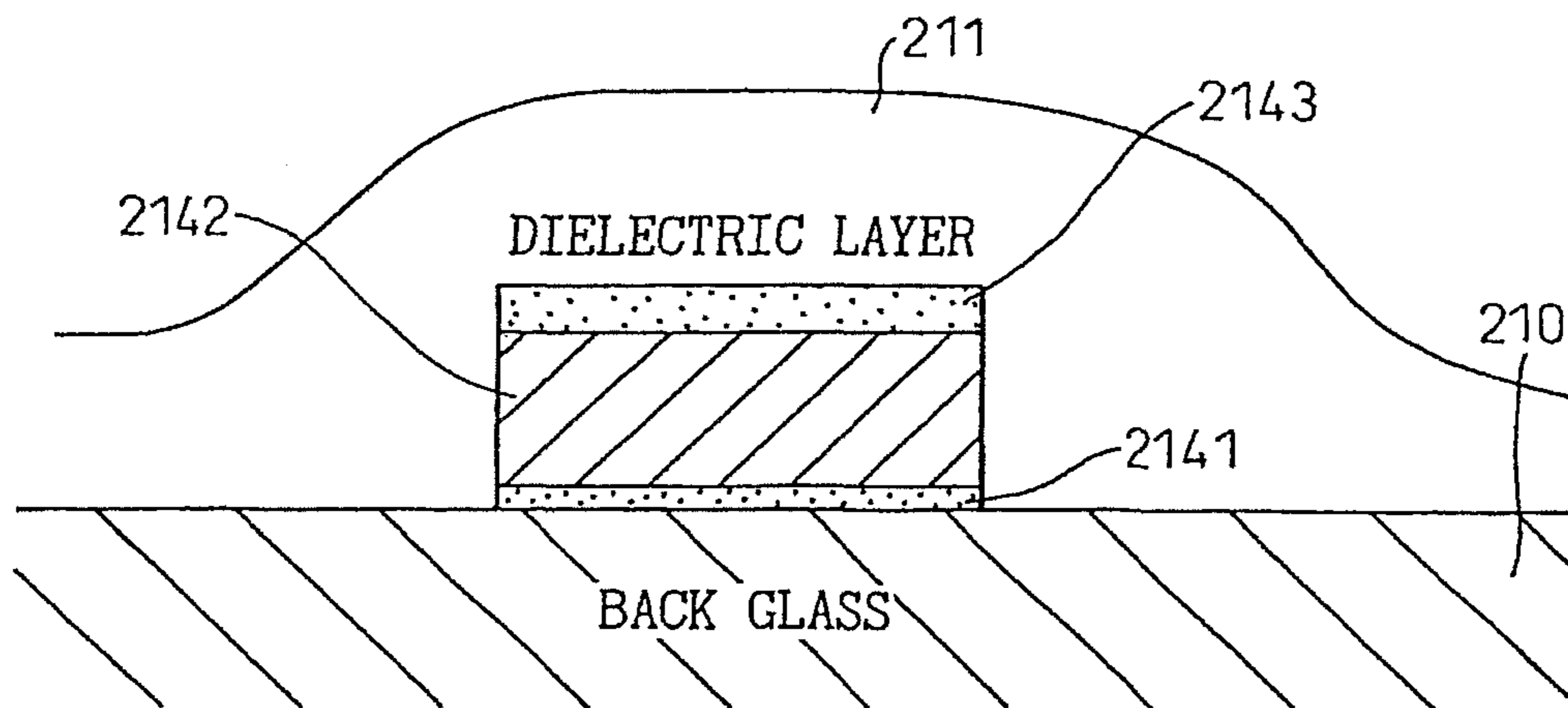
COMPOSITE-MATERIAL ELECTRODE
