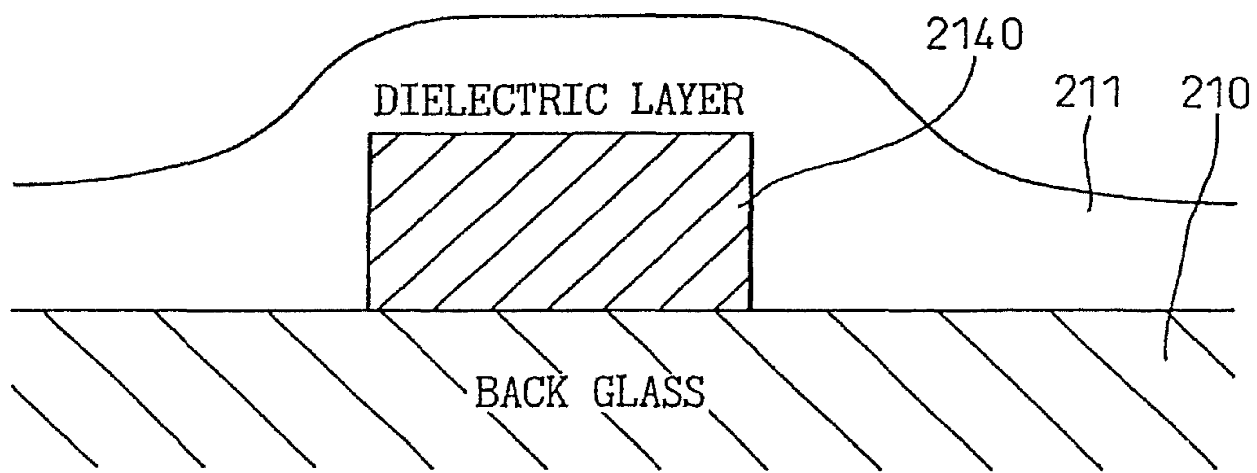
SINGLE-MATERIAL ELECTRODE
