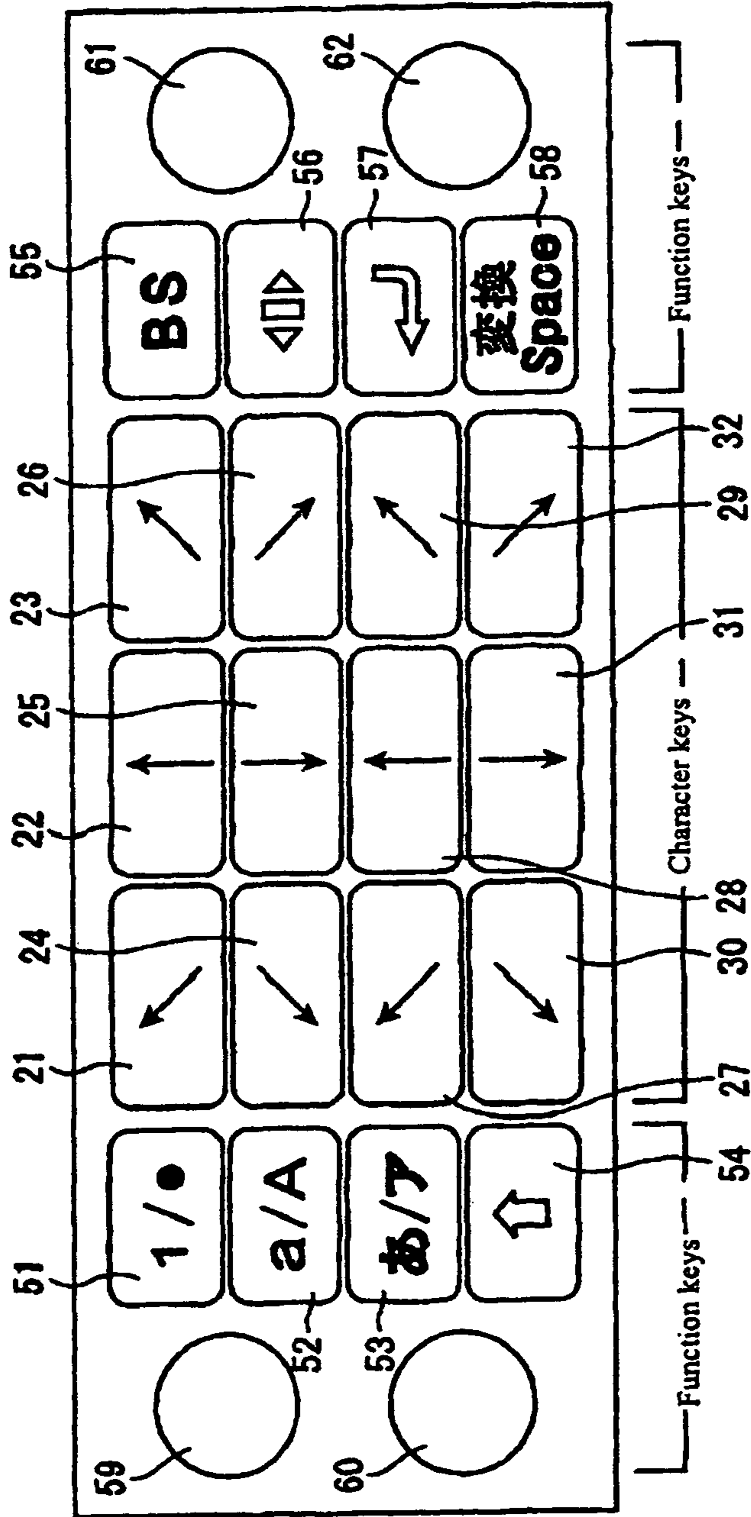
Draw-line touching input used in input portion
