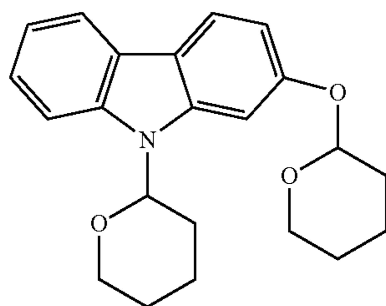
N-tetrahydropyranyl-2- tetrahydropyranyloxy-carbazole
