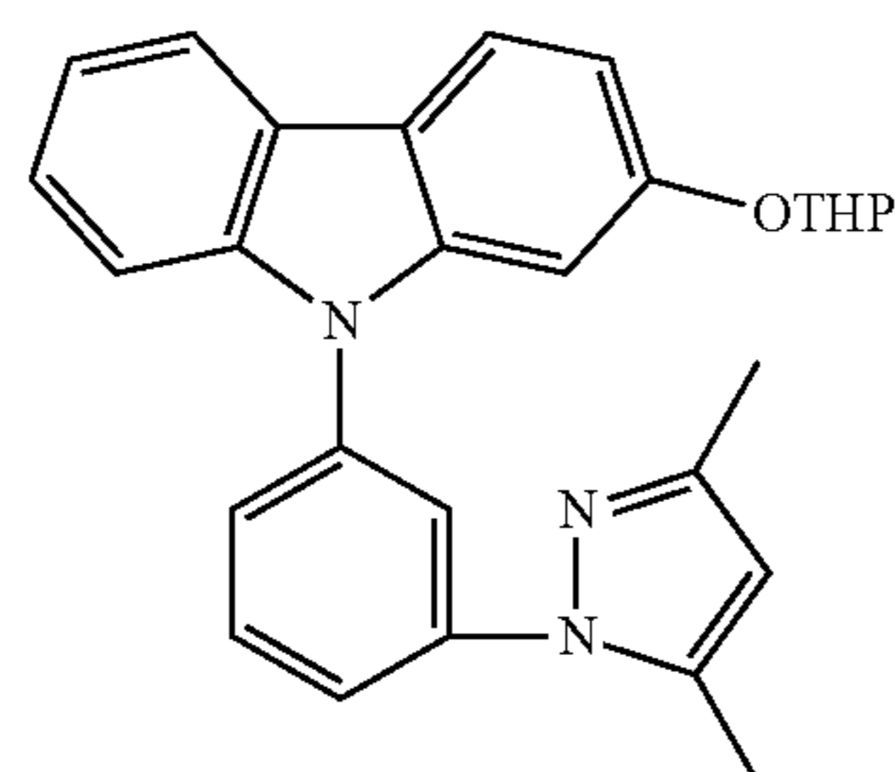
N-[3-(3,5-Dimethylpyrazolyl)phenyl]-2-tetrahydropyranyloxycarbazole
