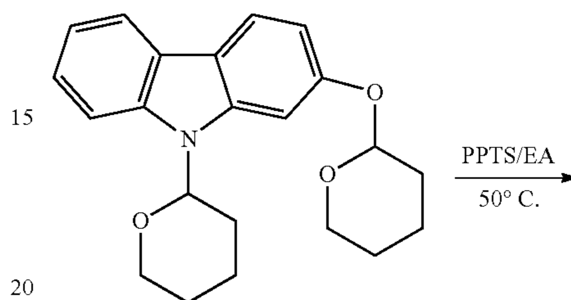
N-tetrahydropyranyl-2-tetrahydropyranyloxy-carbazole
