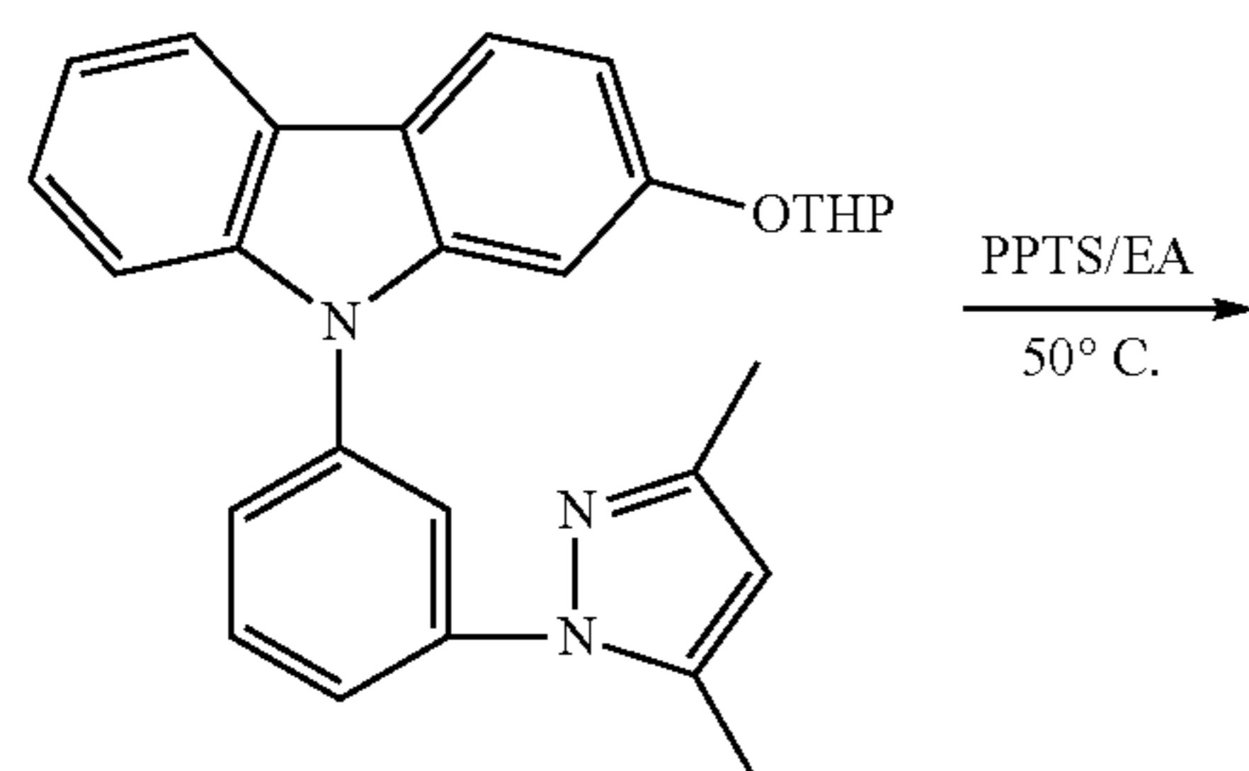
N-[3-(3,5-Dimethylpyrazolyl)phenyl]-2-tetrahydropyranyloxycarbazole
