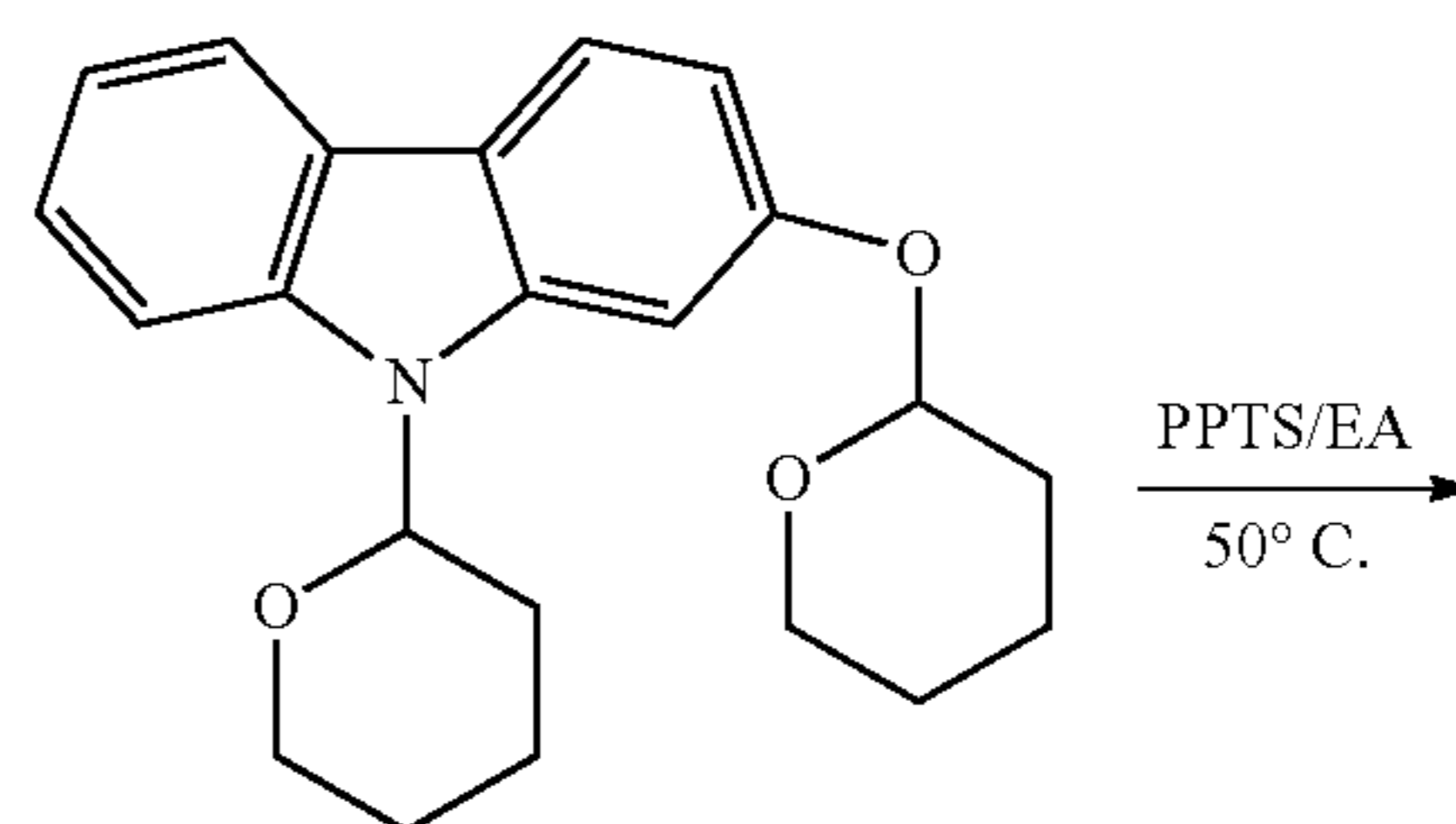
N-tetrahydropyranyl-2- tetrahydropyranyloxy-carbazole
