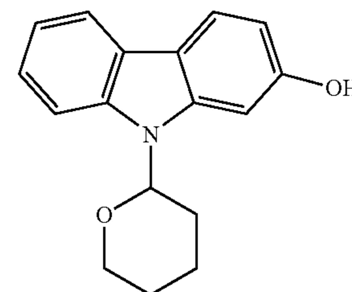
N-tetrahydropyranyl- 2-hydroxycarbazole
