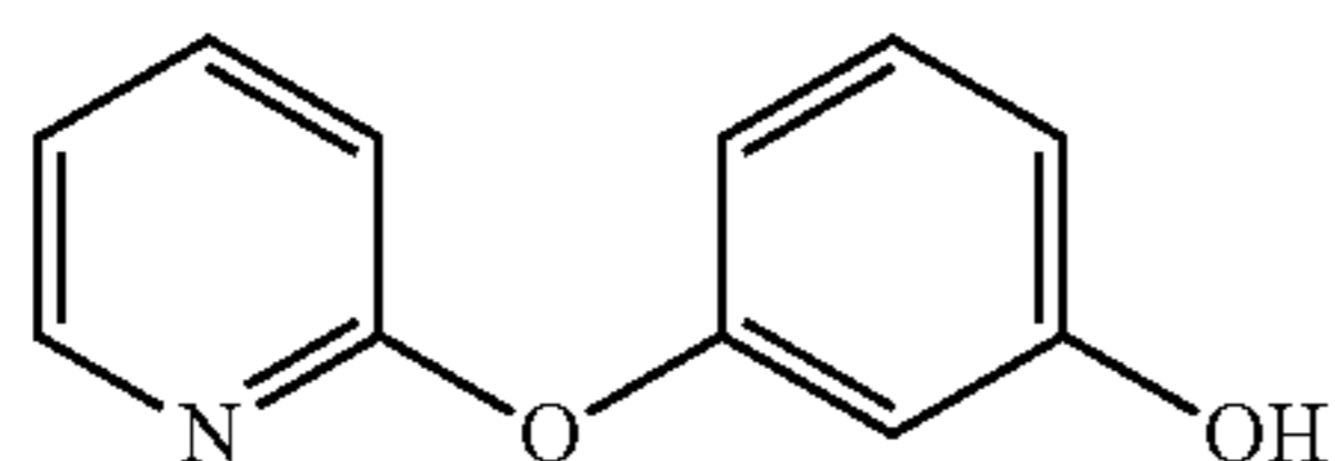
3-(pyridine-2-yloxy)phenol
