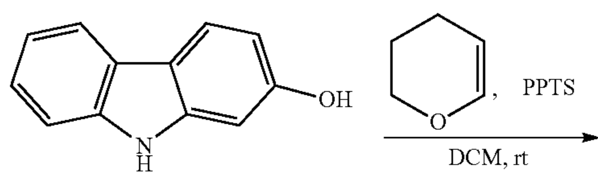
2-hydroxycarbazole
