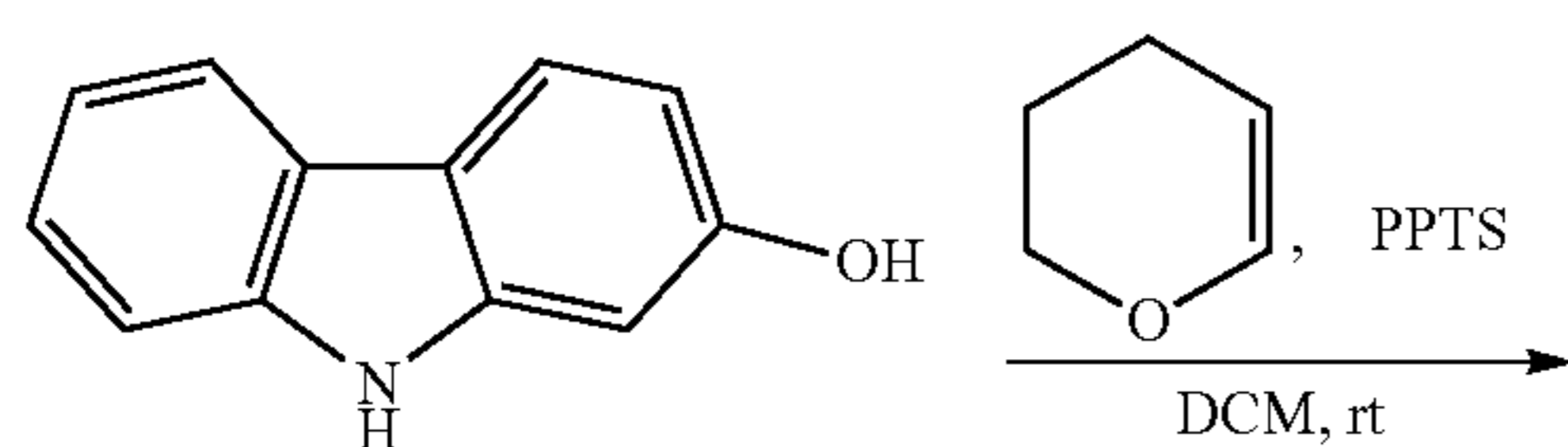
2-hydroxycarbazole
