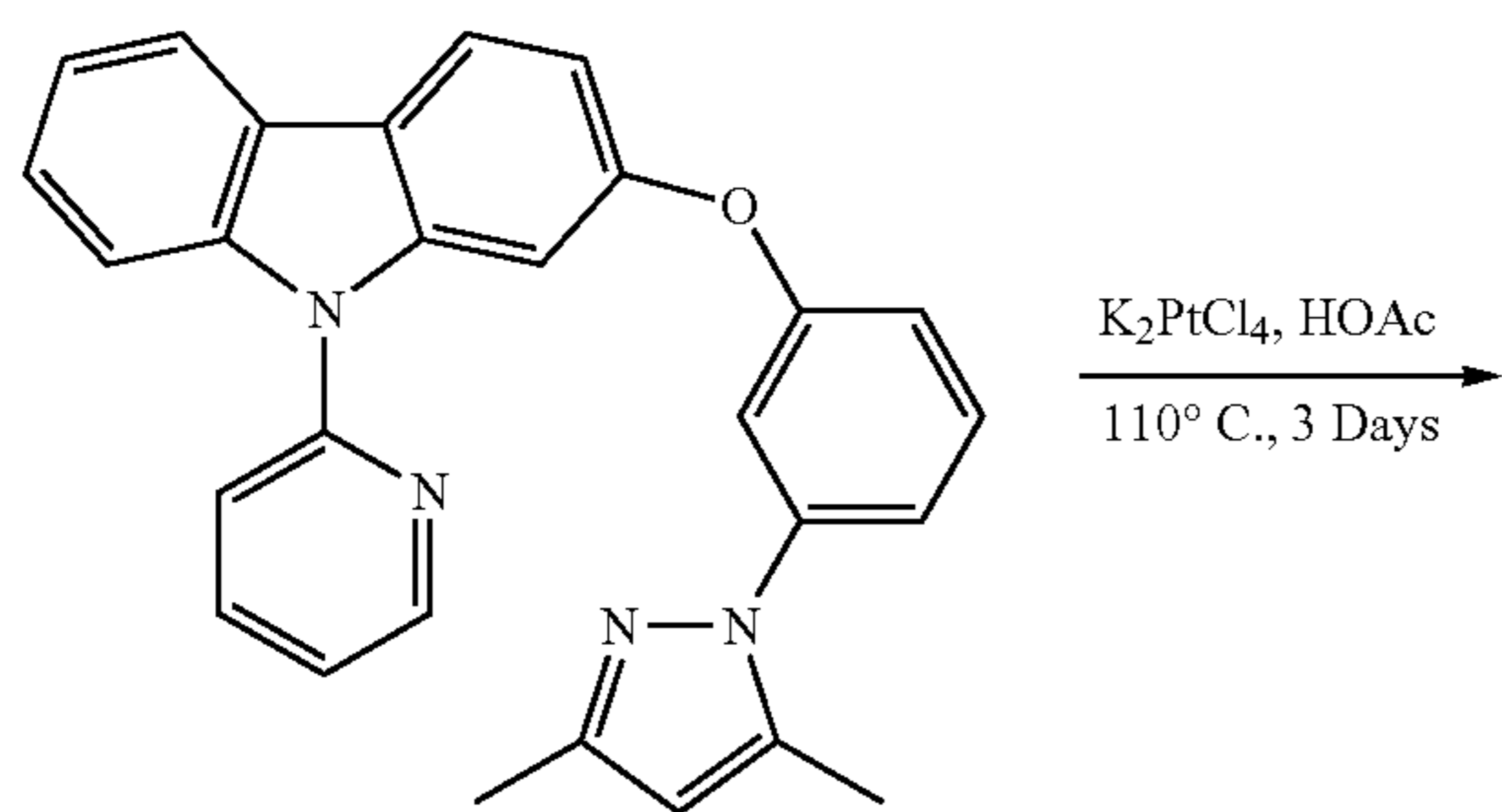
2-[3-(3,5-Dimethylpyrazole-1-yl)-phenoxy]-9-pyridin-2-ylcarbazole
