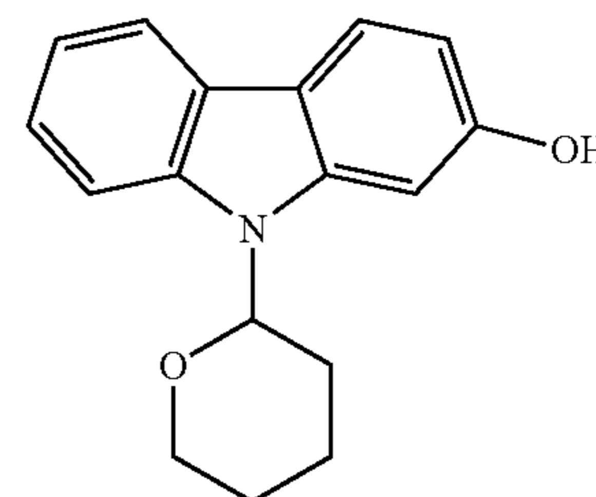
N-tetrahydropyranyl-2-hydroxycarbazole
