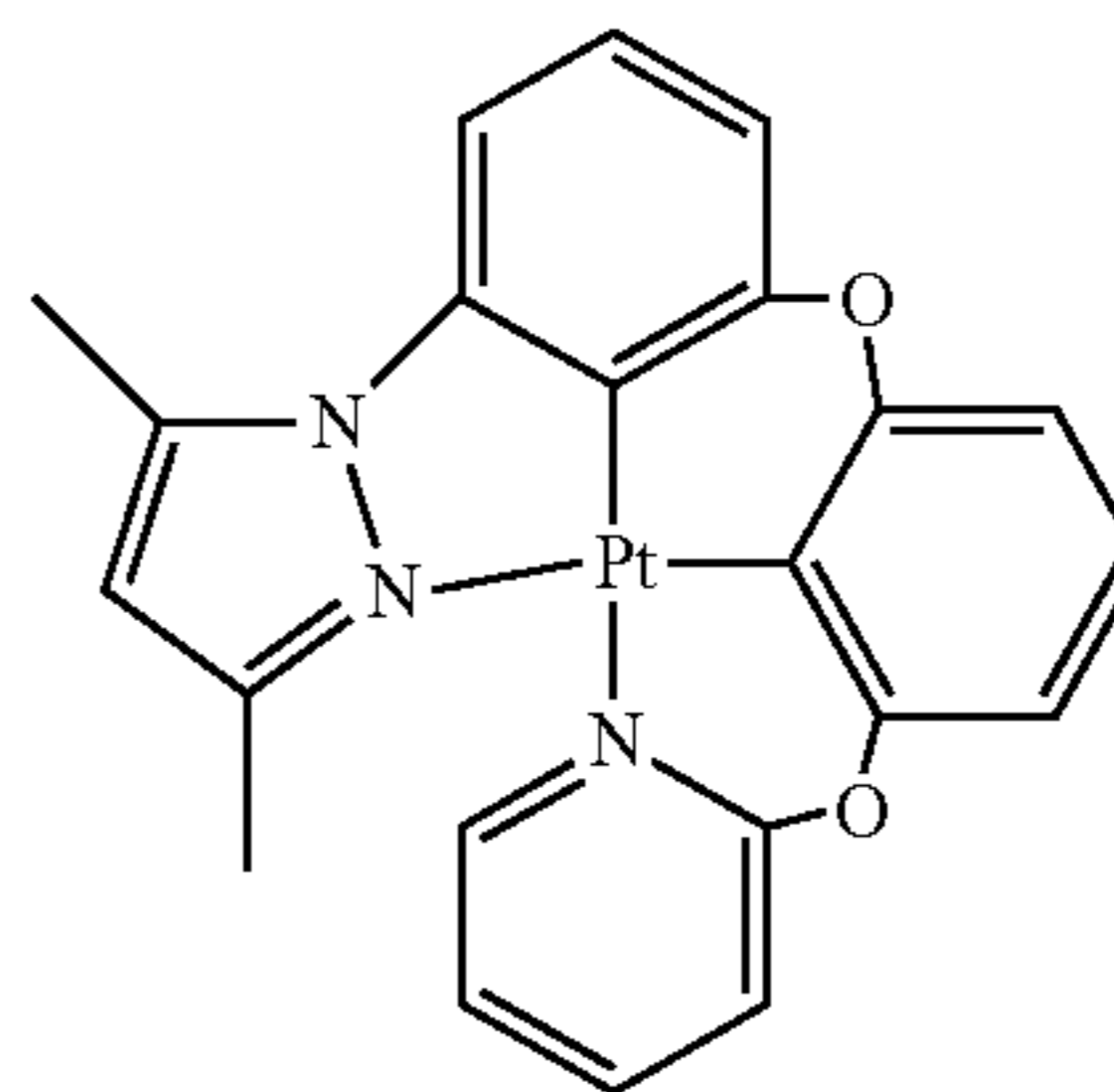
Pt-001 Complex
