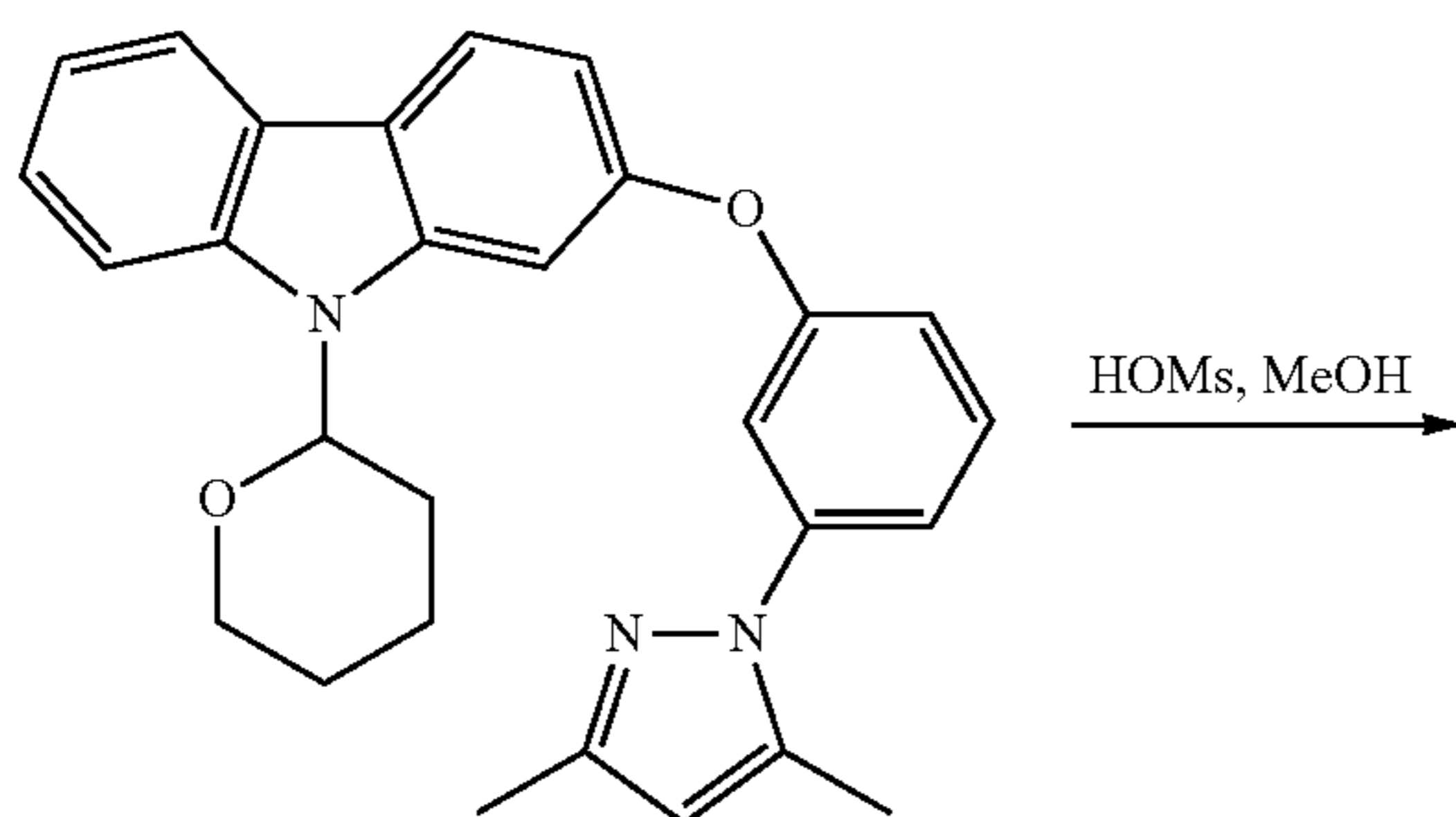
2-[3-(3,5-Dimethylpyrazol-1-yl)-phenoxy]-N-(tetrahydropyranyl)carbazole
