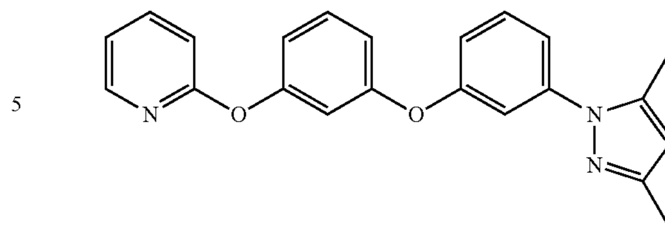
2-(3-(3-(3,5-dimethyl-1H-pyrazol-1-yl)phenoxy)phenoxy)pyridine
