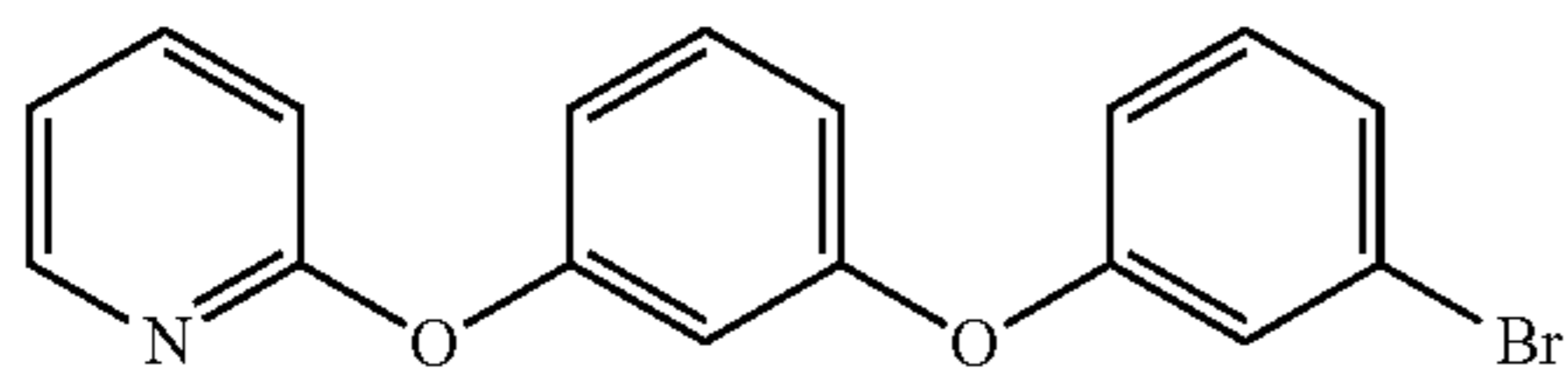
2-(3-(3-bromophenoxy)phenoxy)pyridine
