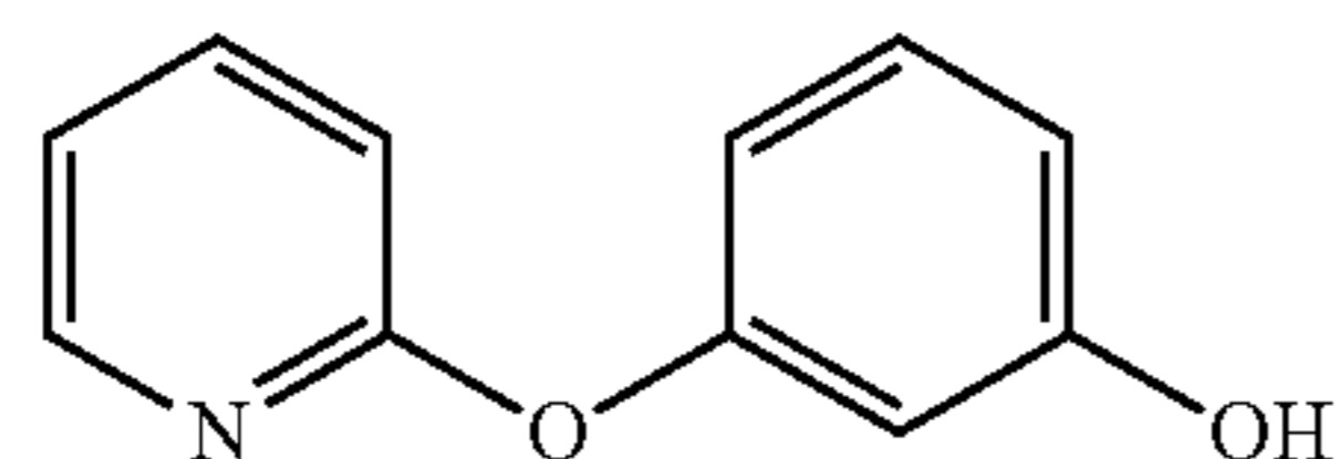
3-(pyridine-2-yloxy)phenol
