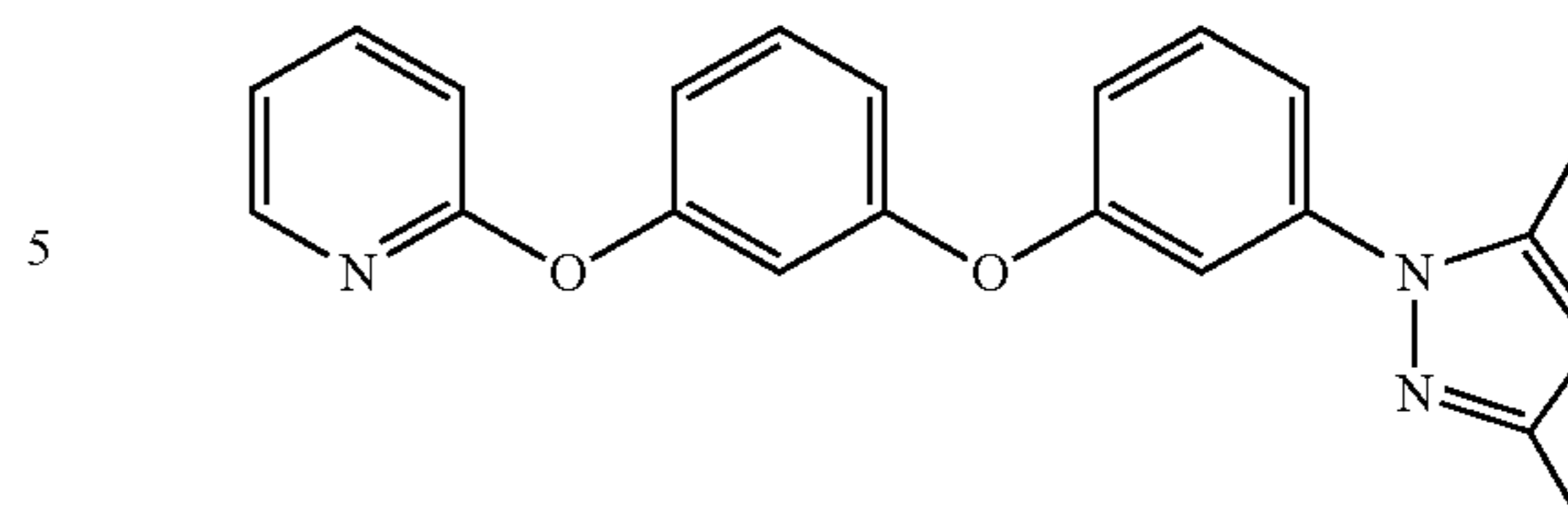
2-(3-(3-(3,5-dimethyl-1H-pyrazol-1-yl)phenoxy)phenoxy)pyridine
