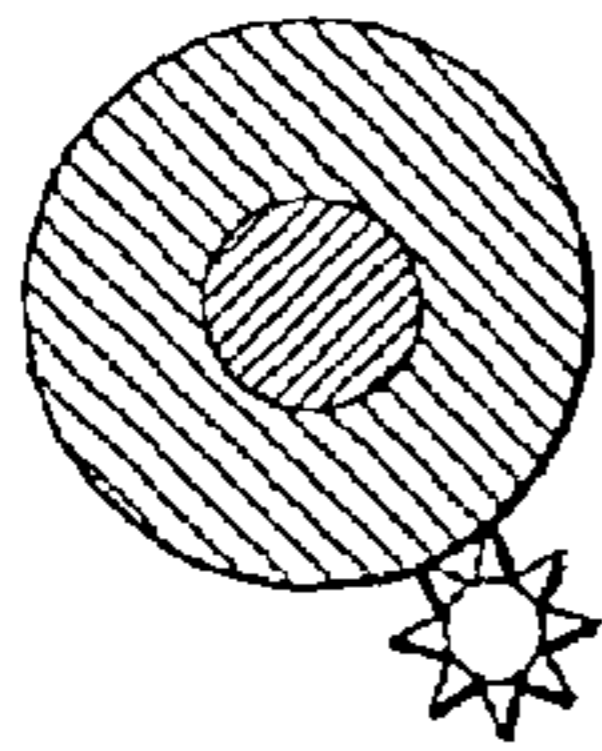
PA MOLECULES BOUND TO METAL NANOPARTICLE
