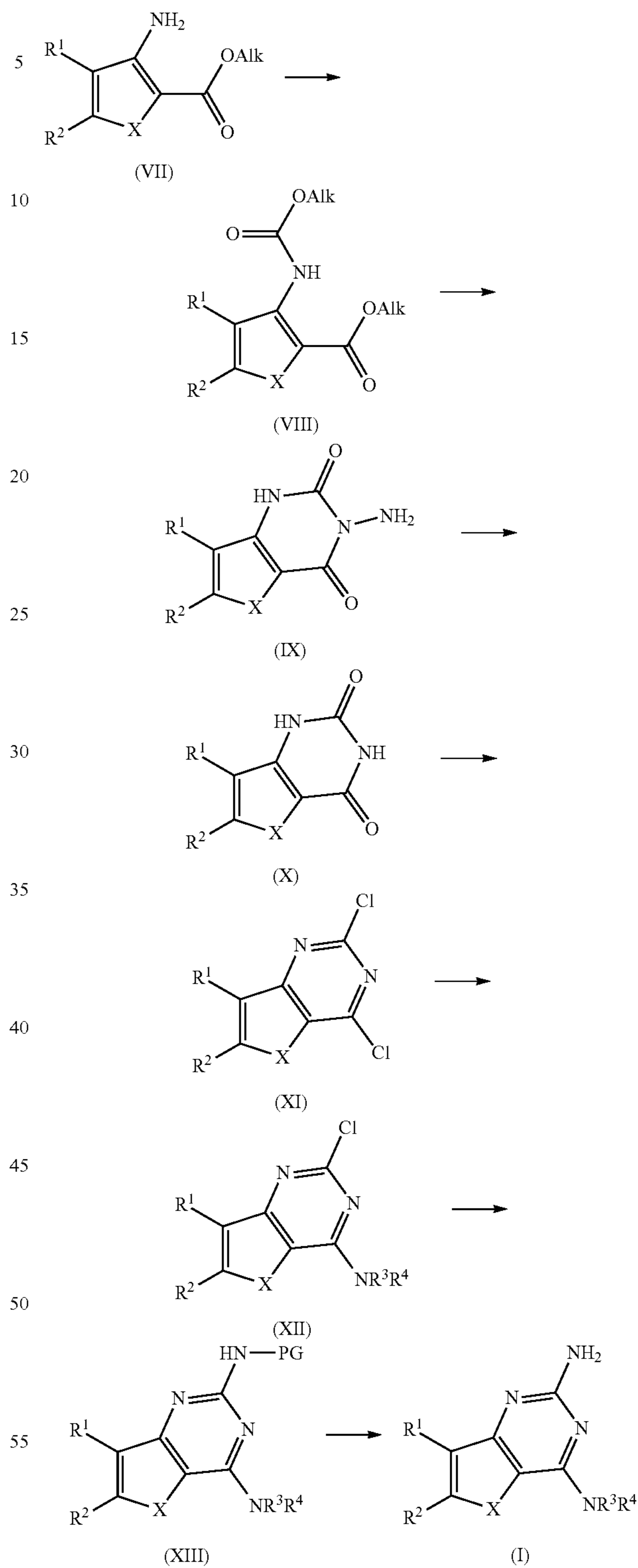
SCHEME A
