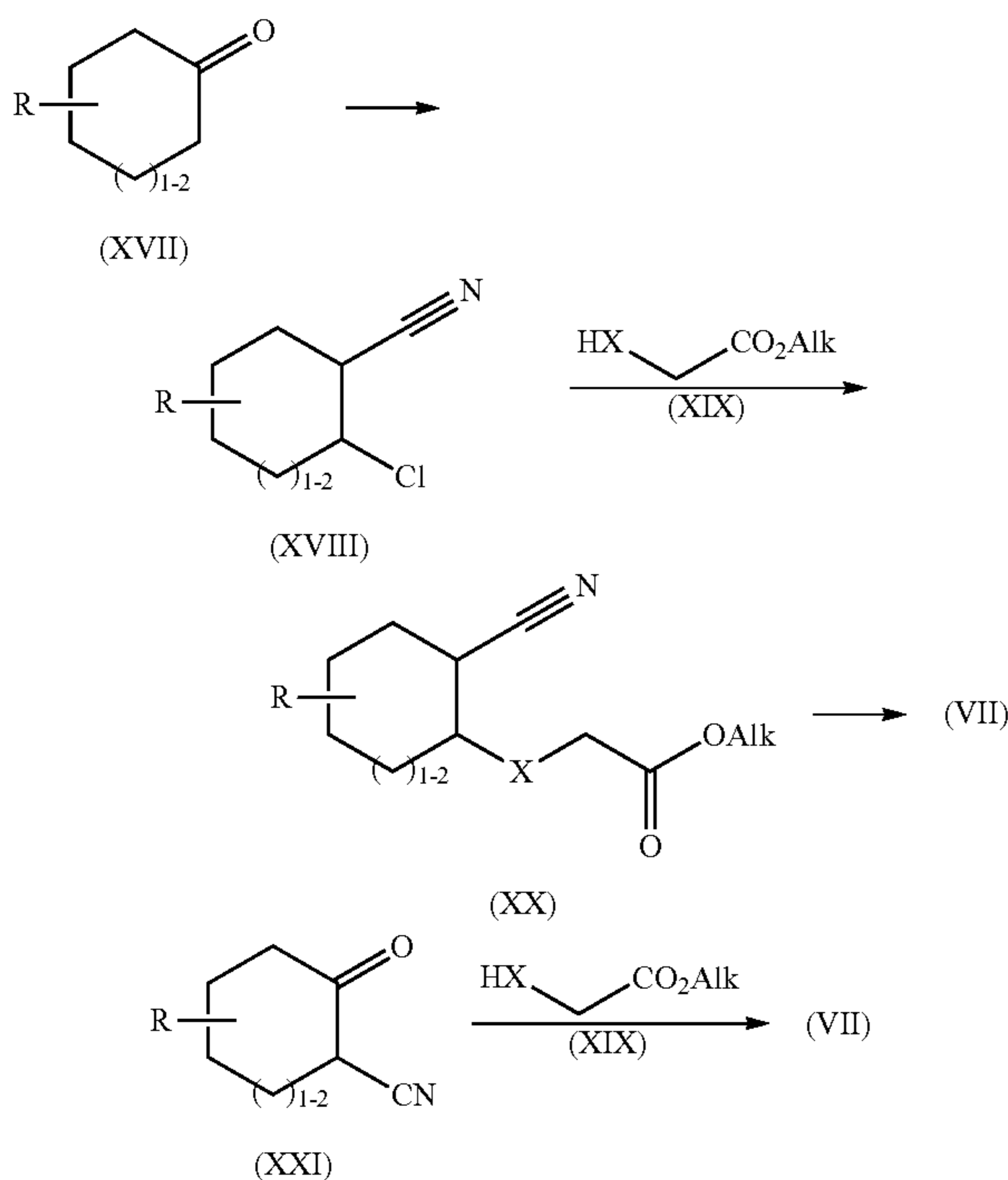
SCHEME C
