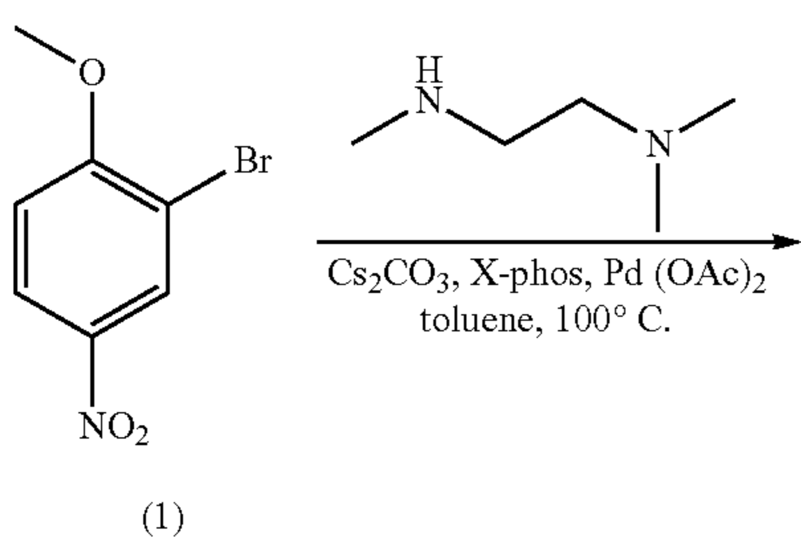
Scheme IV
