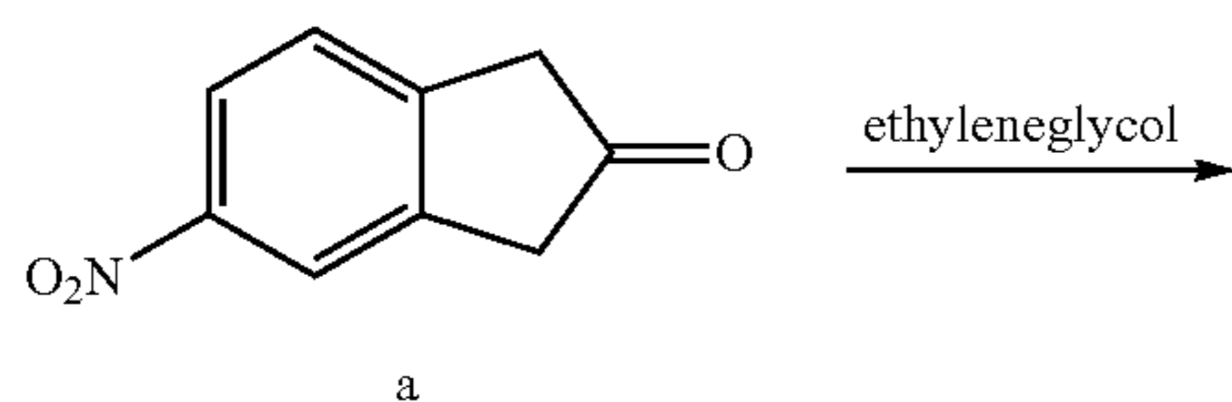
Scheme 3
