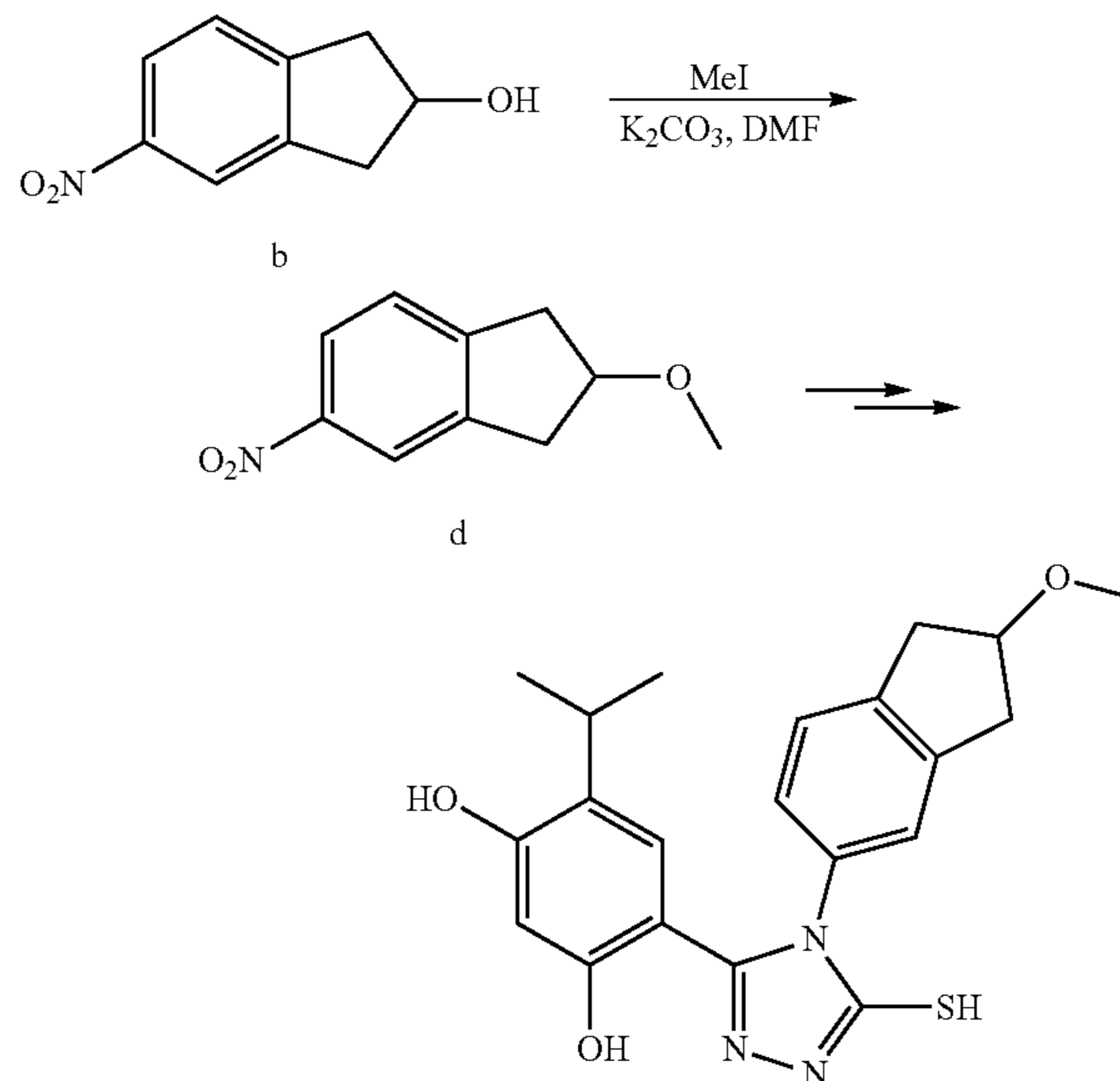
Scheme 2
