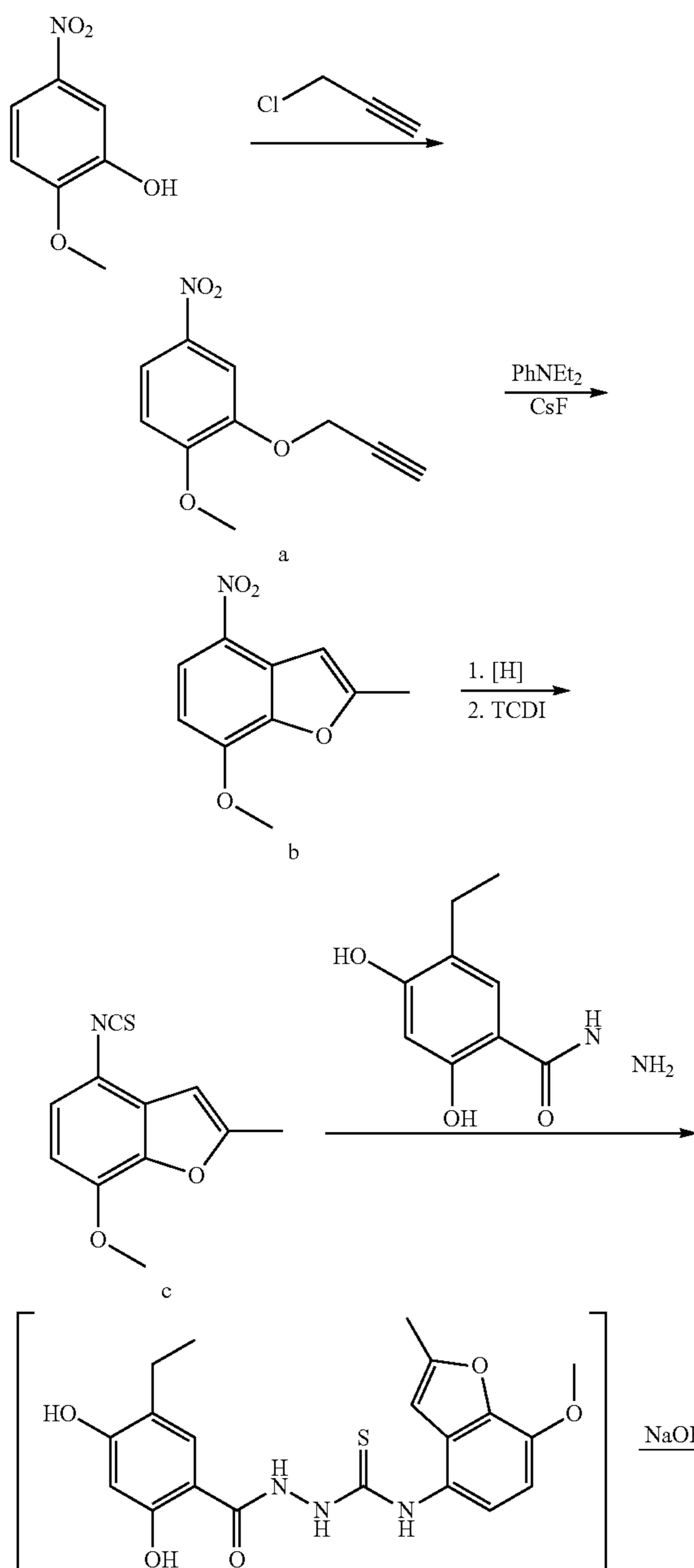
Scheme 7
