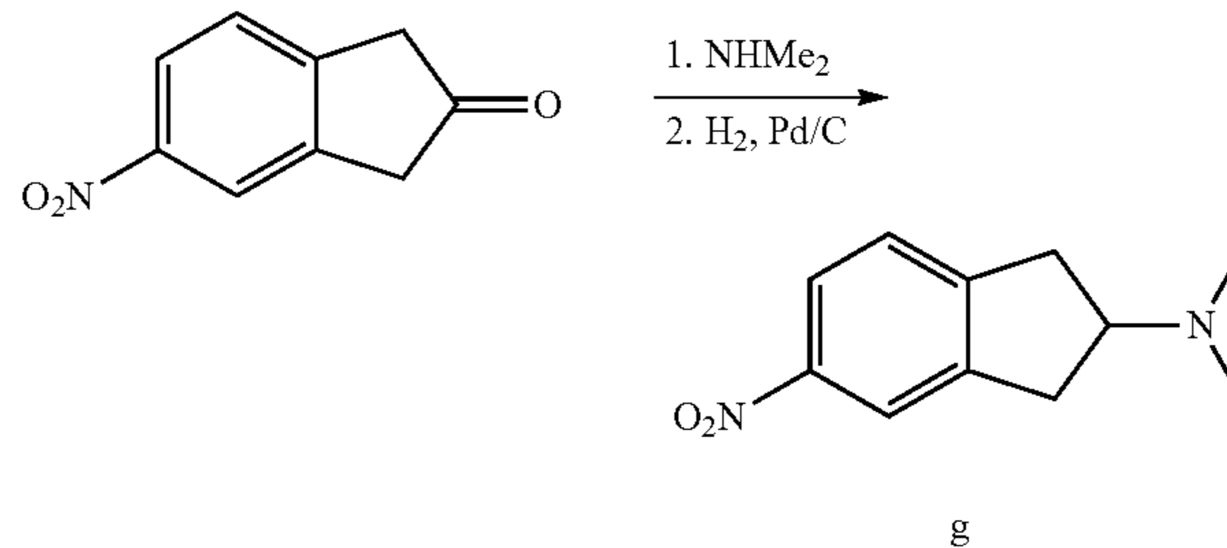
Scheme 6
