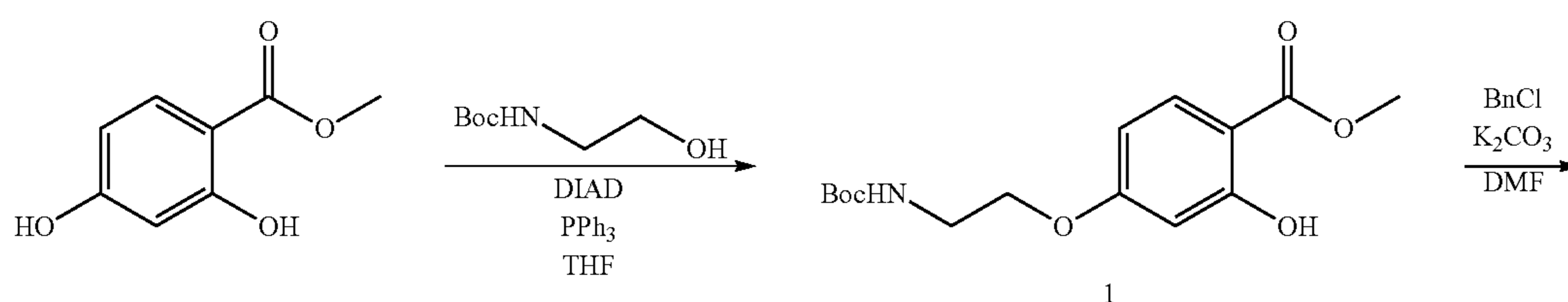
Scheme 8
