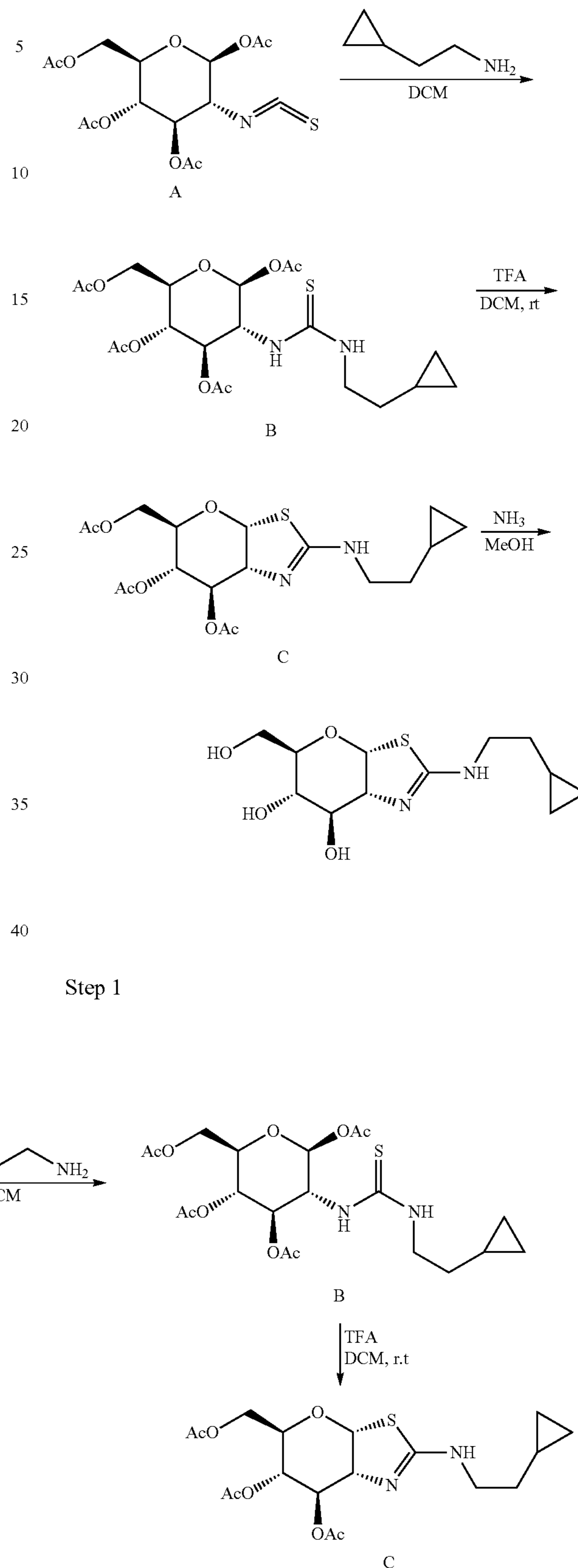
Scheme I
