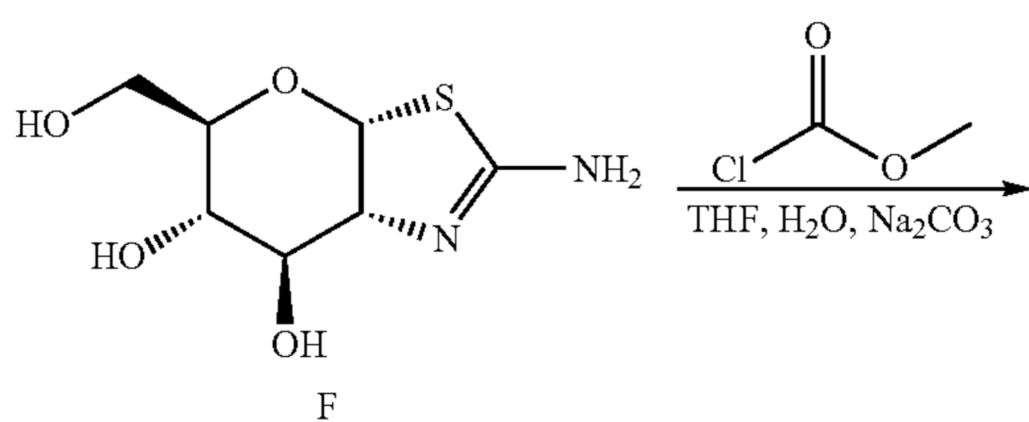
Scheme III
