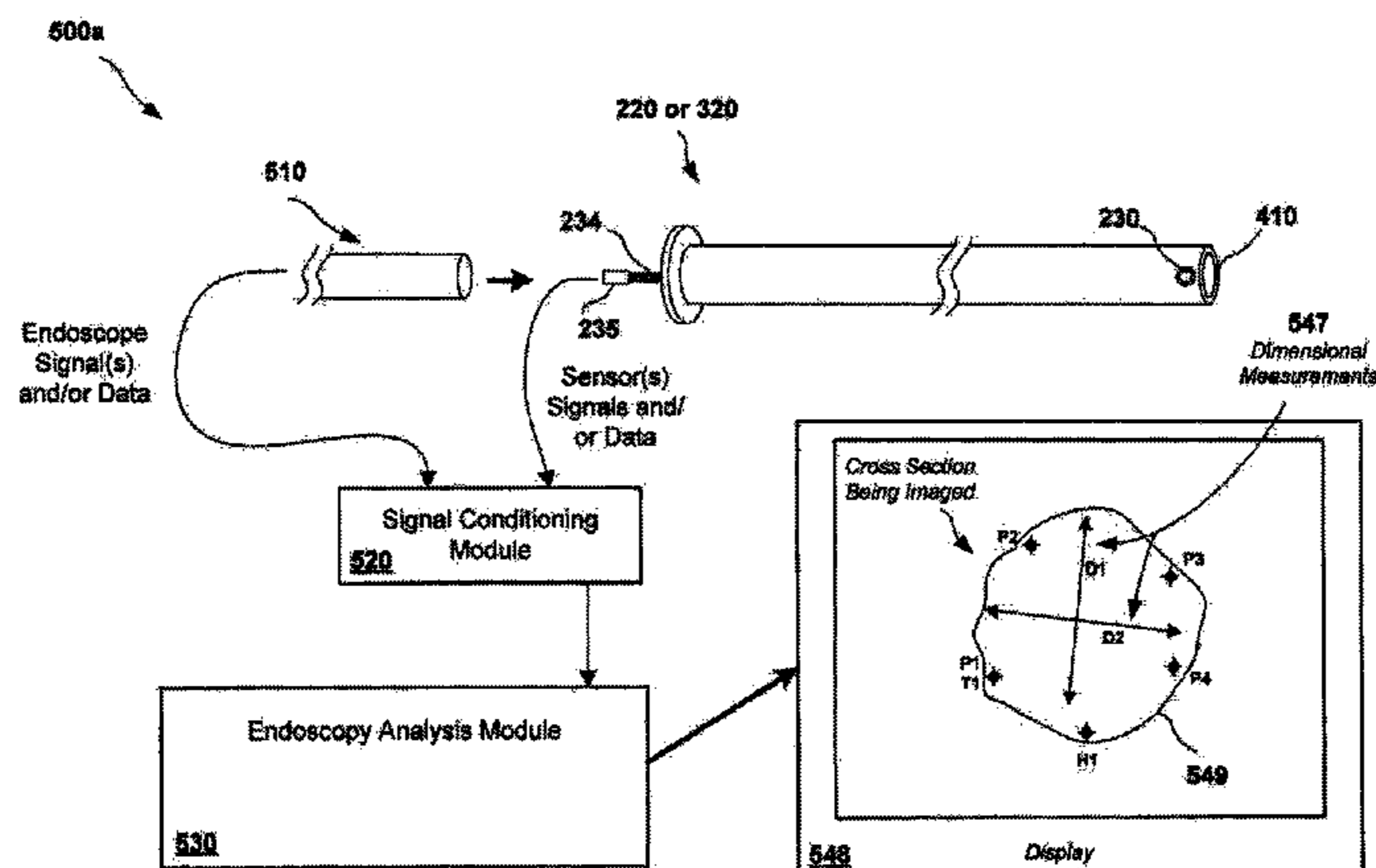
Example Sensor Enhanced Endoscopy System
