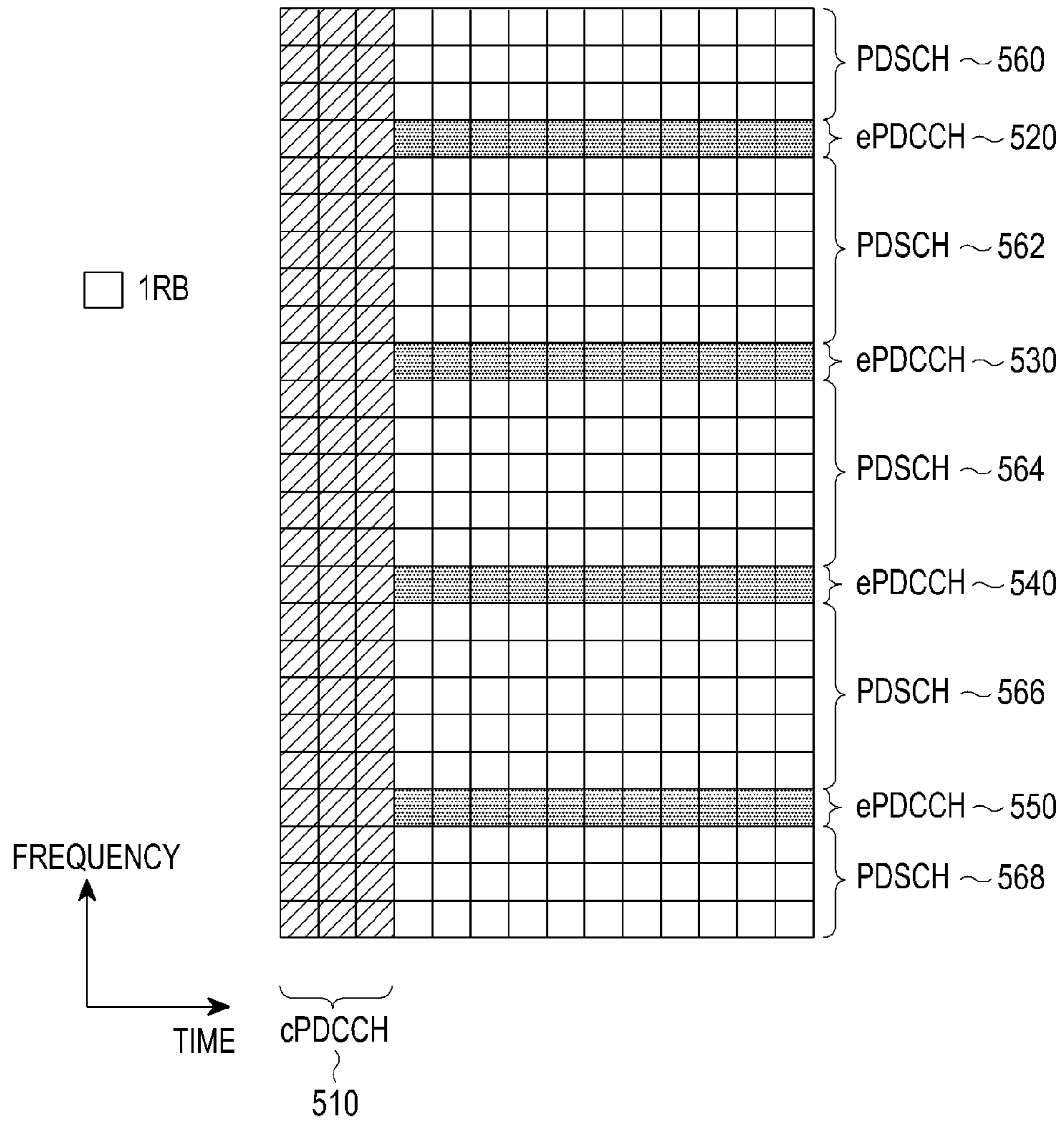
FIG.5 (PRIOR ART)
