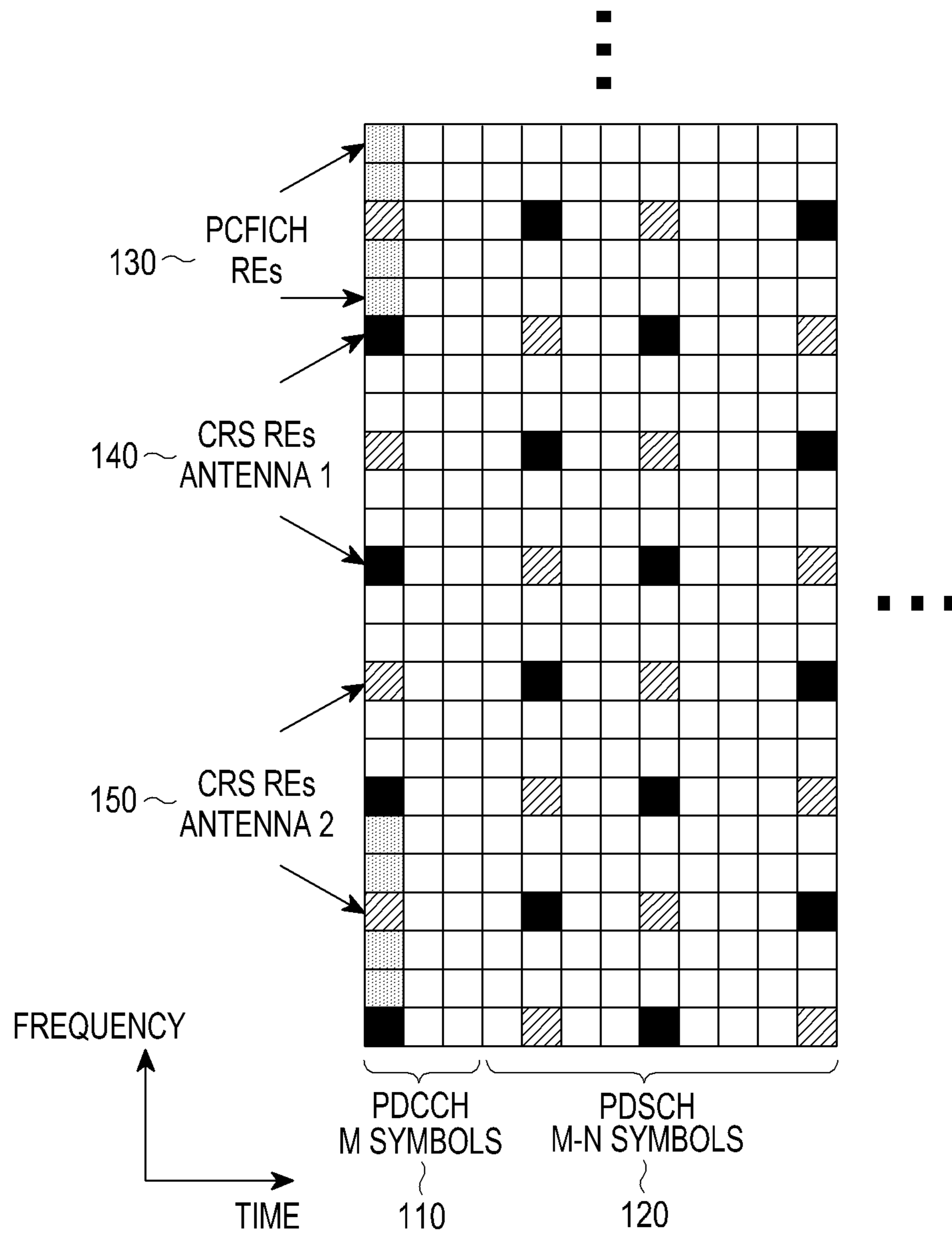
FIG.1 (PRIOR ART)
