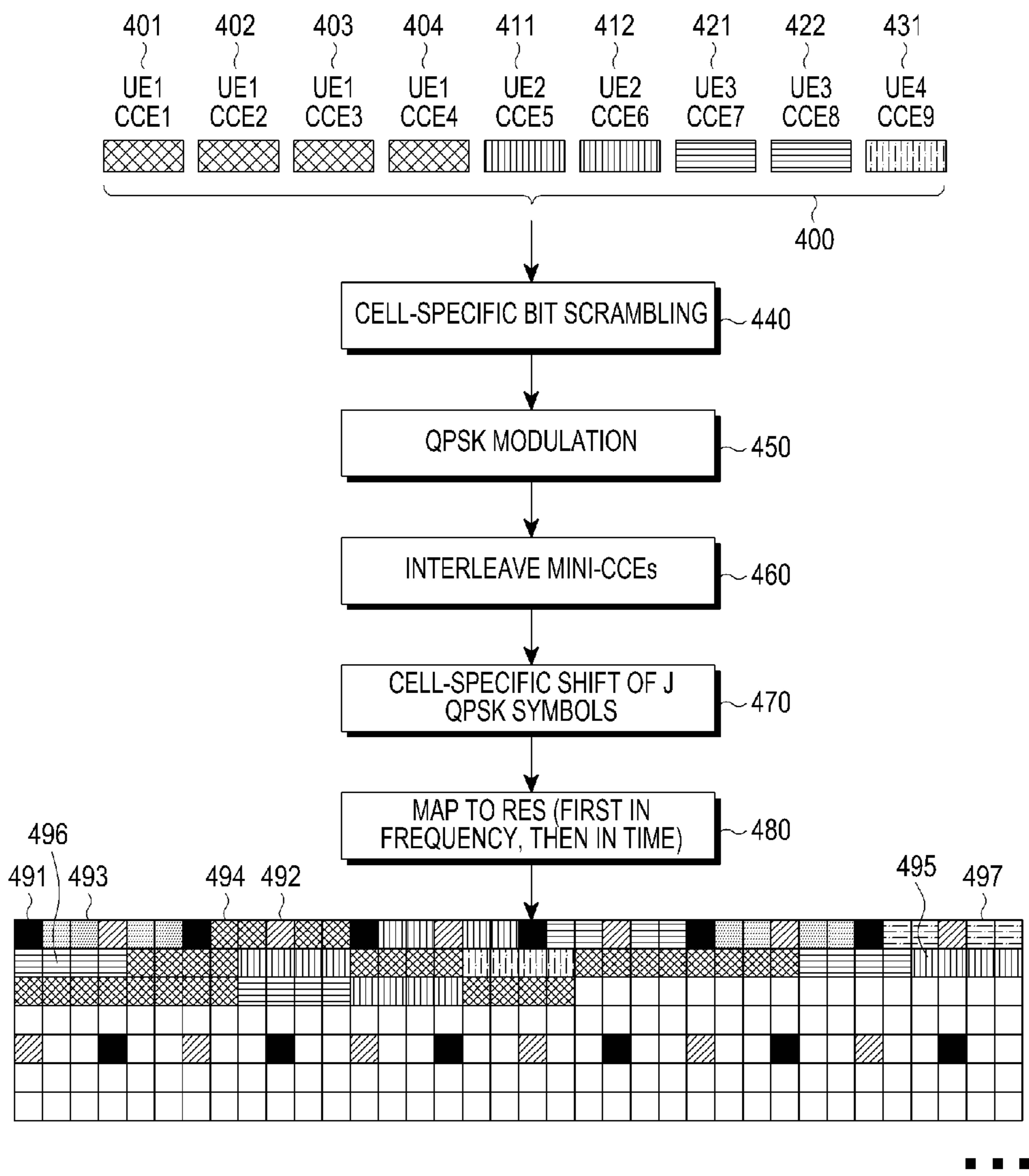
FIG.4 (PRIOR ART)
