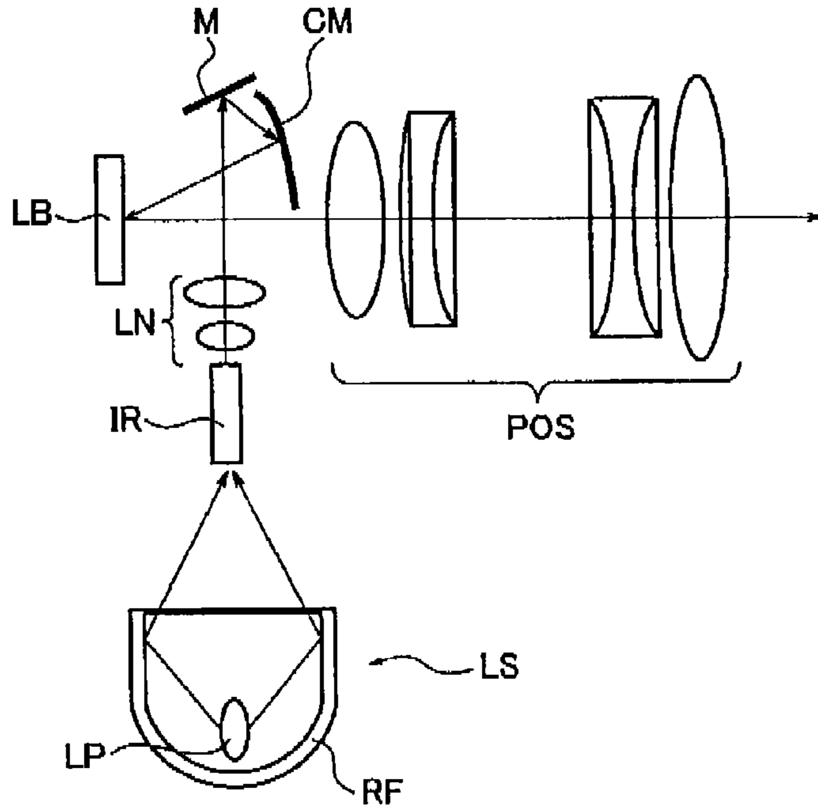
FIG. 1 PRIOR ART
