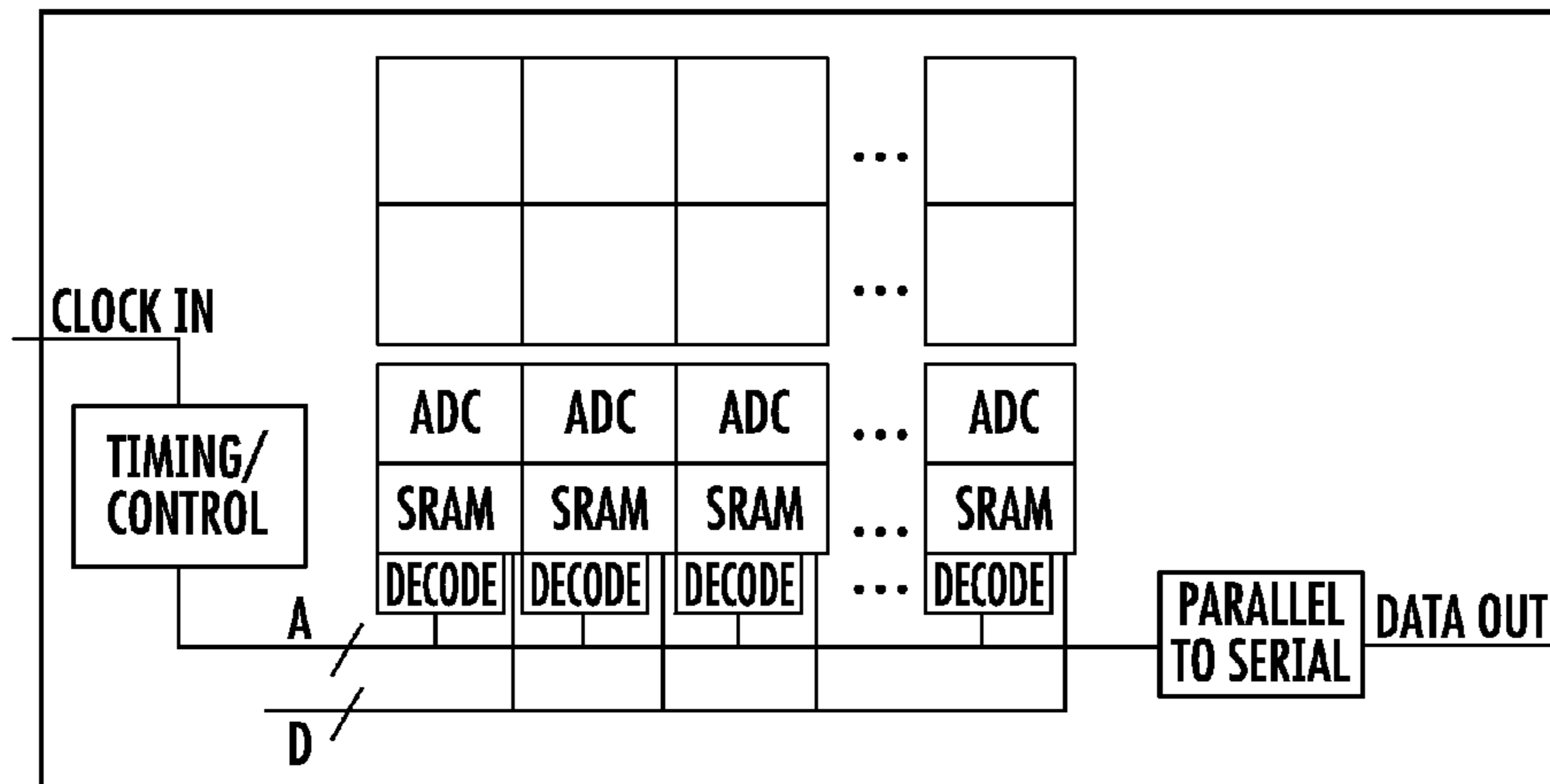
FIG. 9 (PRIOR ART)
