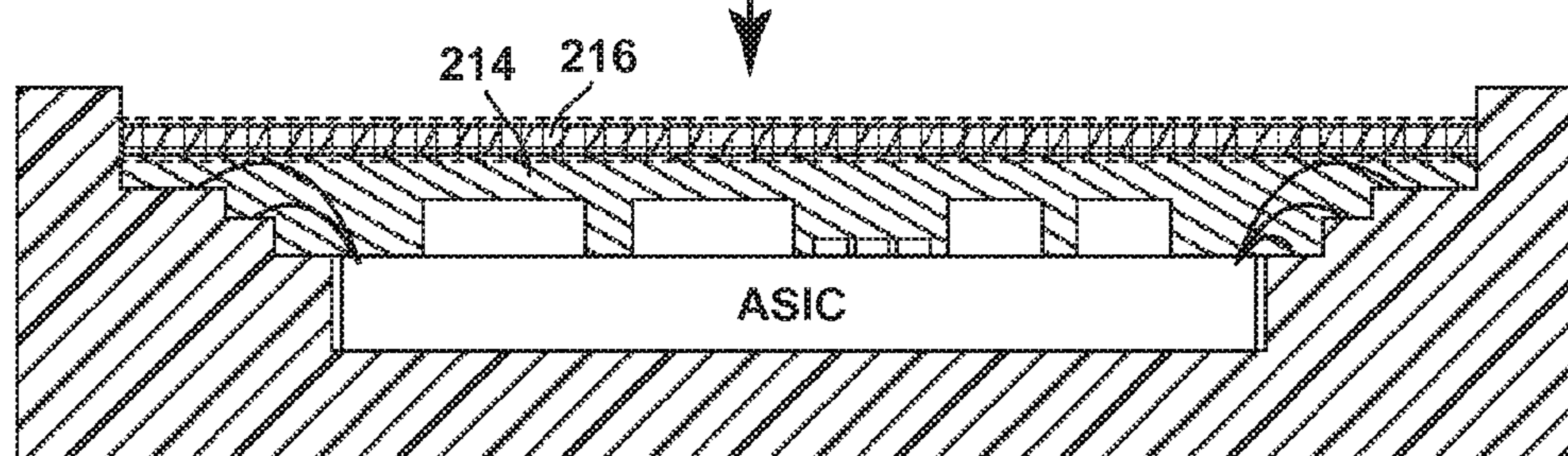
PERIMETER DEEP-SEAL PROCESS
