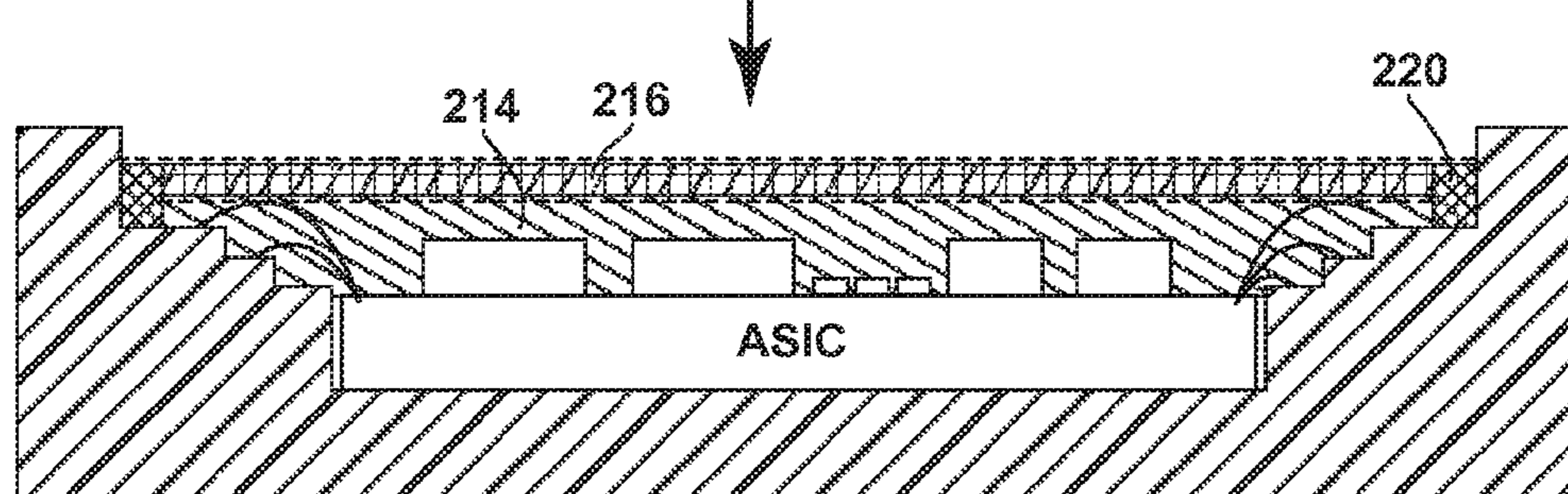
LID & SEAL THE PACKAGE FIG. 2D 204
