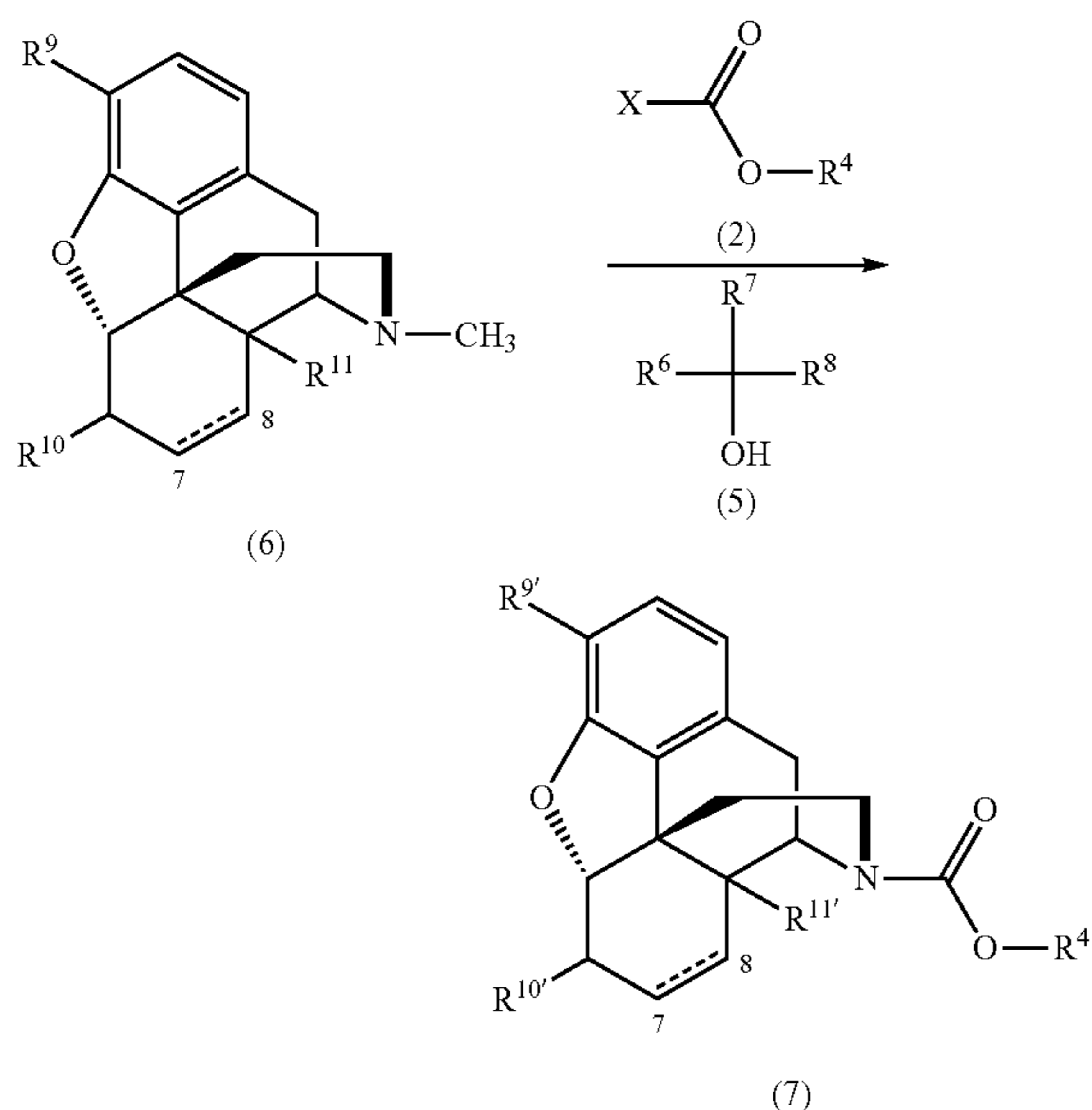
Scheme 4
