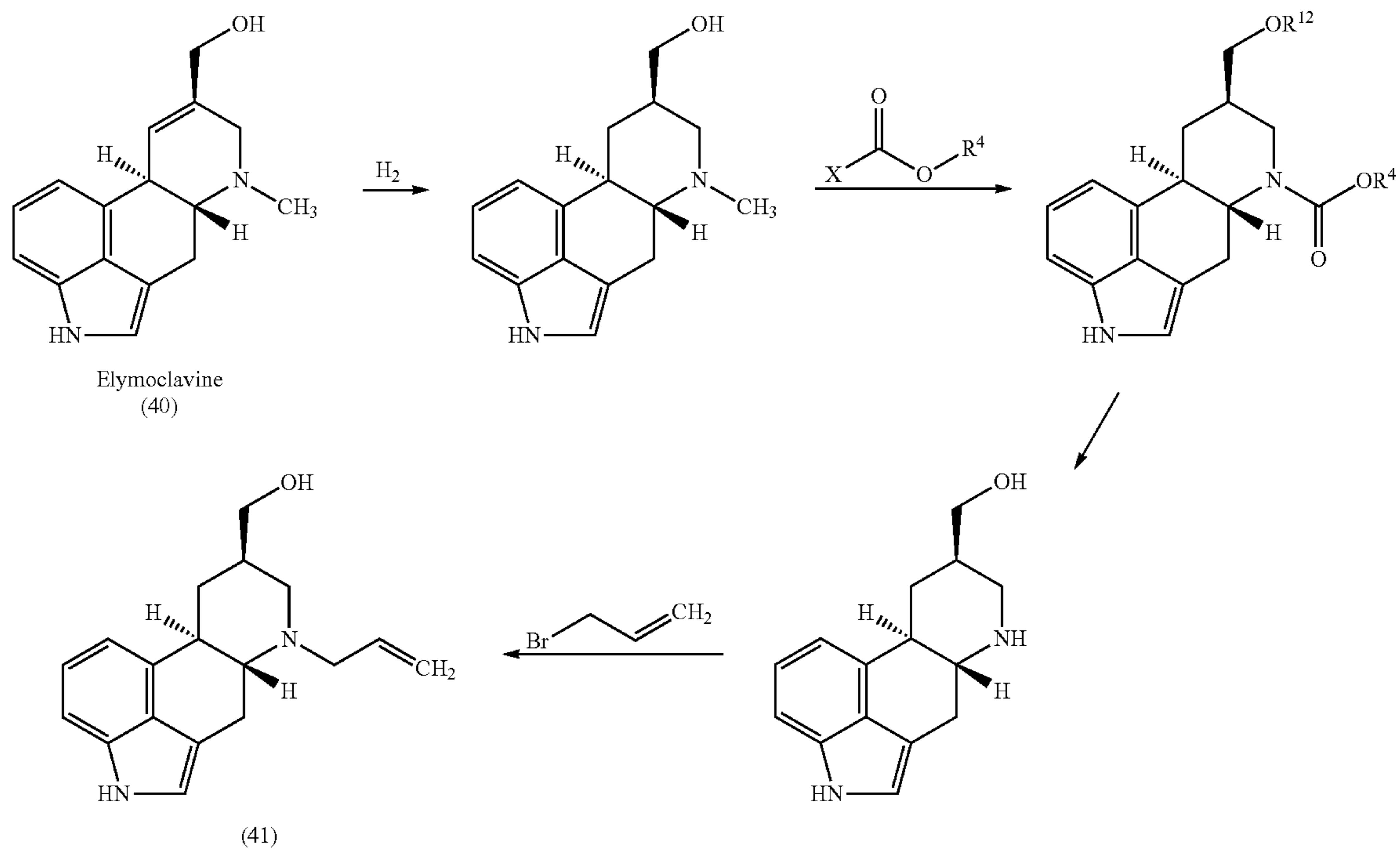
Scheme 14
