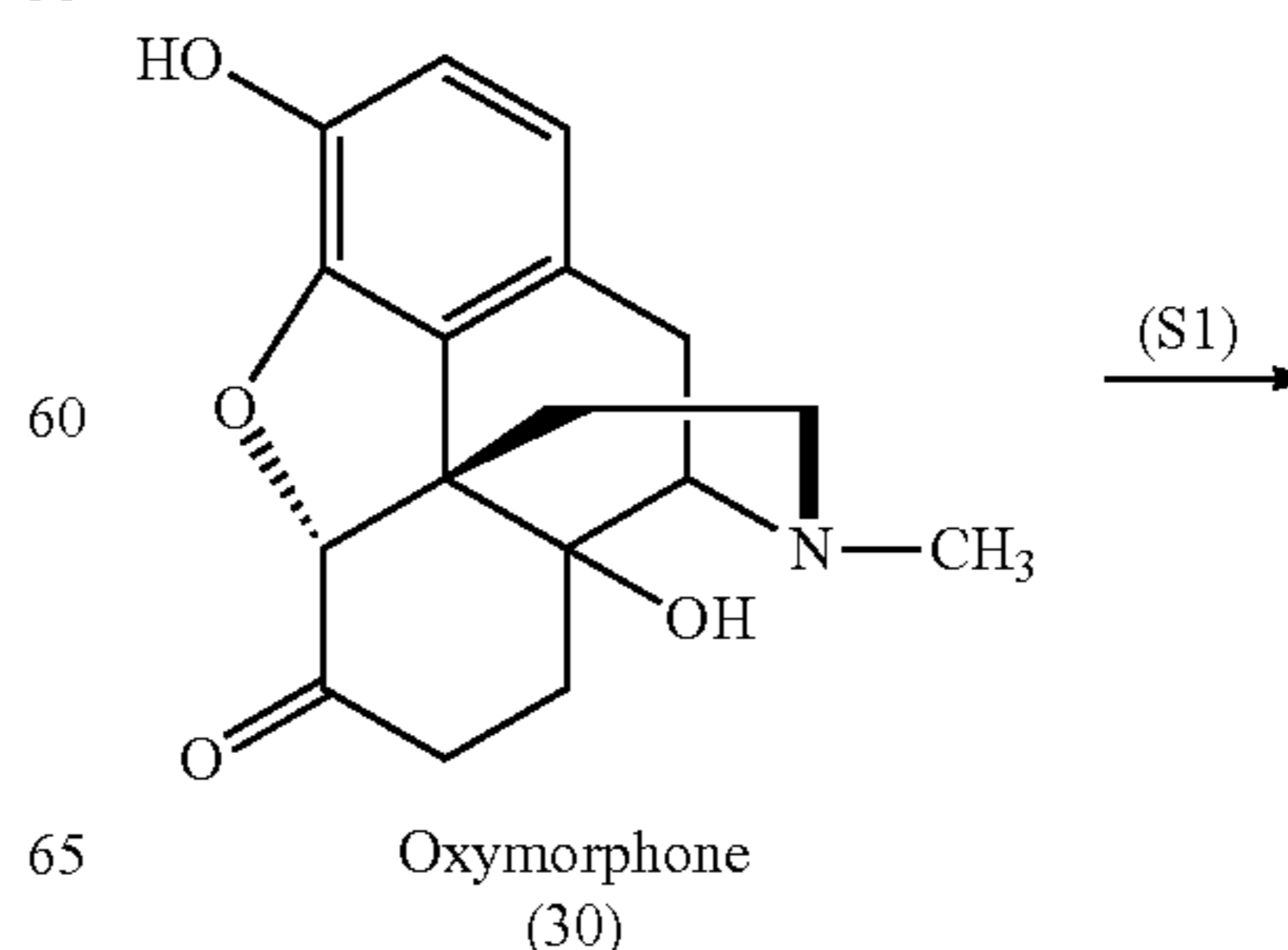
Scheme 8
