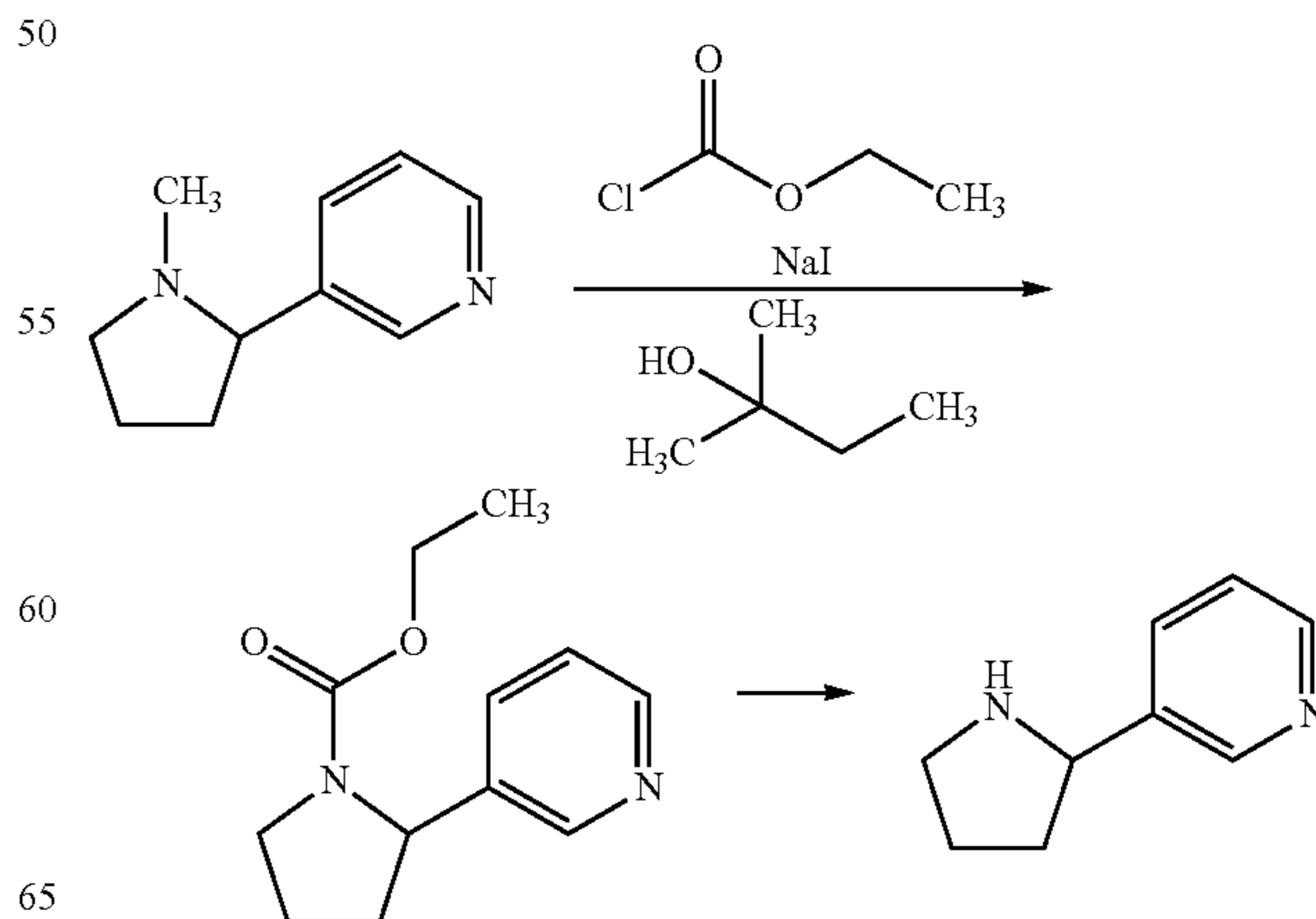
Scheme 19: Nicotine
