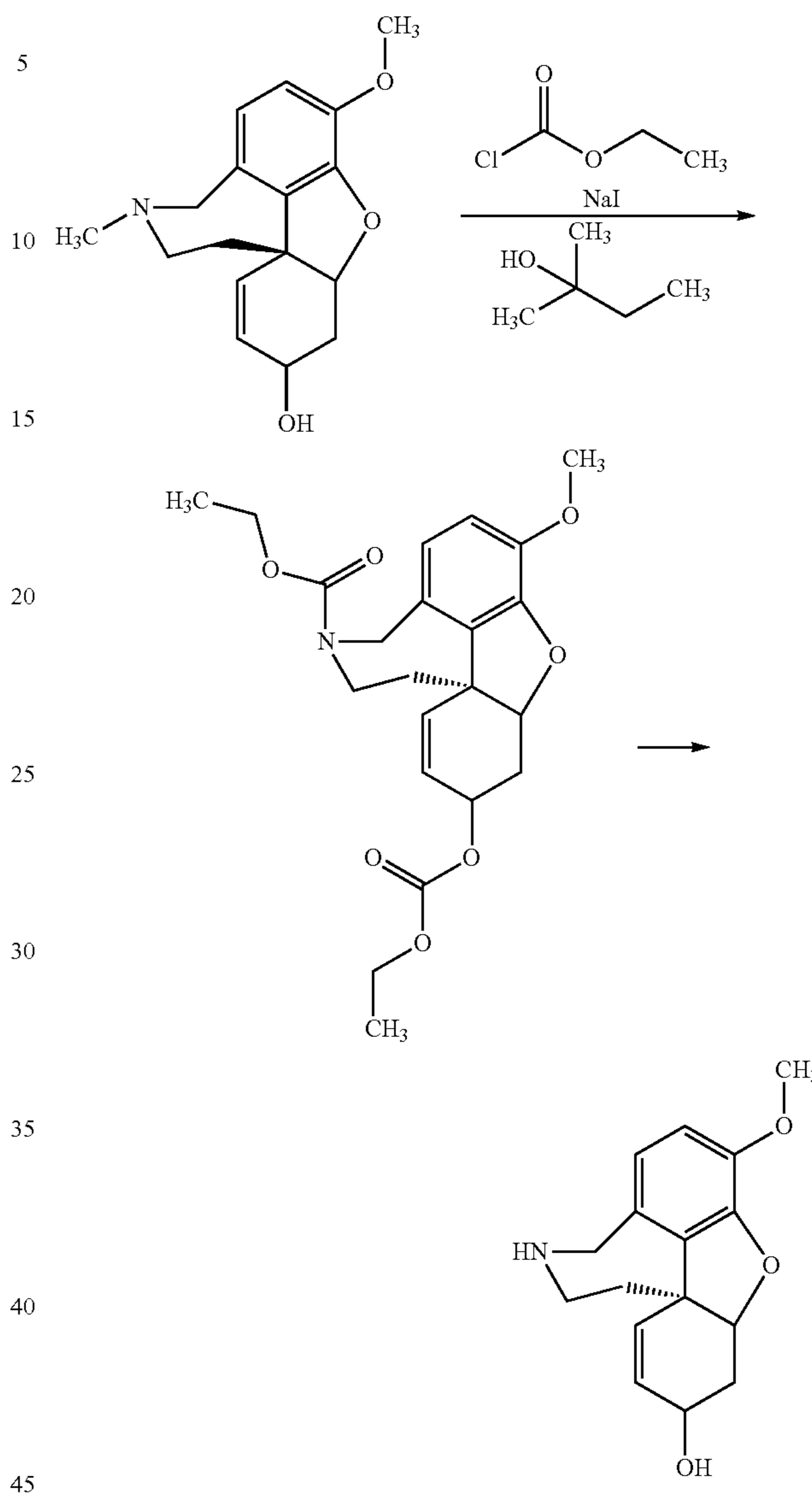
Scheme 18: Galanthamine
