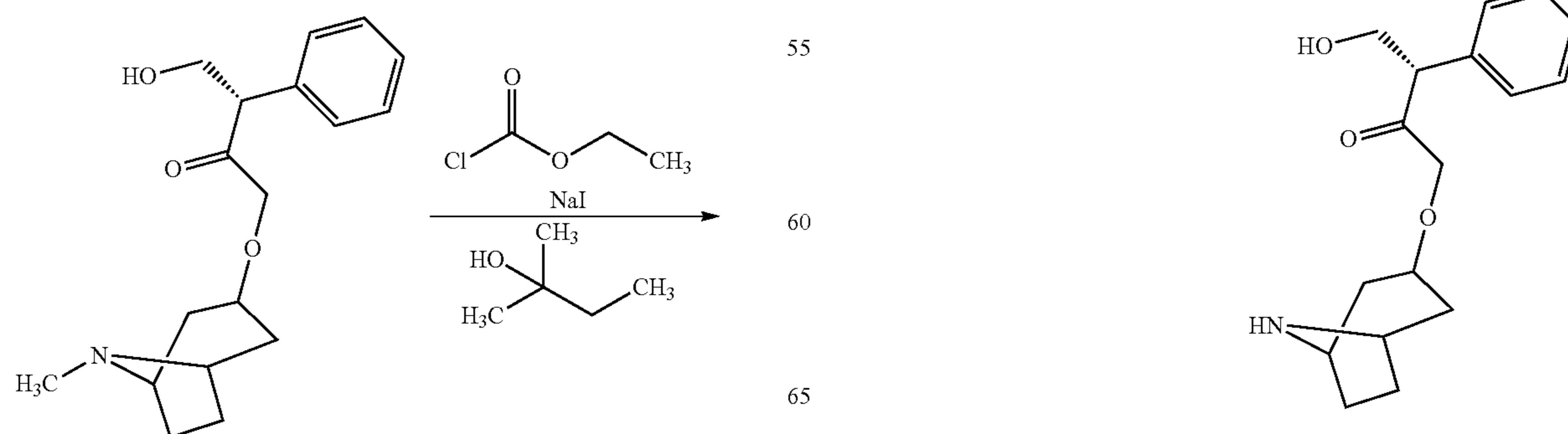
Scheme 15: Atropine
