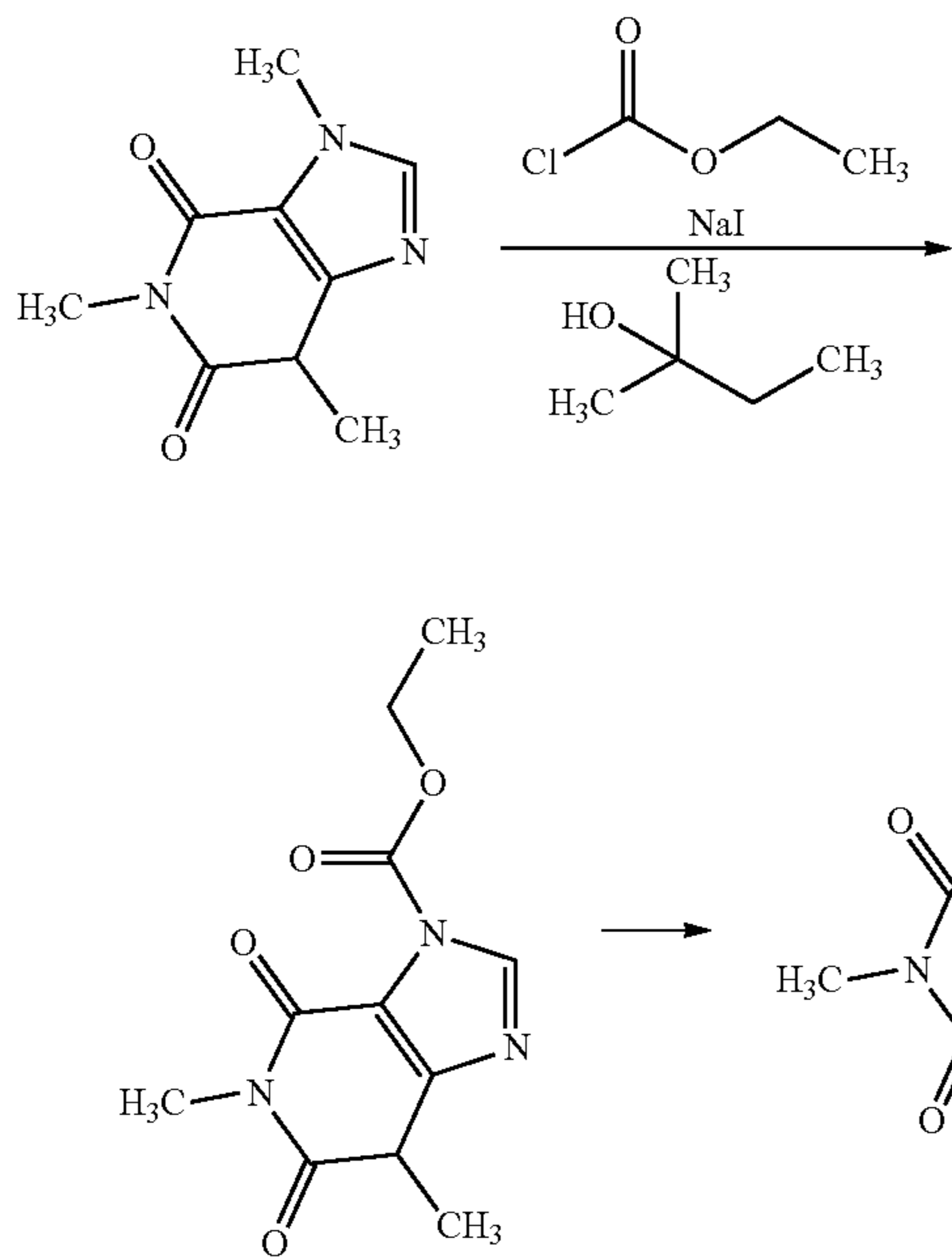
Scheme 16: Caffeine
