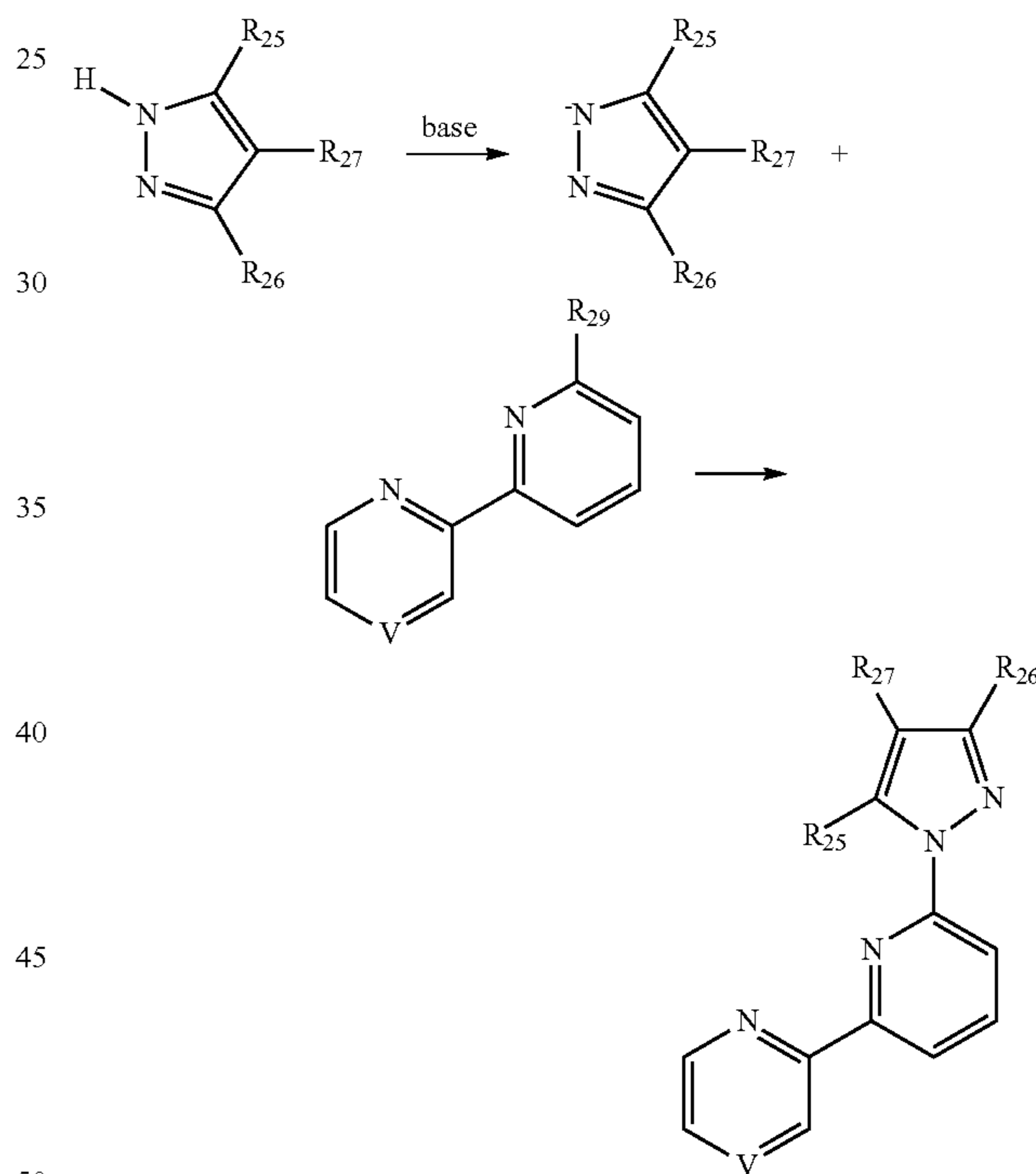
Scheme IV: Formation of a substitute 1-(pyridin-2-yl)pyrazole.
