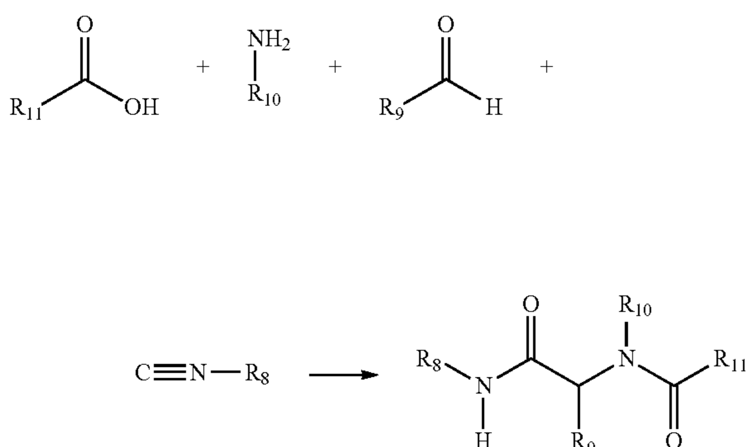
Scheme VI: Ugi reaction to form the compounds represented by Formula III.
