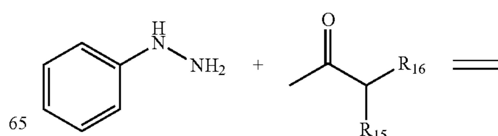
Scheme 3. Typical synthesis of indolium intermediate
