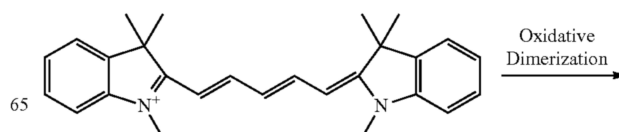
Scheme 2. Oxidative dimerization of carbocyanines
