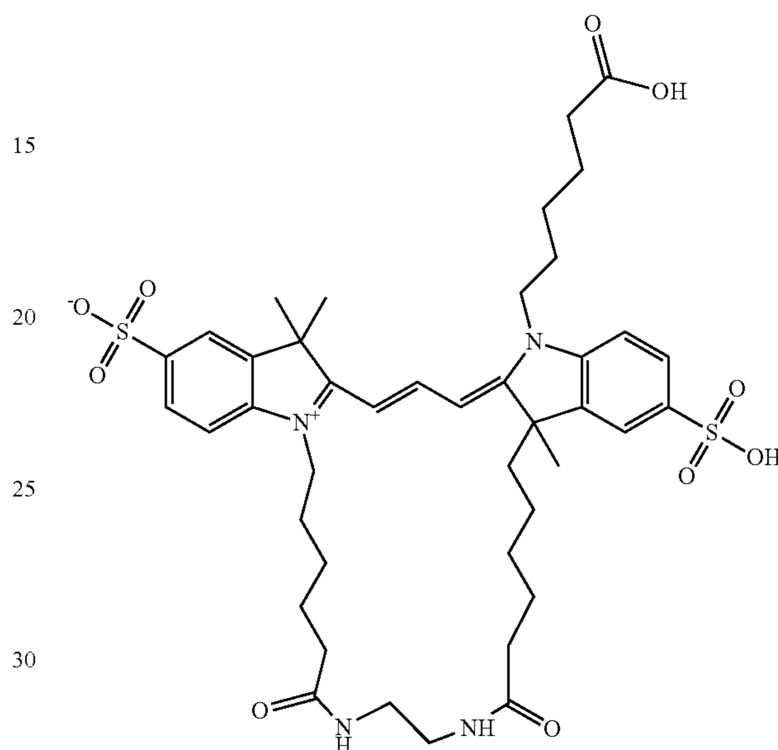
Compound 55
