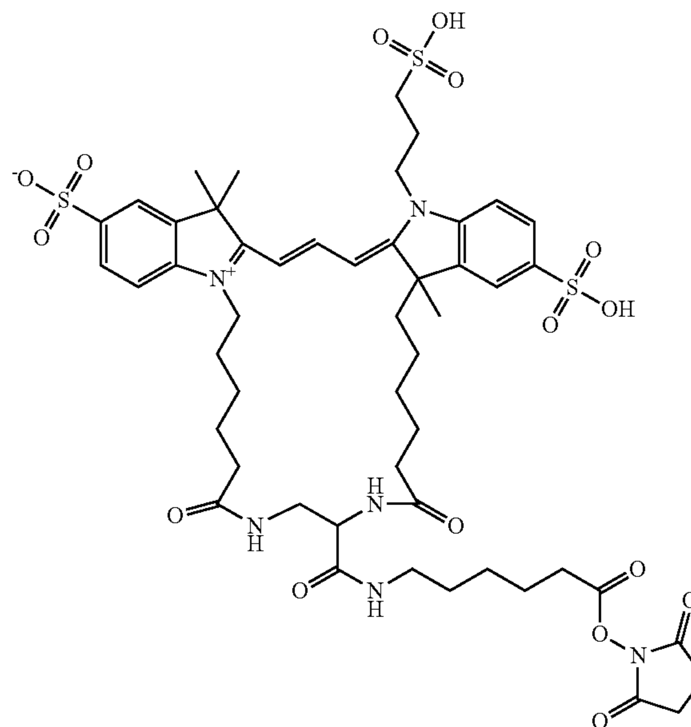
Compound 20
