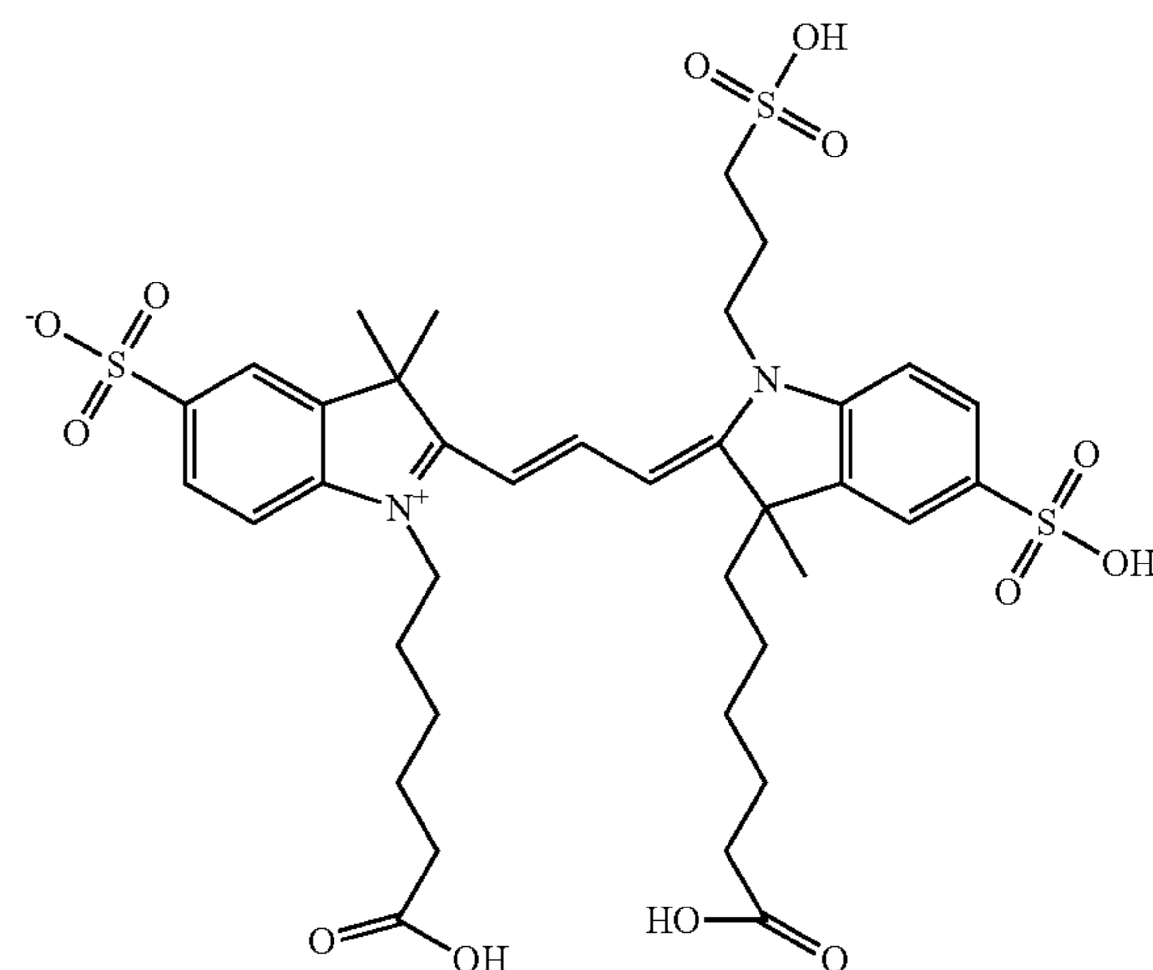
Compound 18
