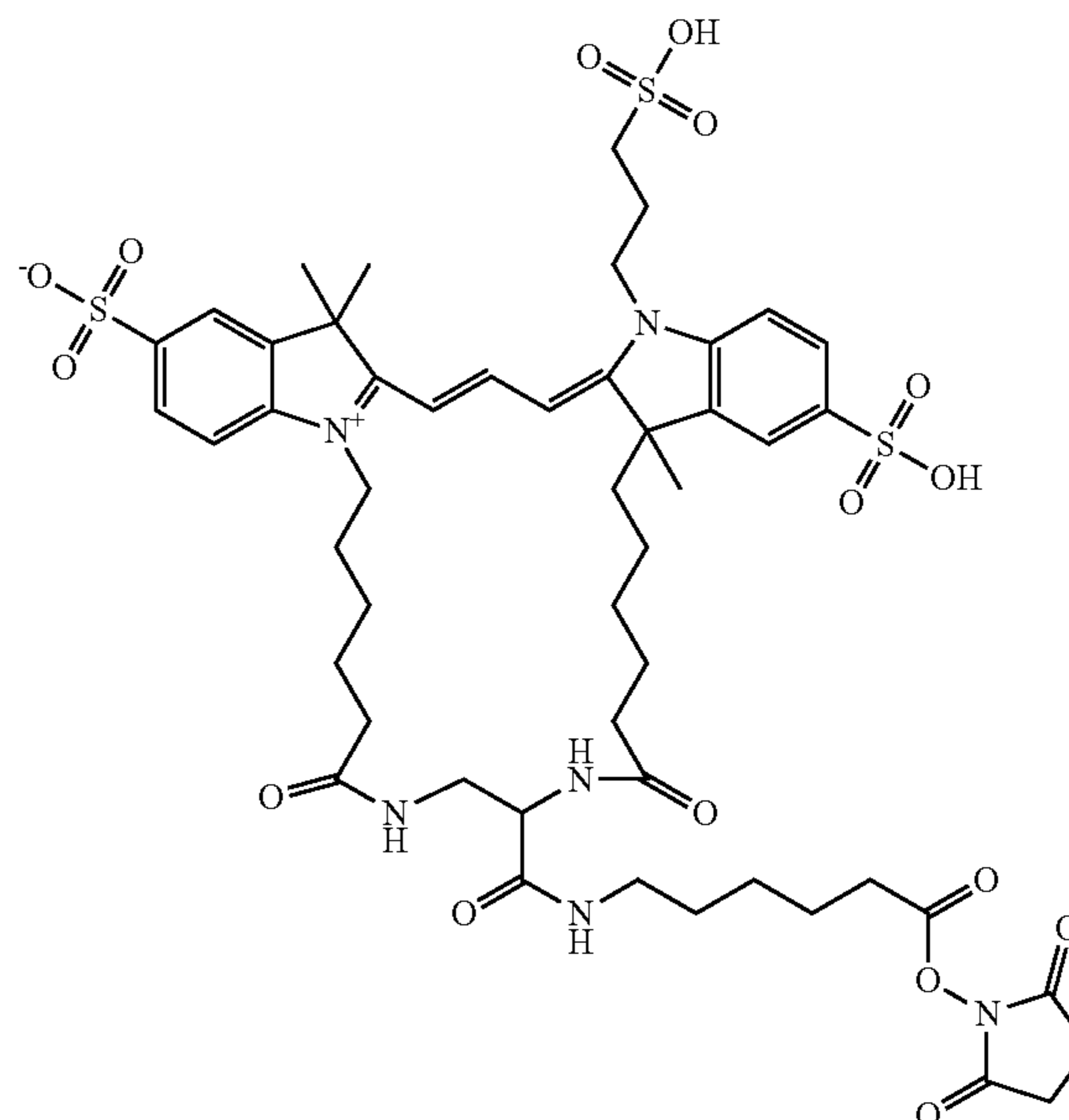
Compound 20
