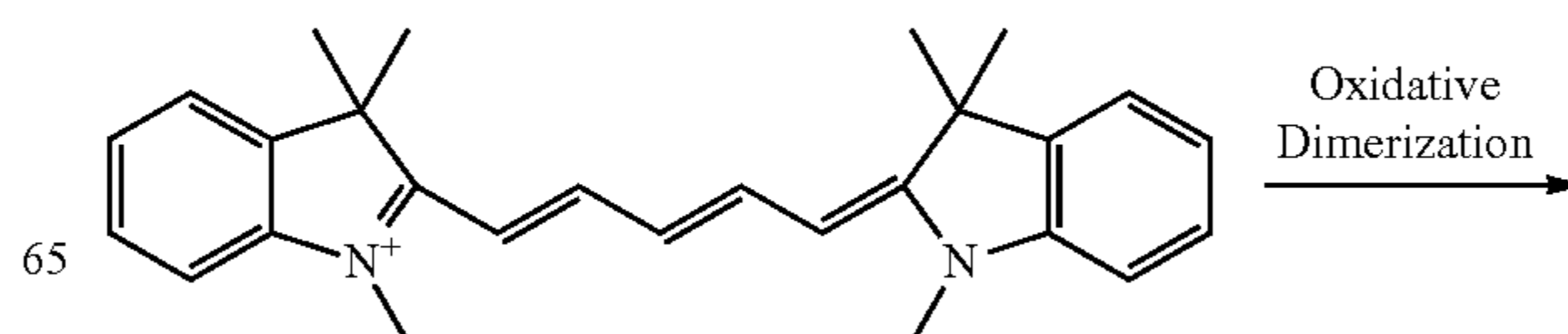
Scheme 2. Oxidative dimerization of carbocyanines
