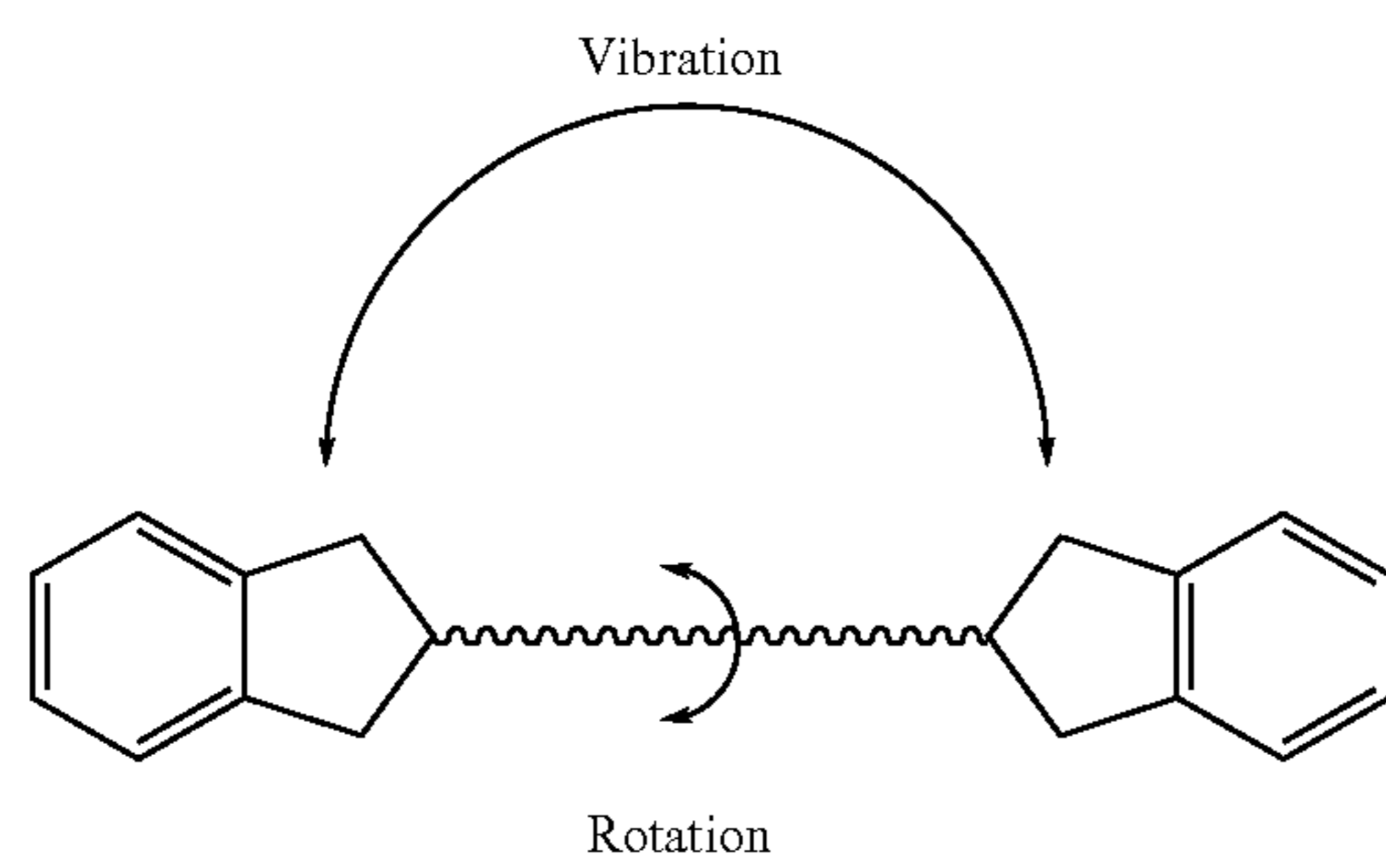
Scheme 1. 'Loose Belt Effect' through vibration and rotation around the middle conjugated double bonds
