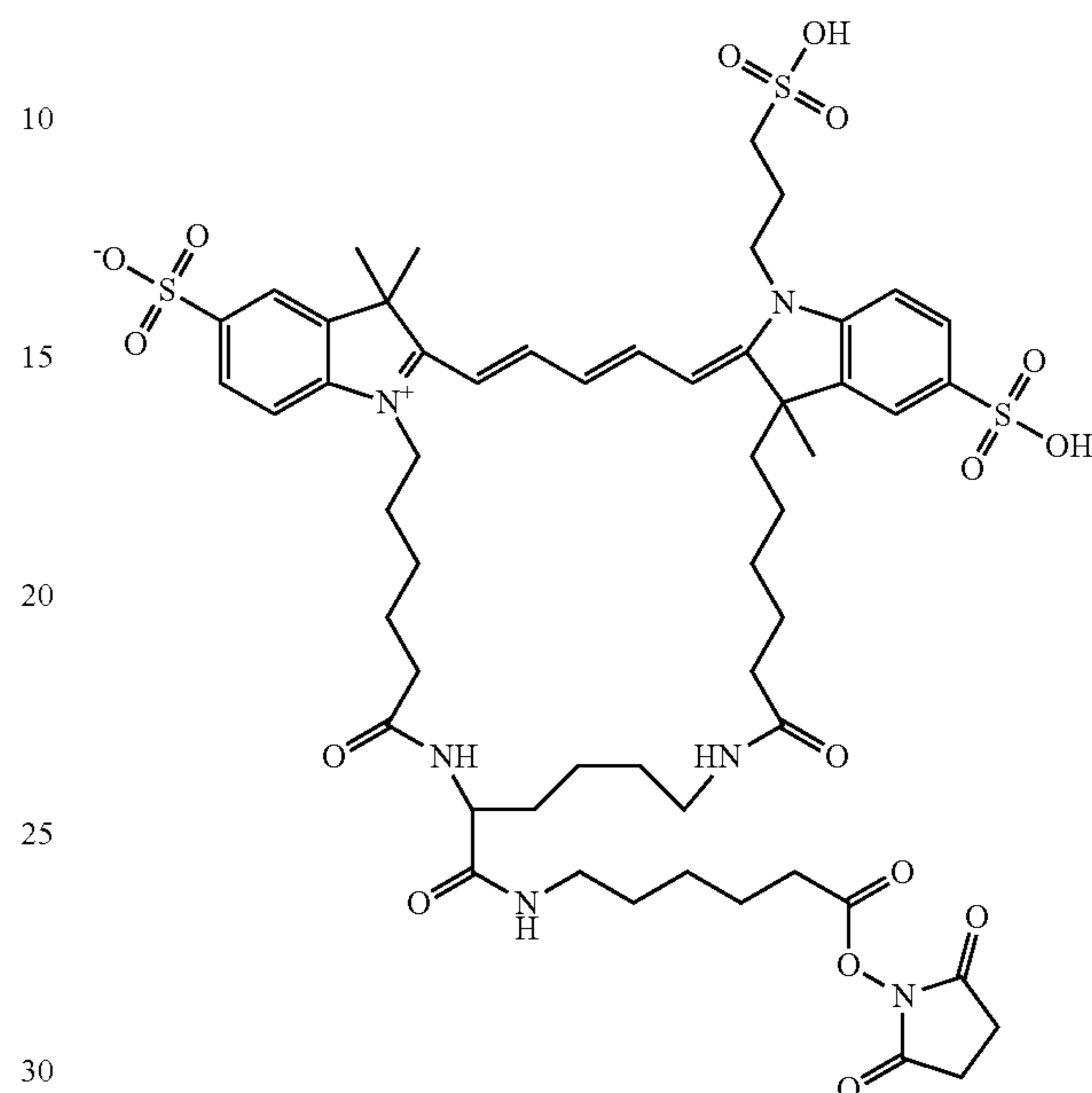
Compound 14
