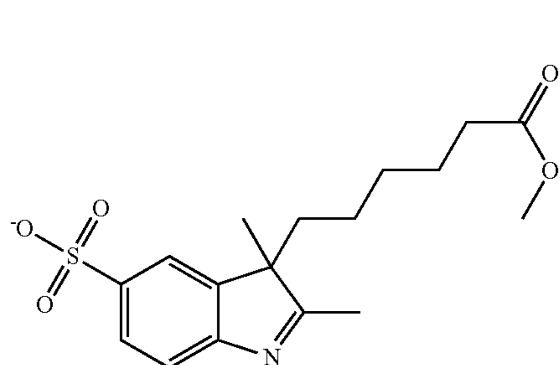
Compound 5
