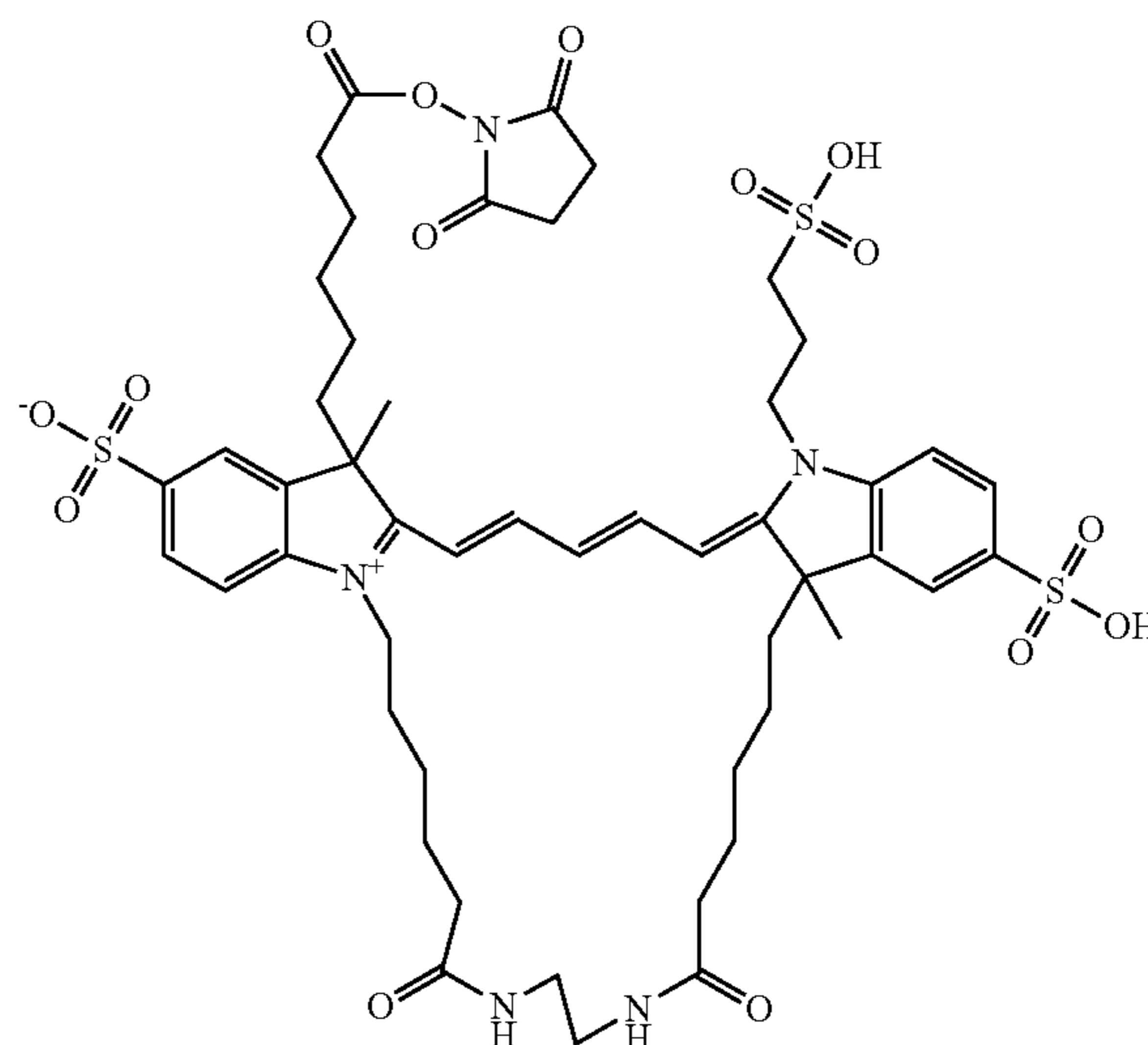
Compound 17
