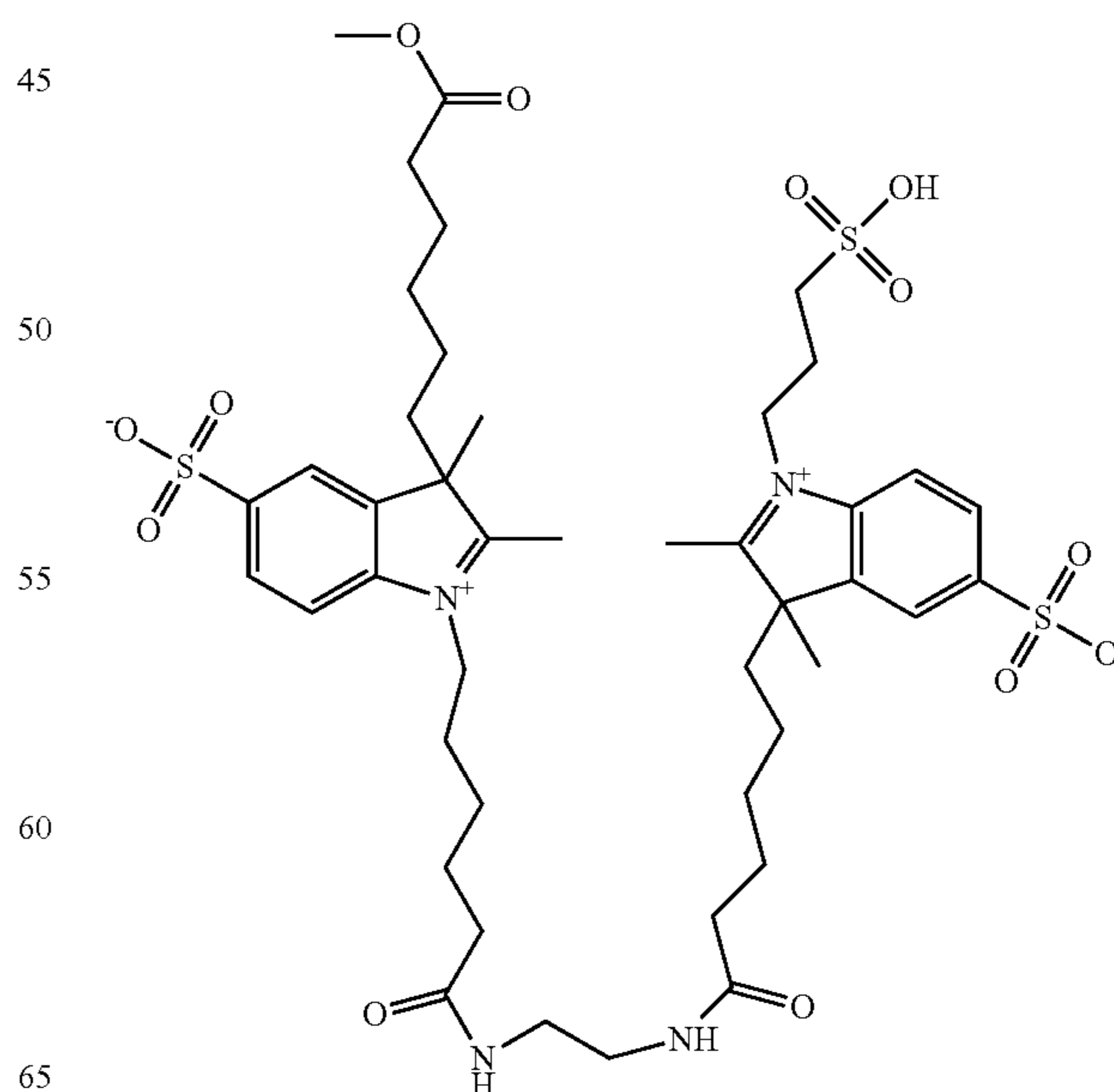
Compound 48
