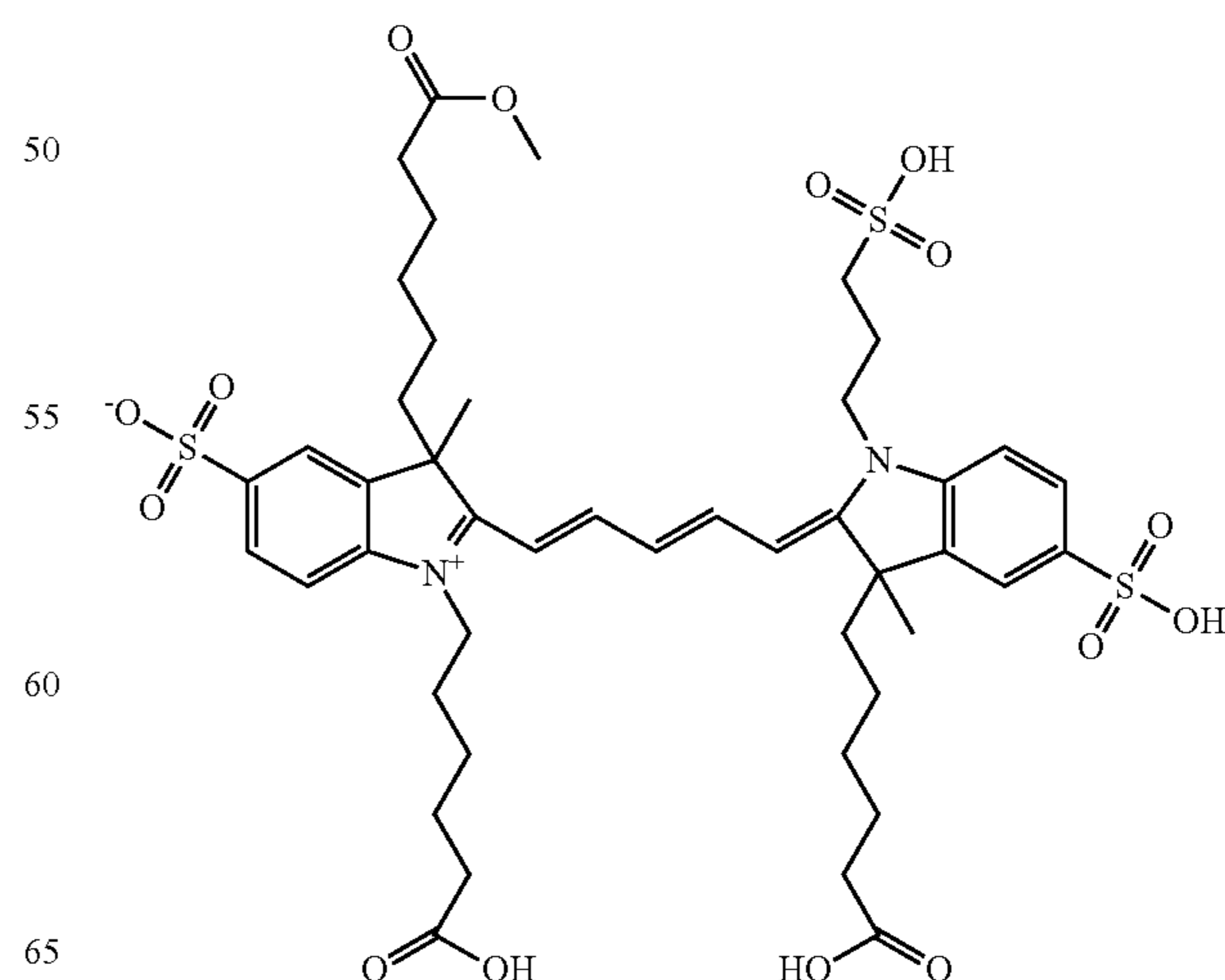
Compound 15
