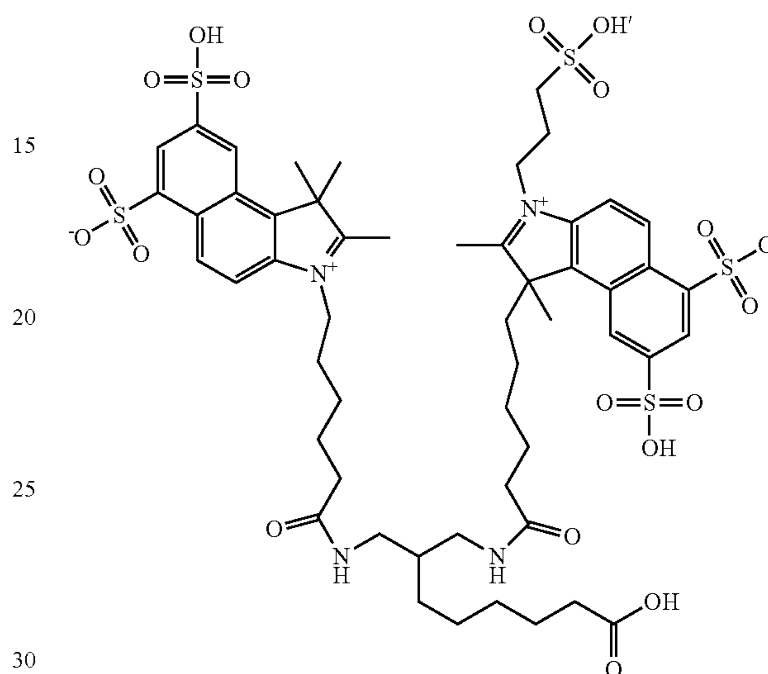
Compound 47
