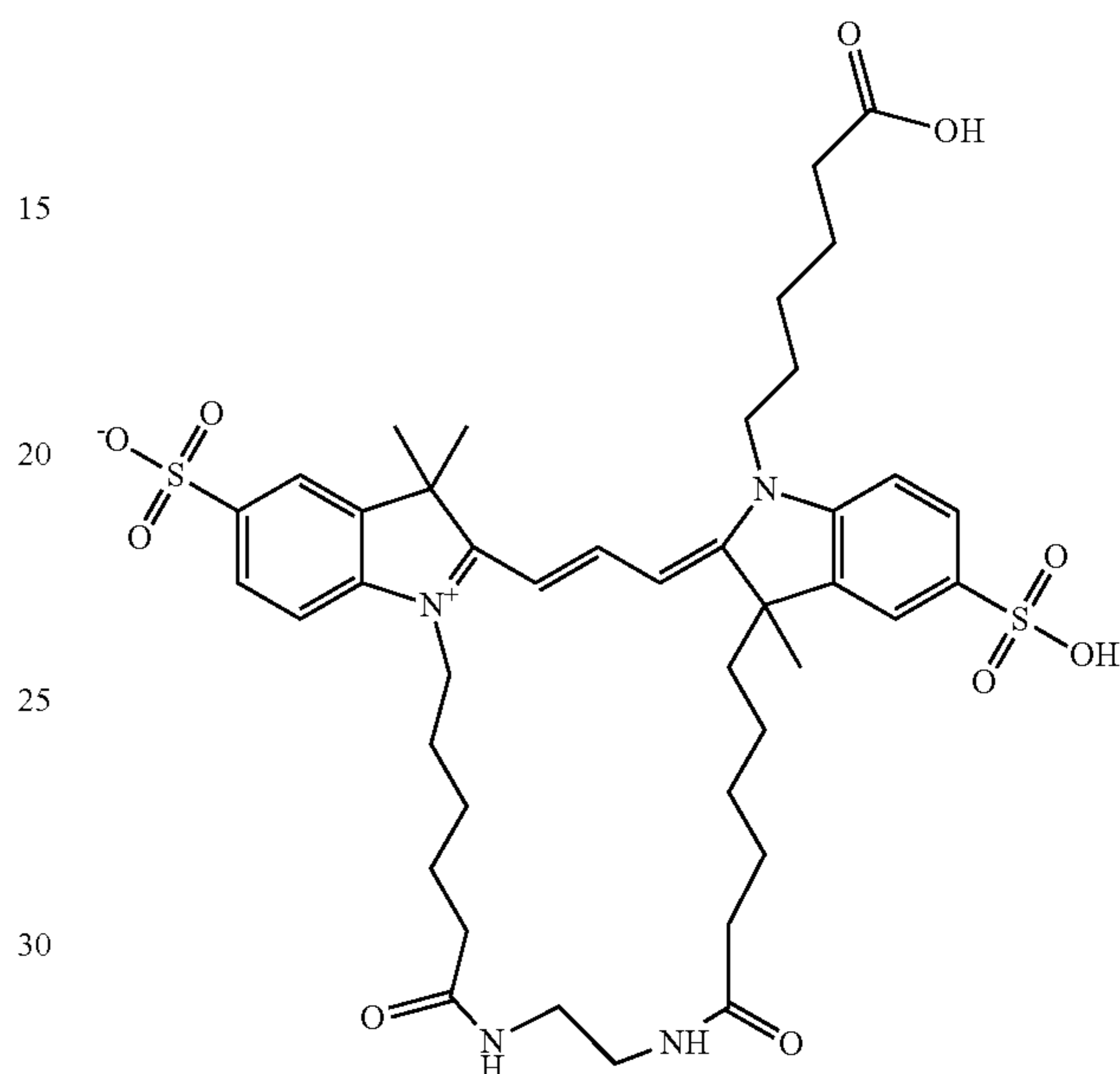
Compound 55
