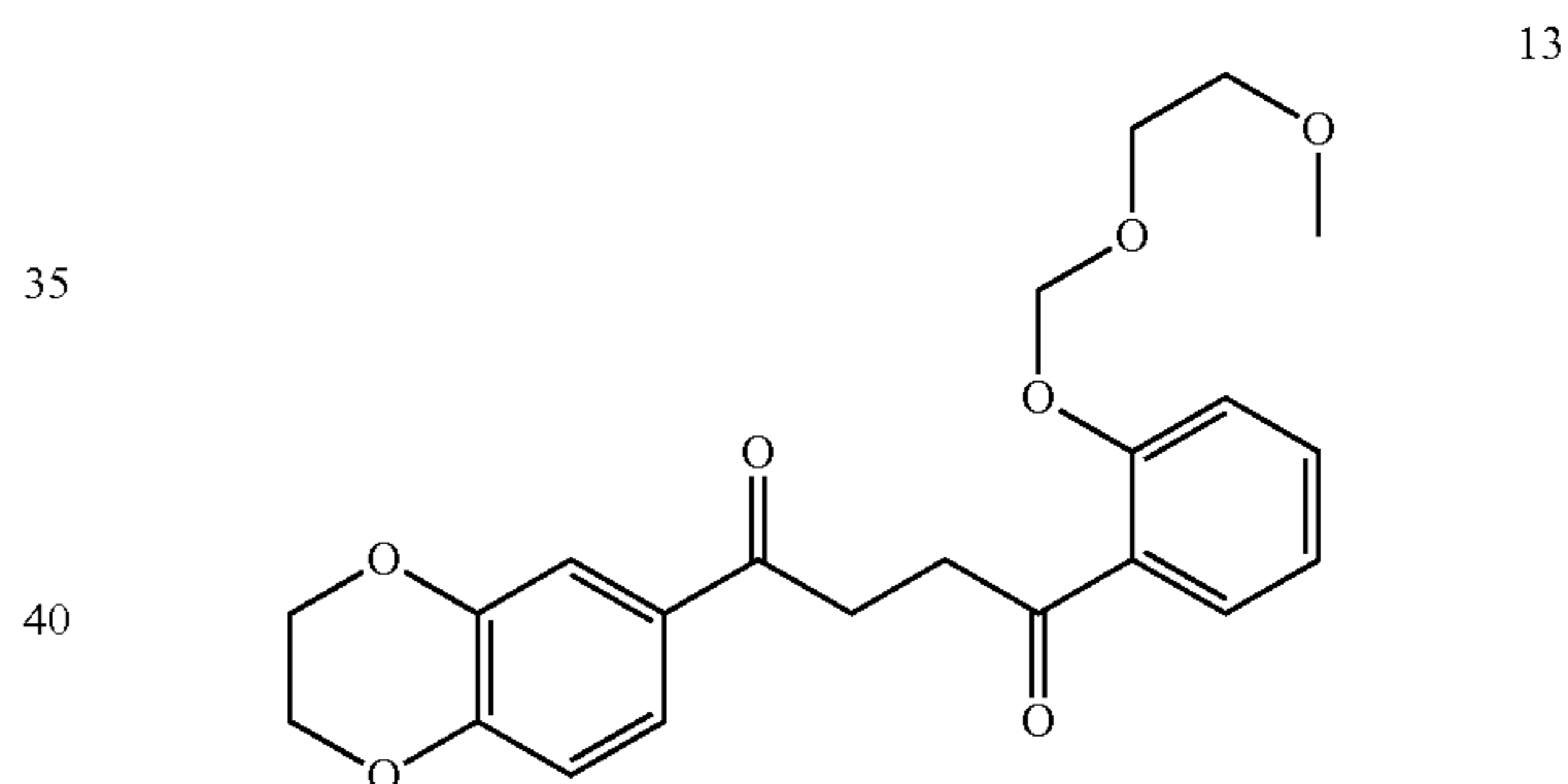
1-(2,3-dihydrobenzo[b][1,4]dioxin-6-yl)-4-(4-methoxyphenyl)butane-1,4-dione 10
