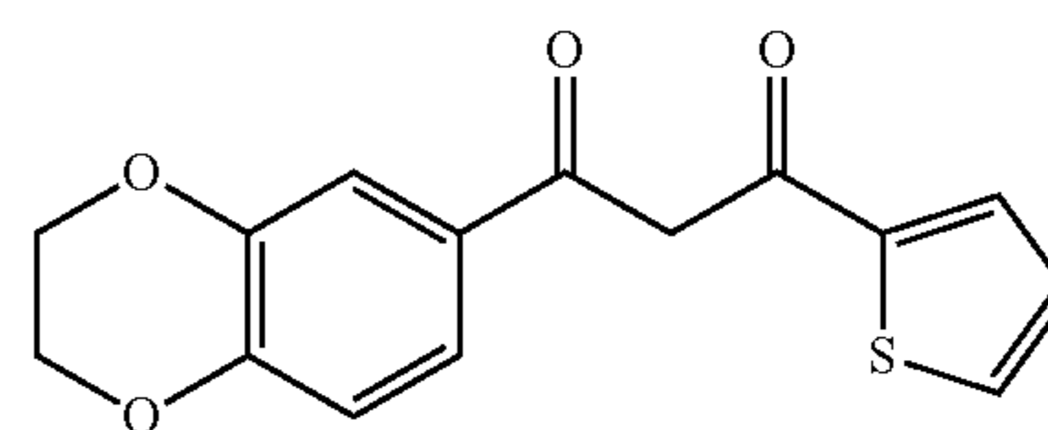
1-(2,3-dihydrobenzo[b][1,4]dioxin-6-yl)-3-(thiophen-2-yl)propane-1,3-dione 16
