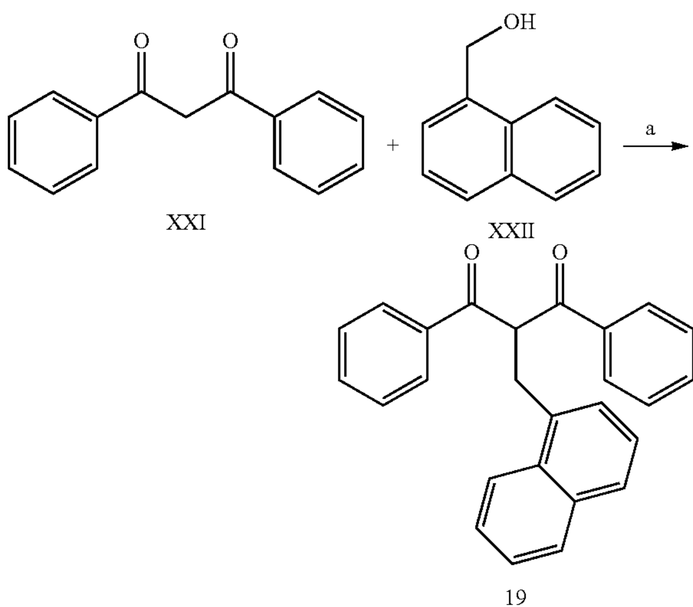
Scheme 10
