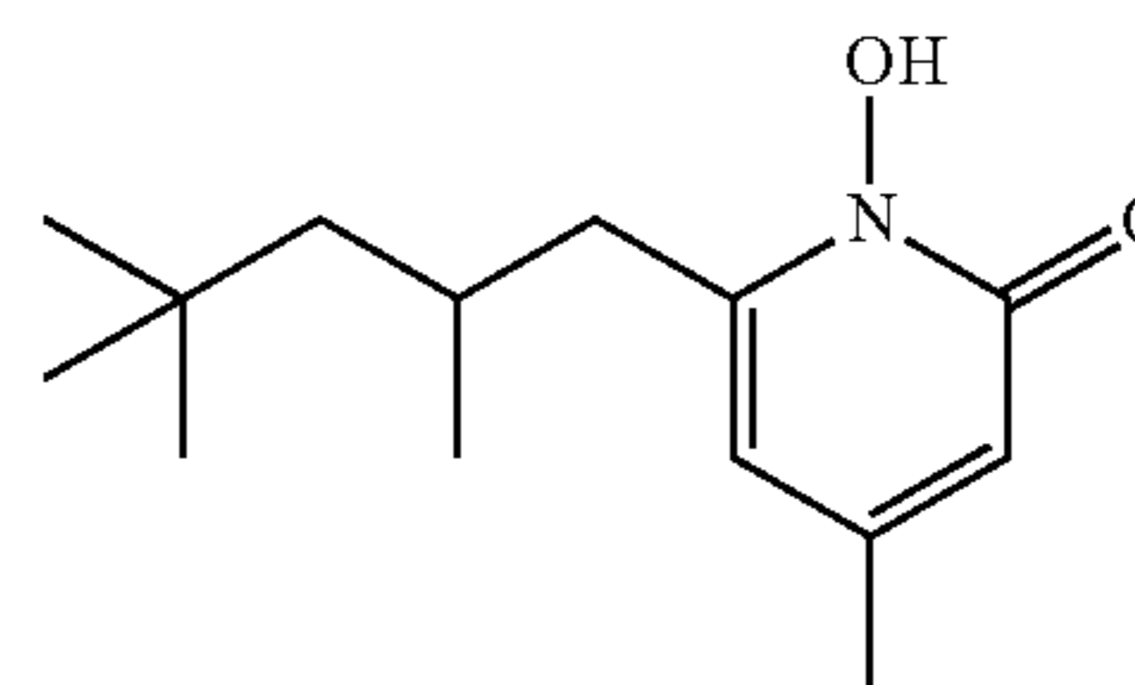
piroctone (II-d) (CAS 50650-76-5)
