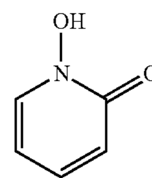
1-hydroxy-2-pyridinone (II-a) (CAS 822-89-9)
