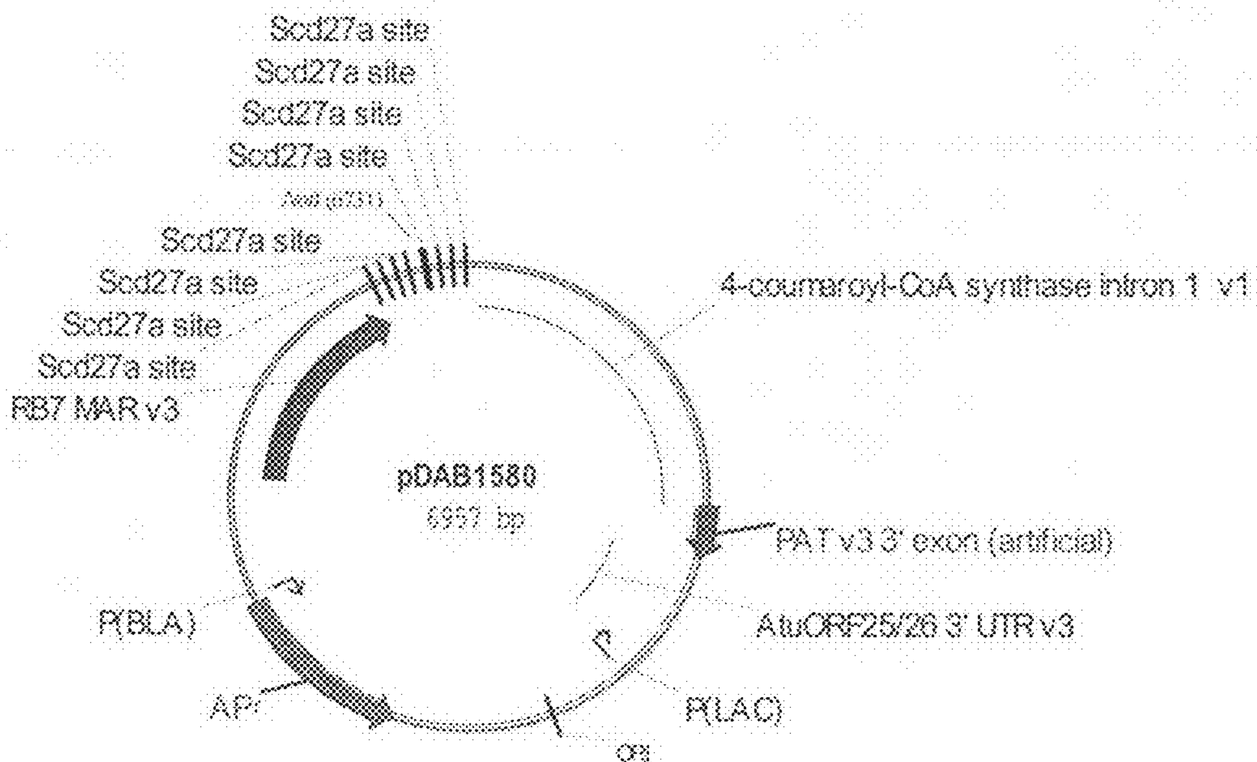
Figure 19: Schematic representation of plasmid pDAB1580
