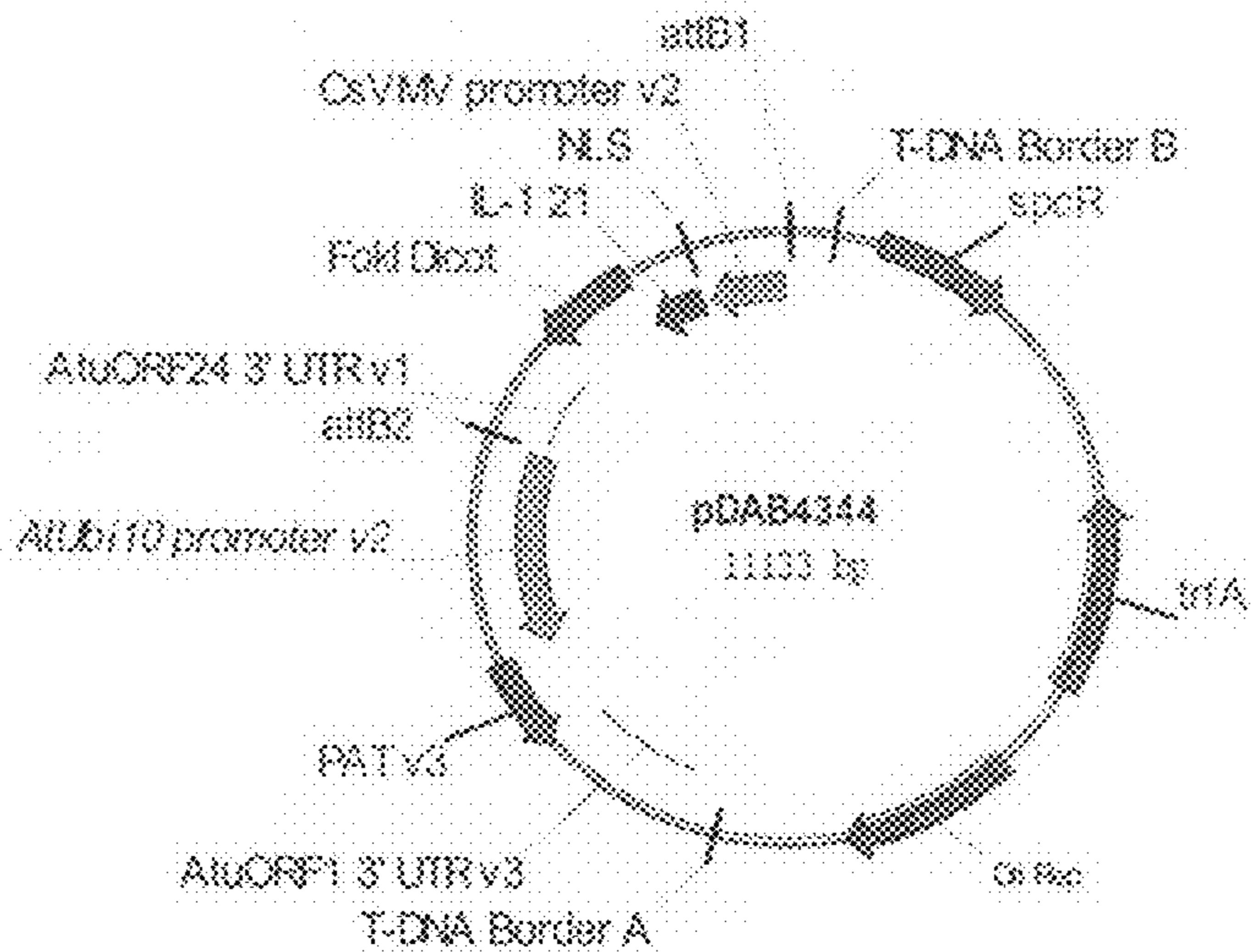
Figure 44: Schematic representation of plasmid pDAB4344
