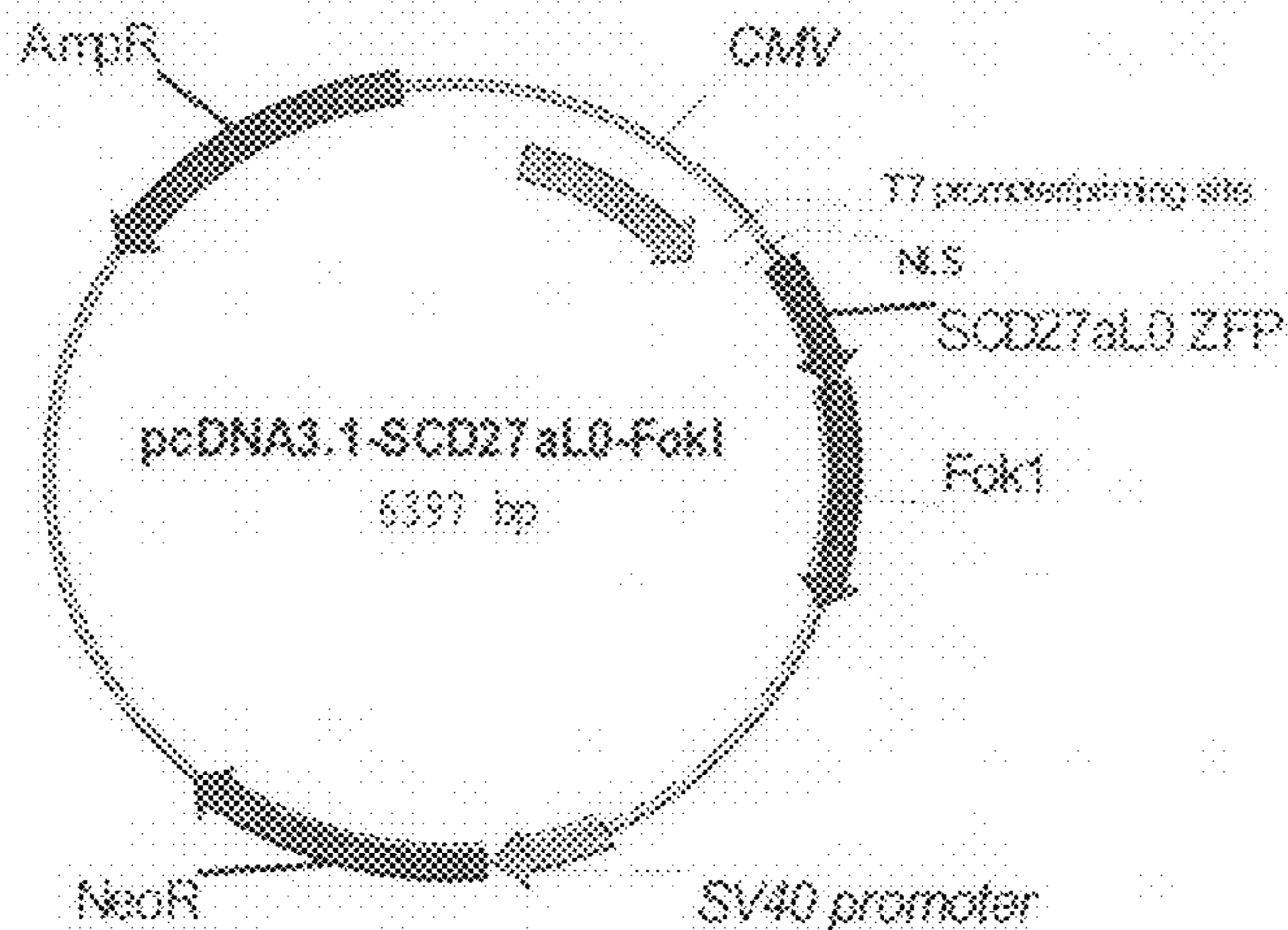
Figure 53: Schematic representation of plasmid pCDNA3.1-SCD27a-L0-FokI
