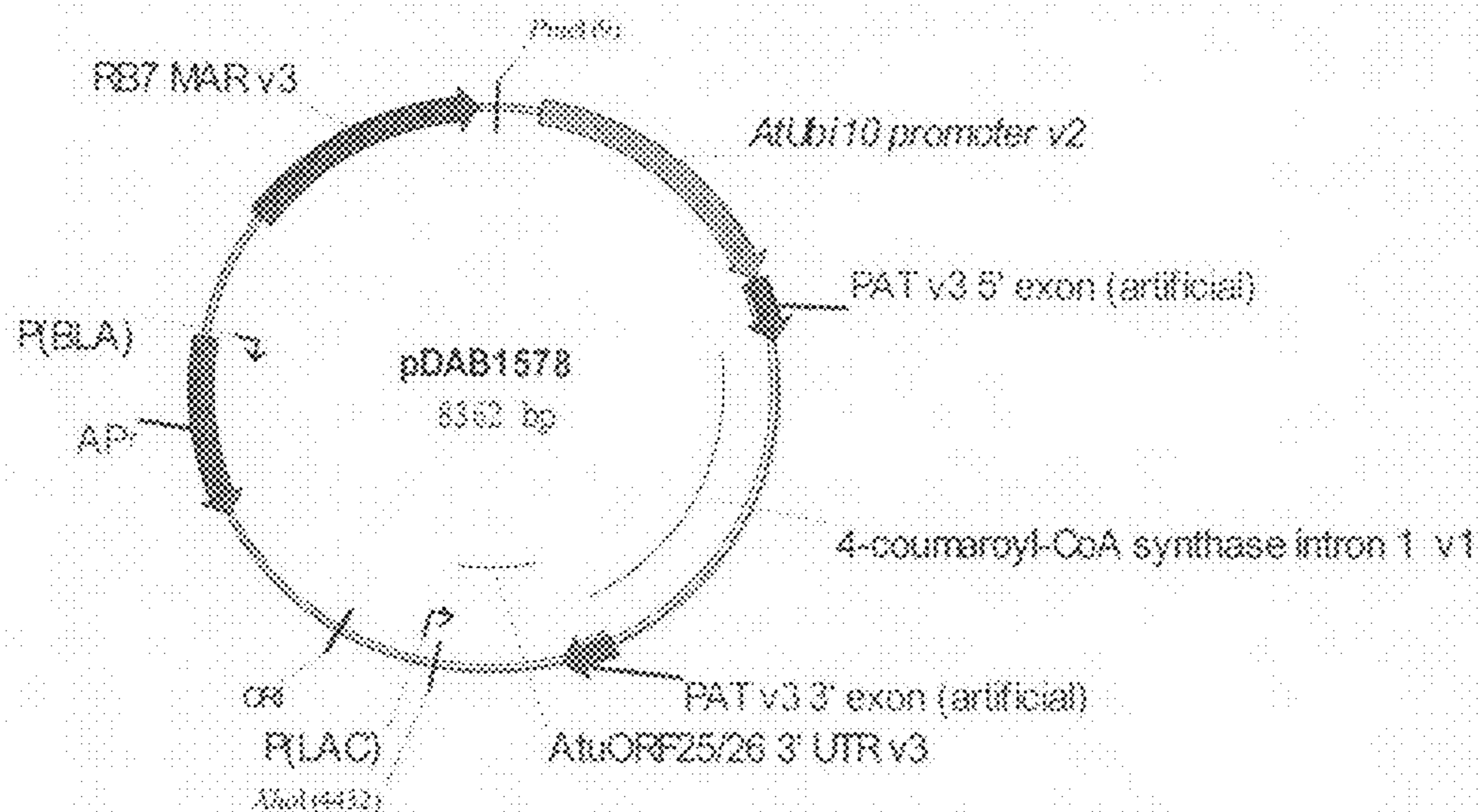
Figure 57: Schematic representation of plasmid pDAB1578
