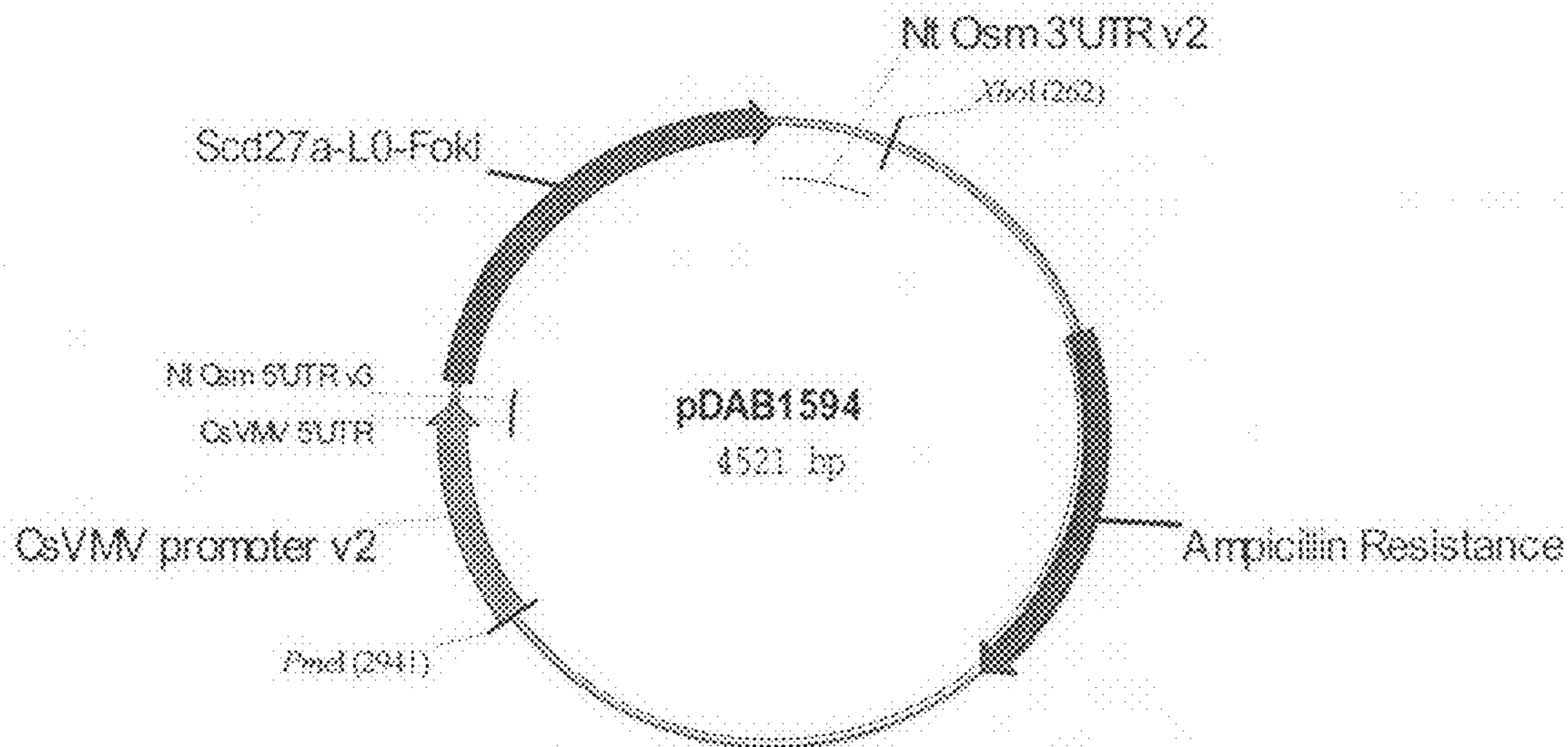
Figure 54: Schematic representation of plasmid pDAB1594
