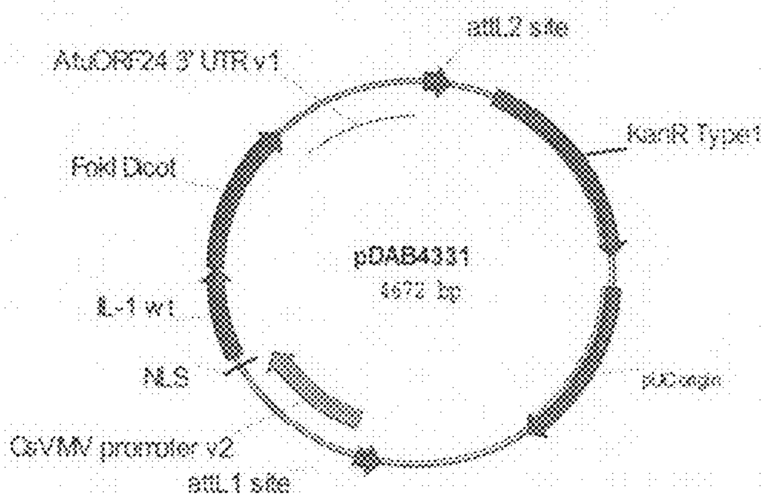
Figure 33: Schematic representation of plasmid pDAB4331
