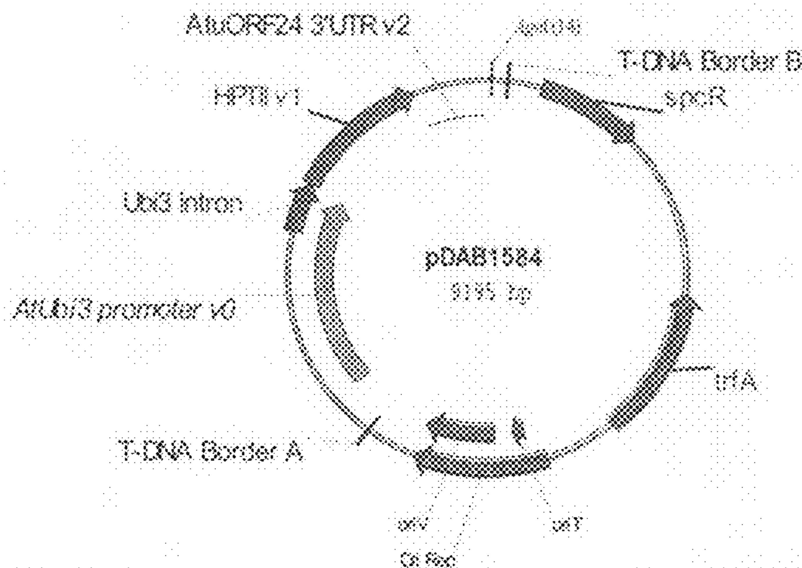
Figure 13: Schematic representation of plasmid pDAB1584
