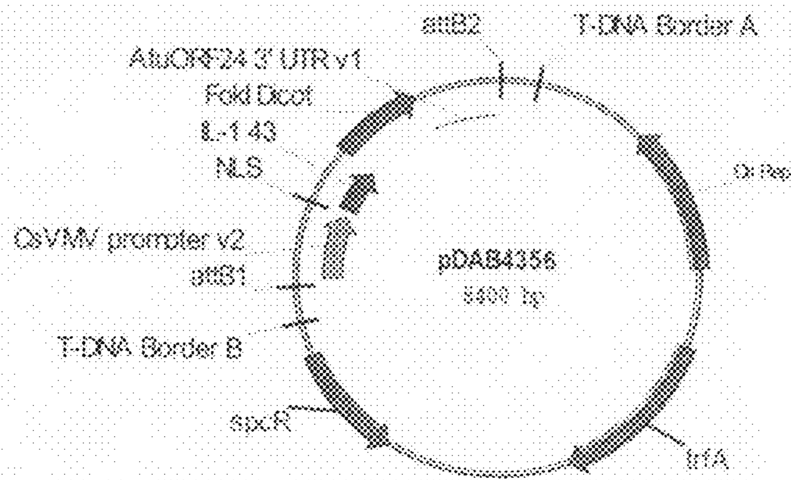
Figure 48: Schematic representation of plasmid pDAB4356
