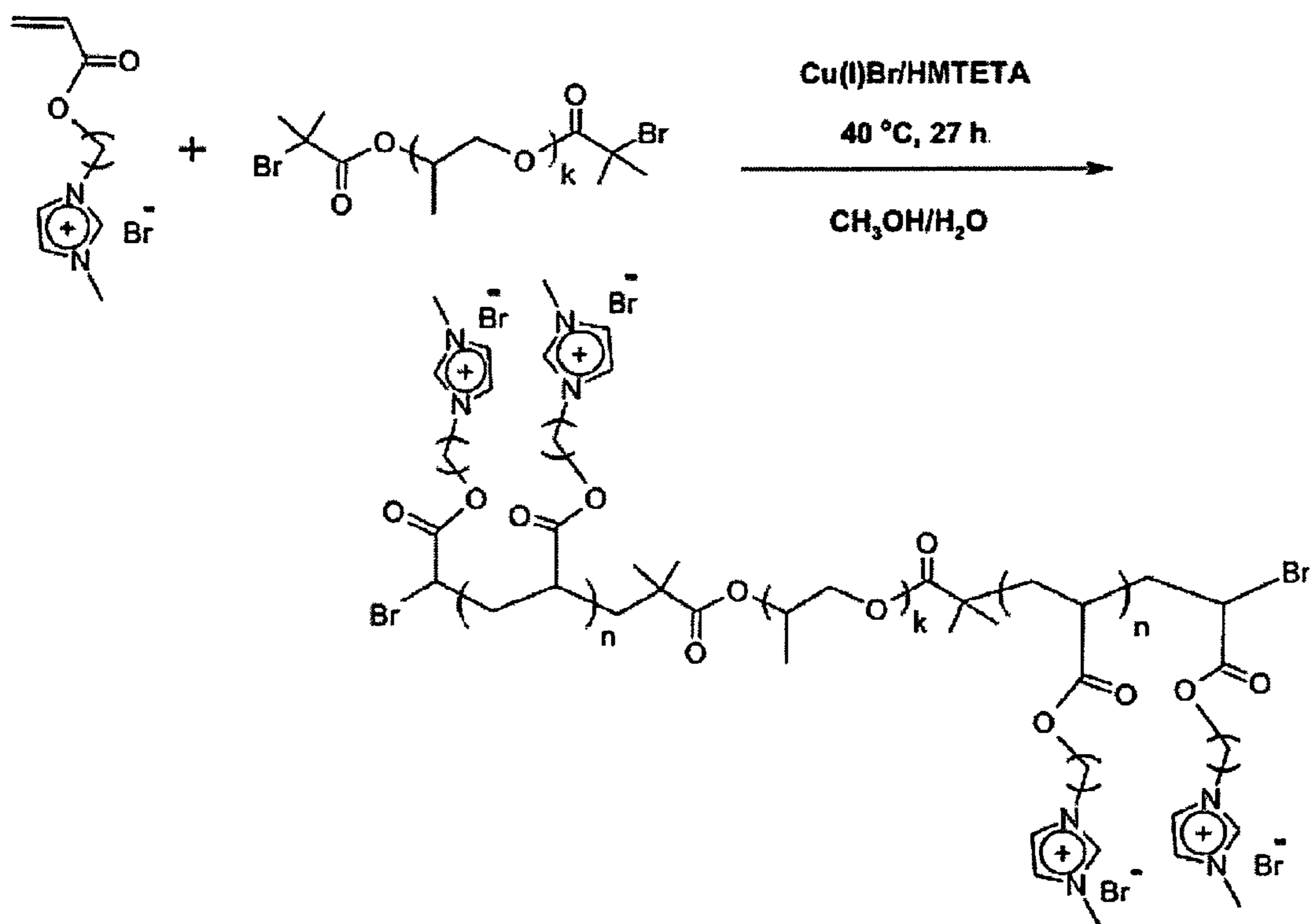
ATRP Reaction Scheme
