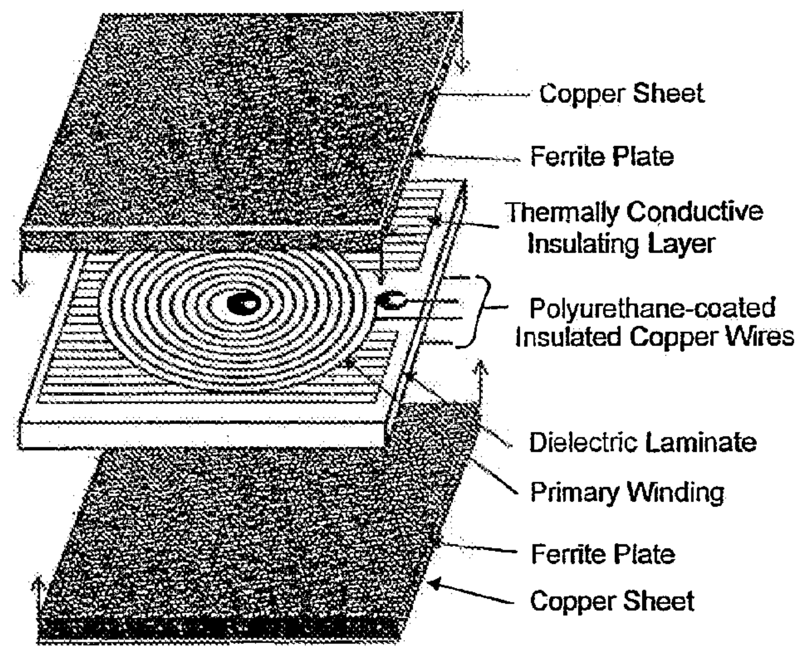
FIG.3 (PRIOR ART)
