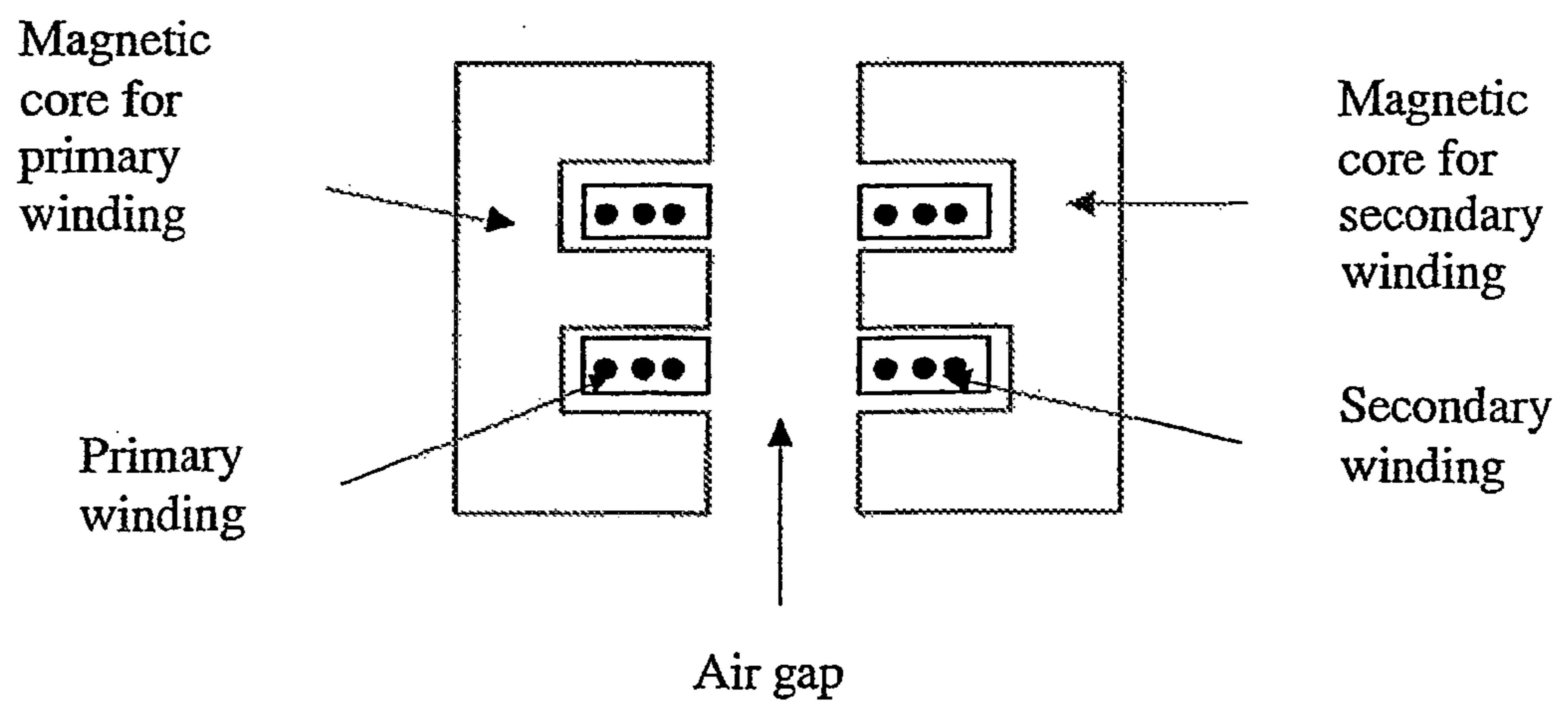
FIG.2 (PRIOR ART)
