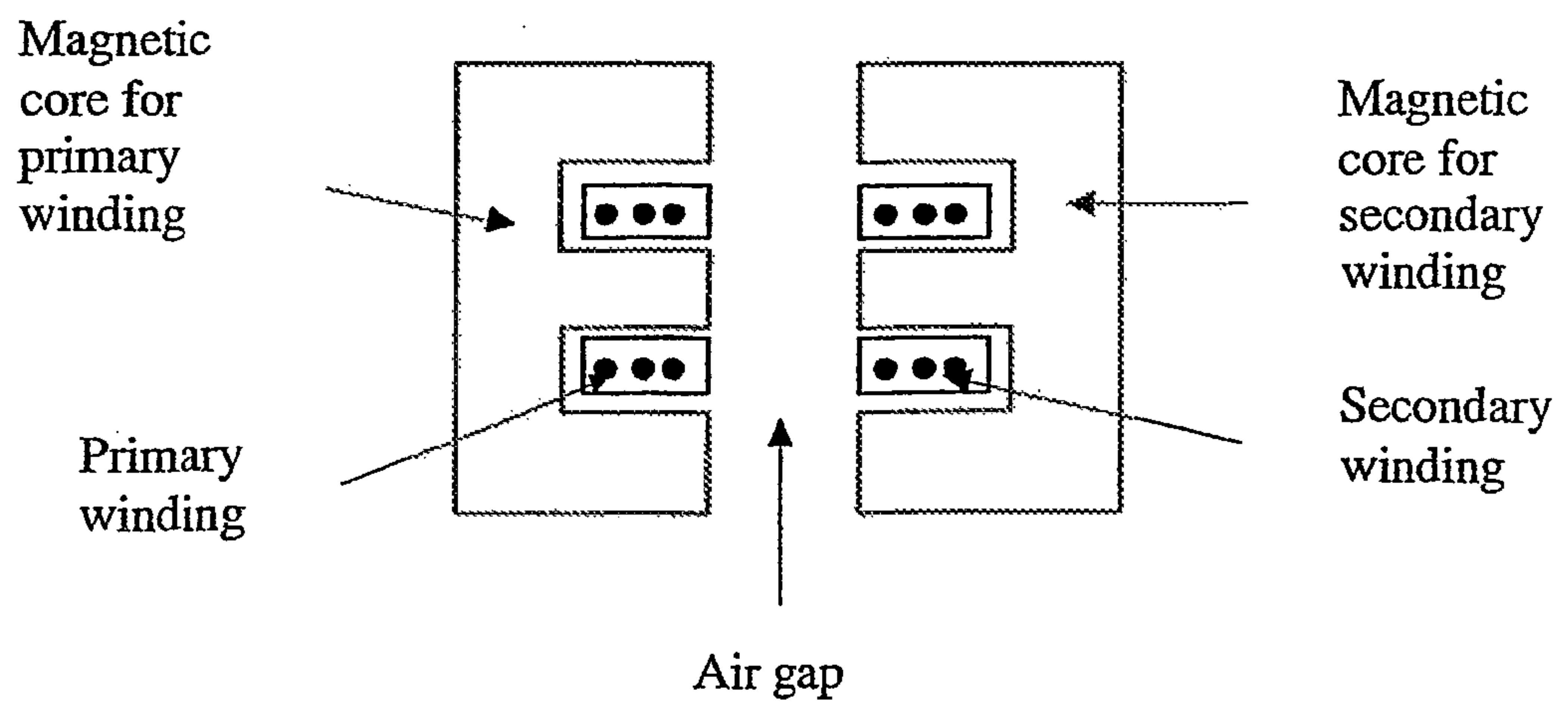
FIG.2 (PRIOR ART)
