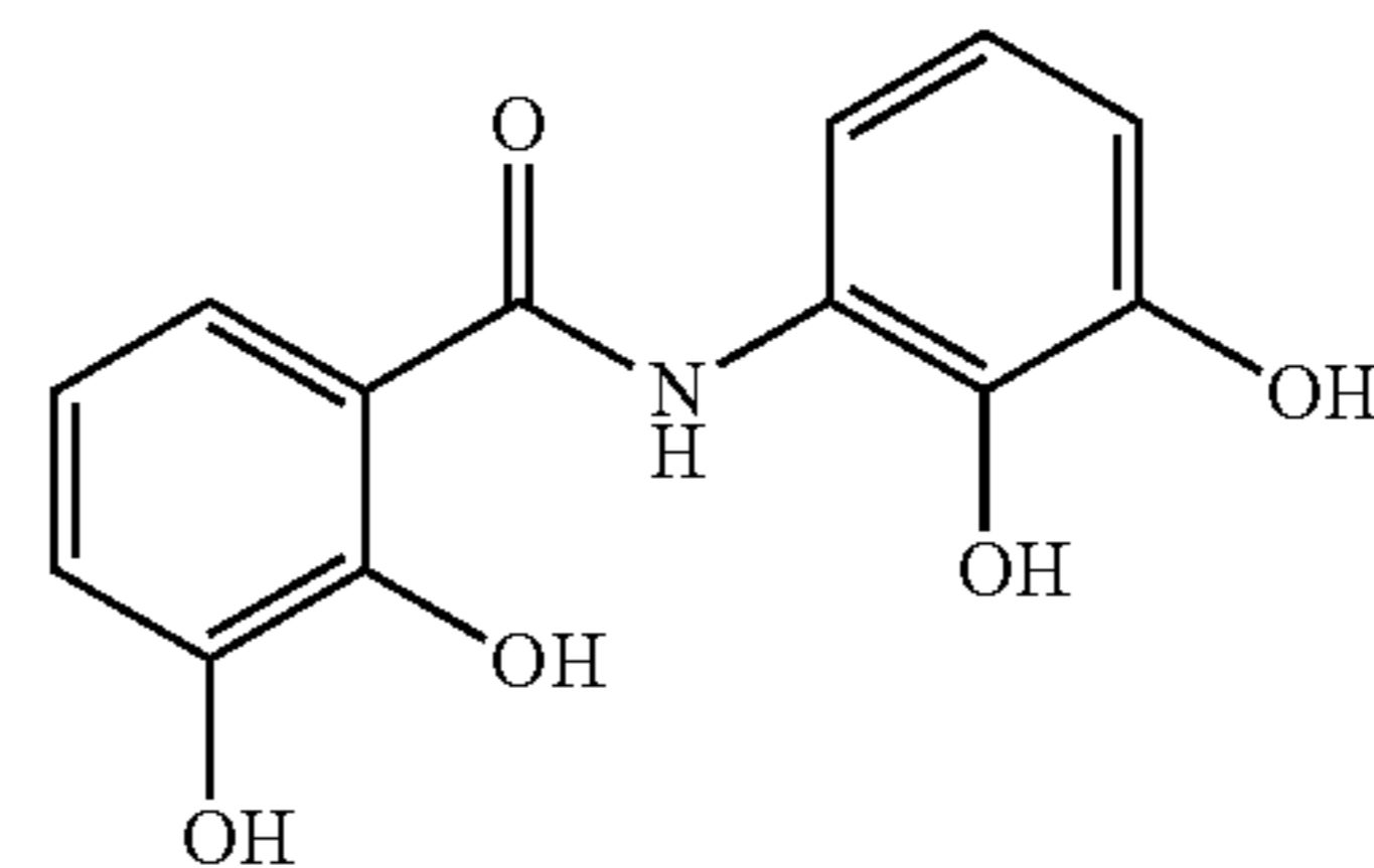
2,3 dihydroxybenzoic acid 2,3 dihydroxyanilide
