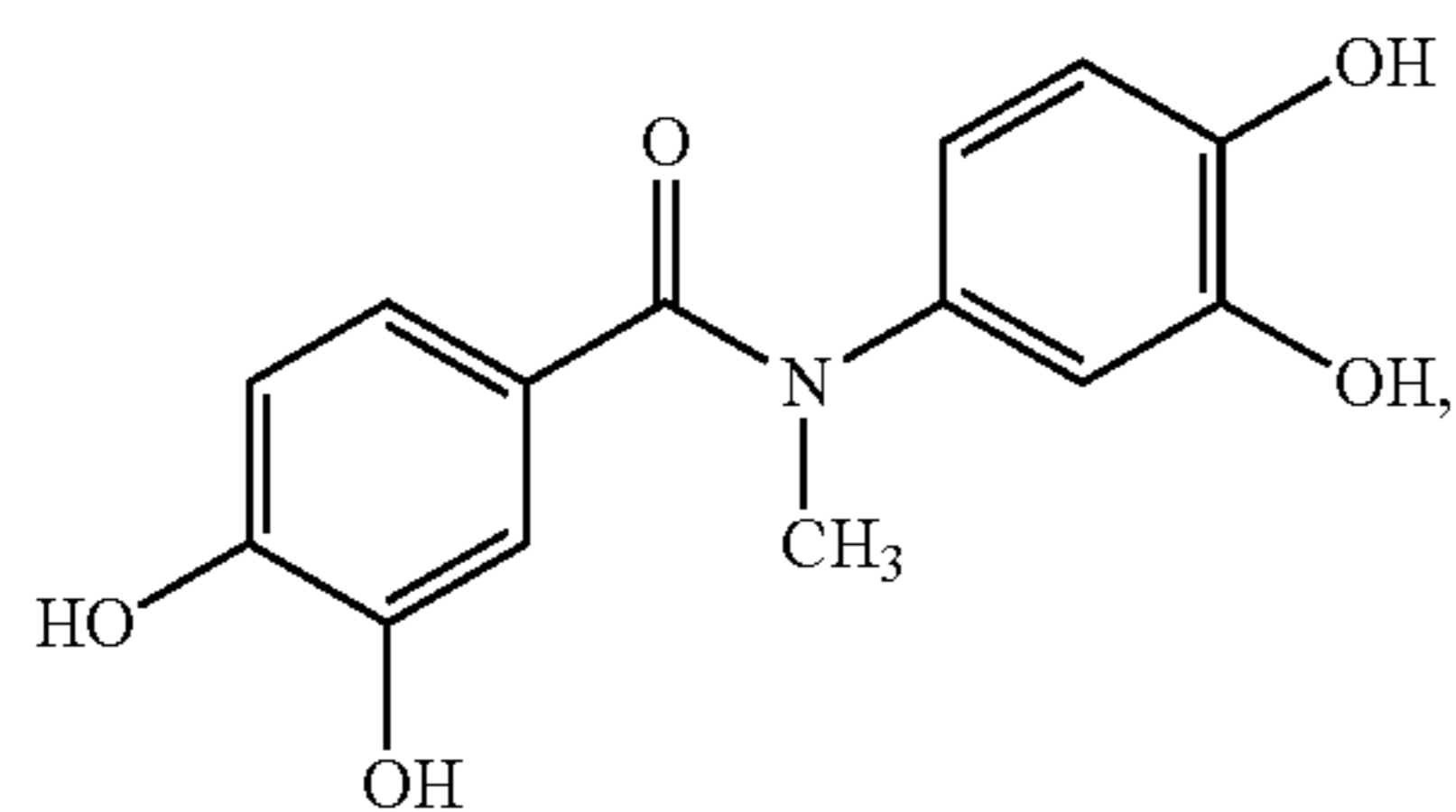
3,4 dihydroxybenzoic acid 3,4 dihydroxy N-methyl anilide
