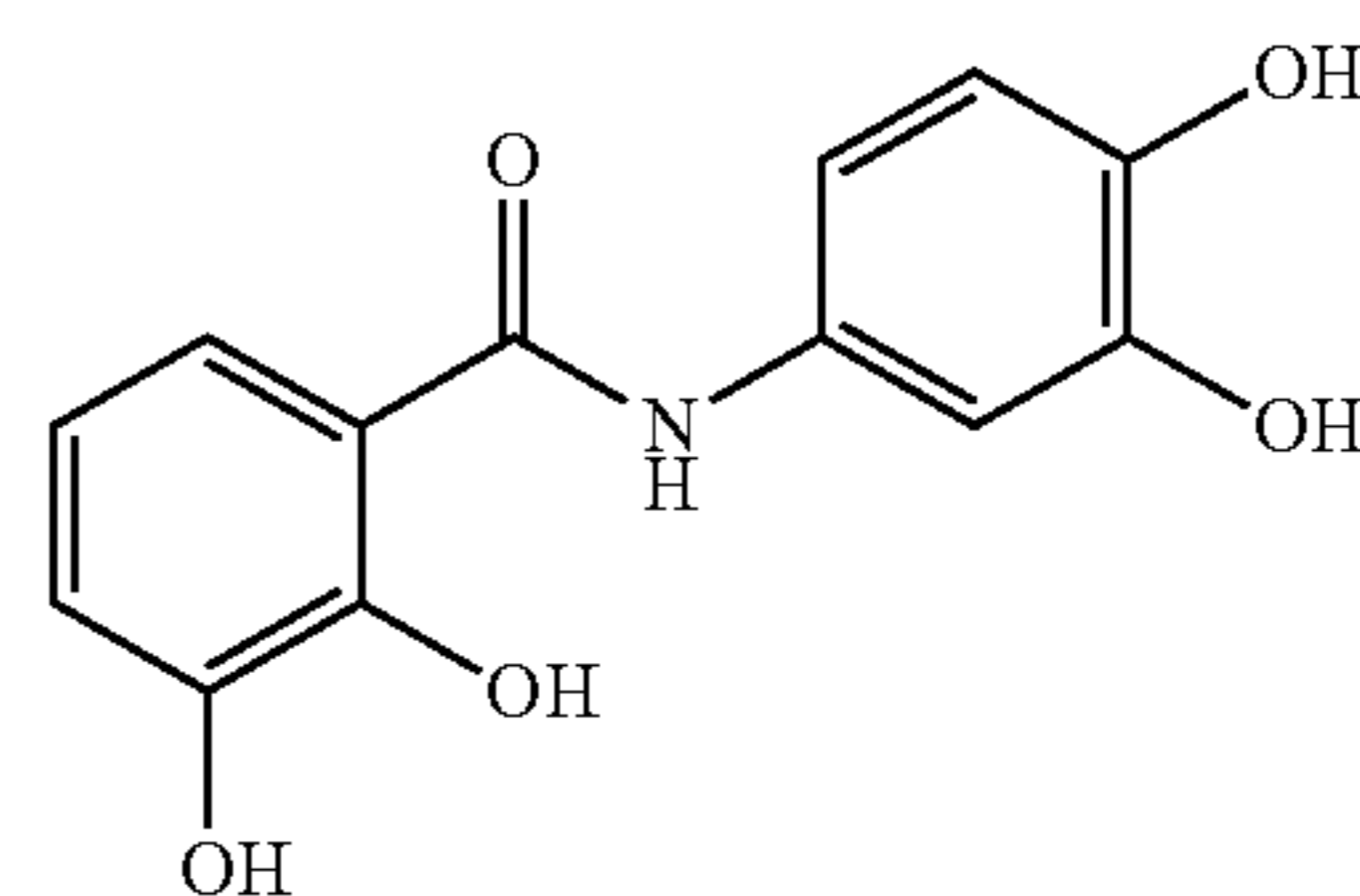
2,3 dihydroxybenzoic acid 3,4 dihydroxyanilide
