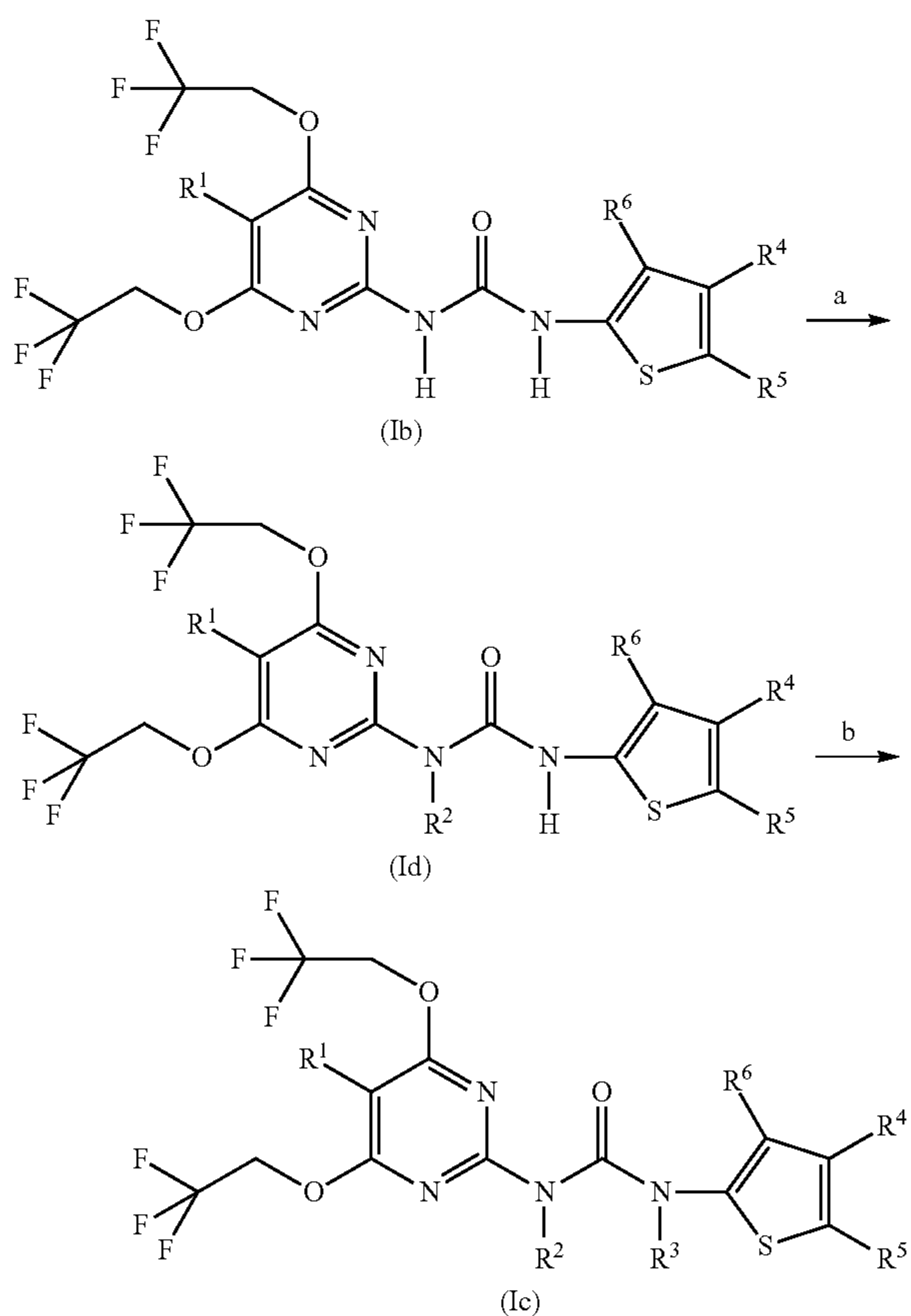
Scheme V
