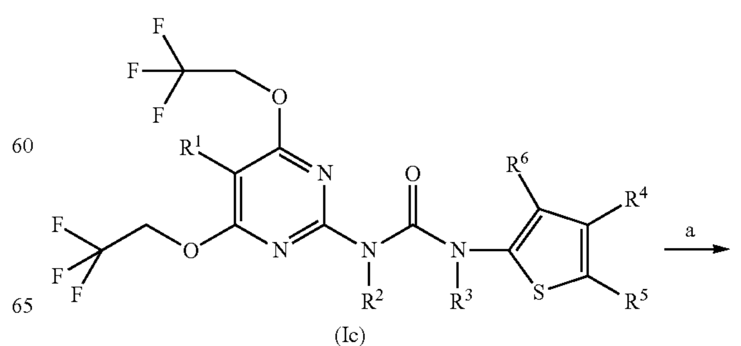
Scheme VII
