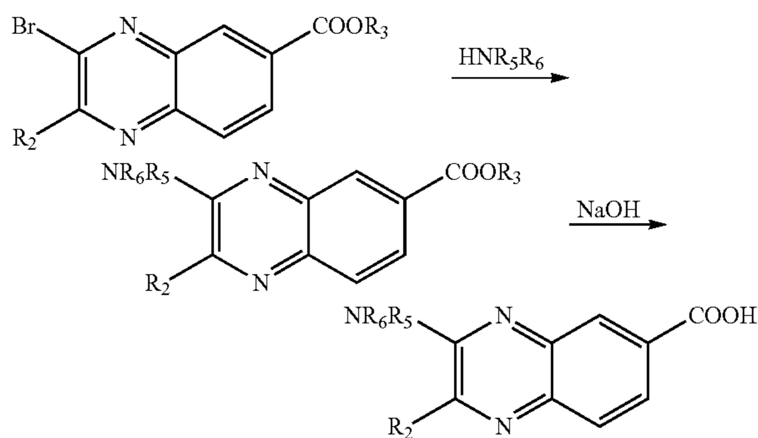
Scheme II
