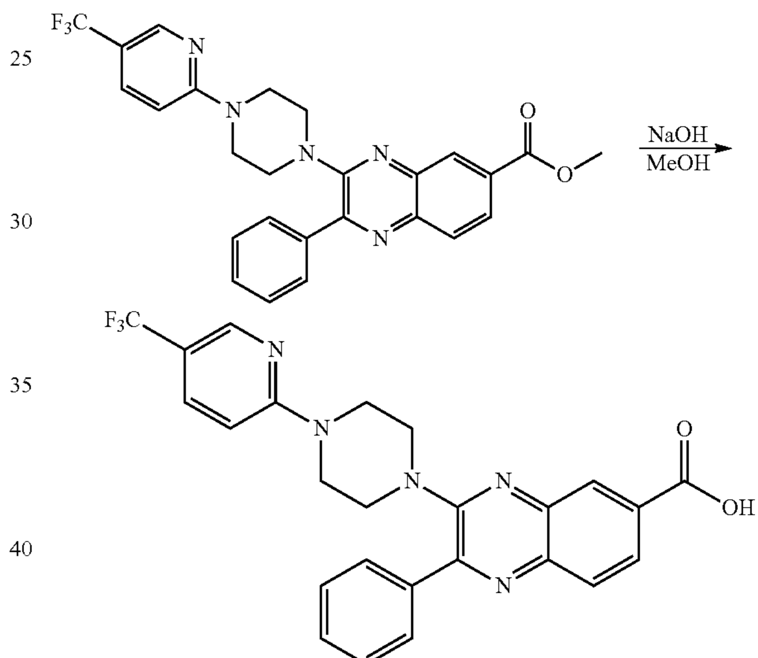
Step 1. Methyl 2-phenyl-3-(4-(5-(trifluoromethyl)pyridin-2-yl)piperazin-1-yl)quinoxaline-6-carboxylate
