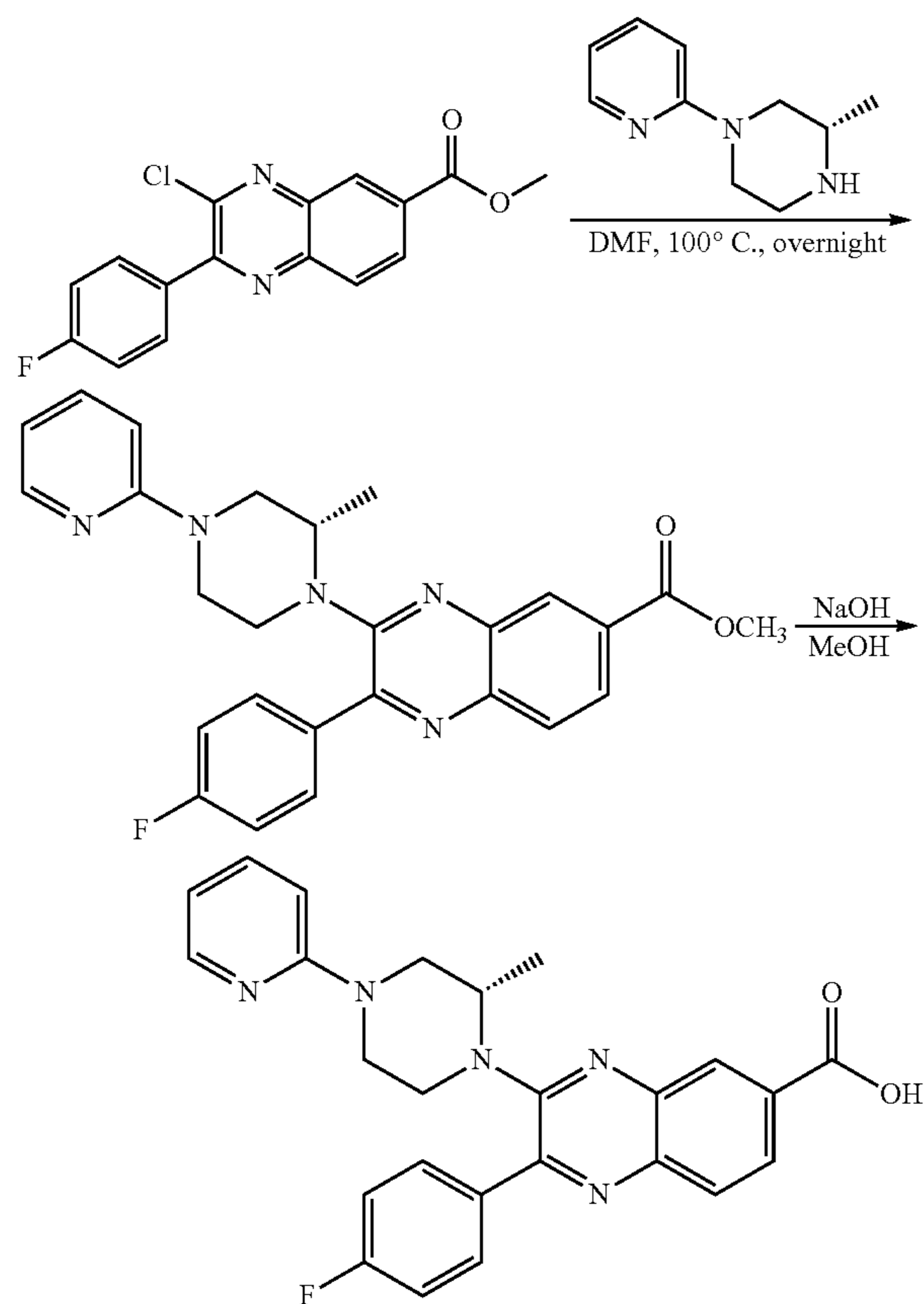
Scheme IV.
