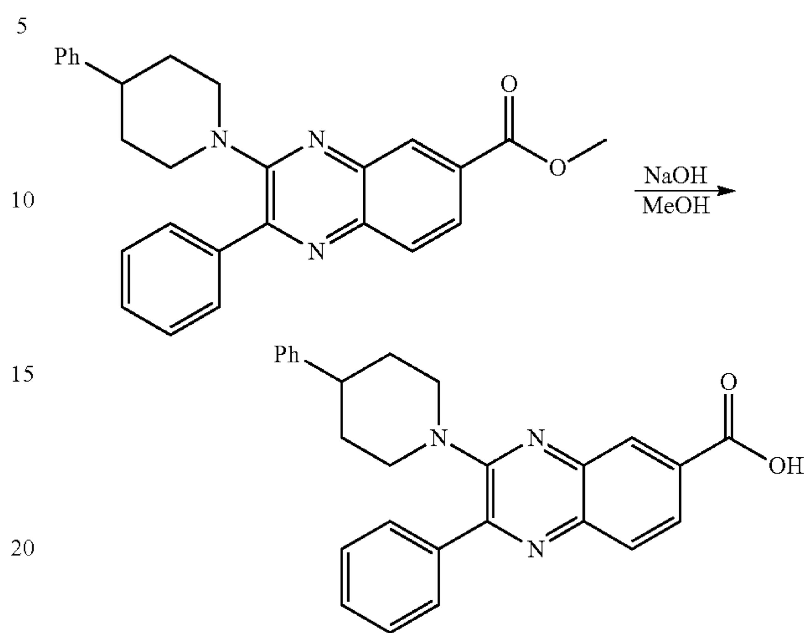
Step 2. 2-Phenyl-3-(4-phenylpiperidin-1-yl)quinoxaline-6-carboxylic acid
