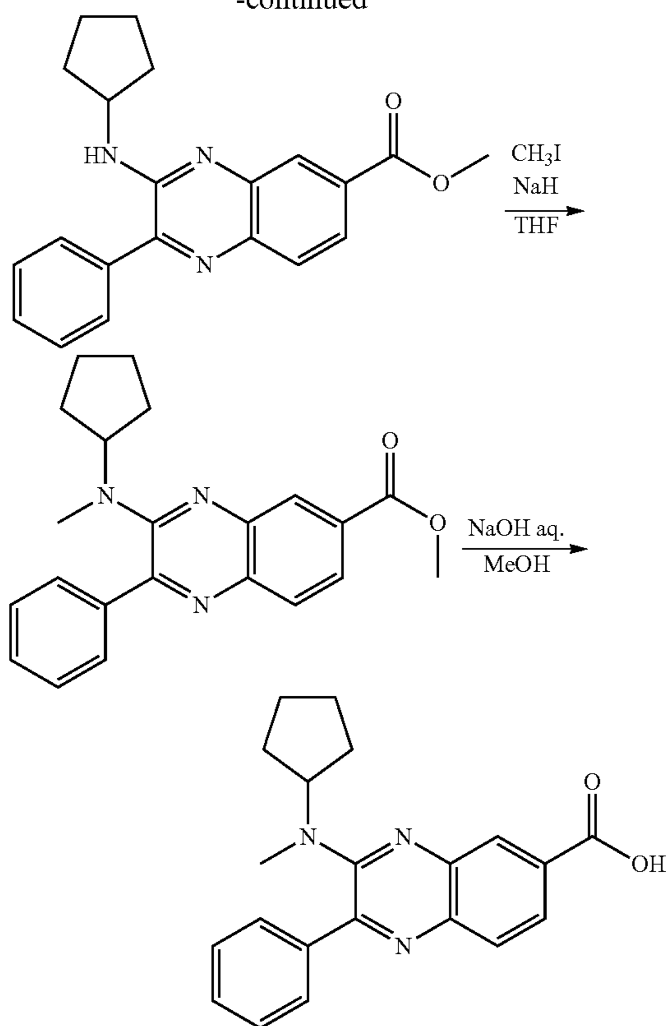
Step 1. Methyl 3-(cyclopentylamino)-2-phenylquinoxaline-6-carboxylate
