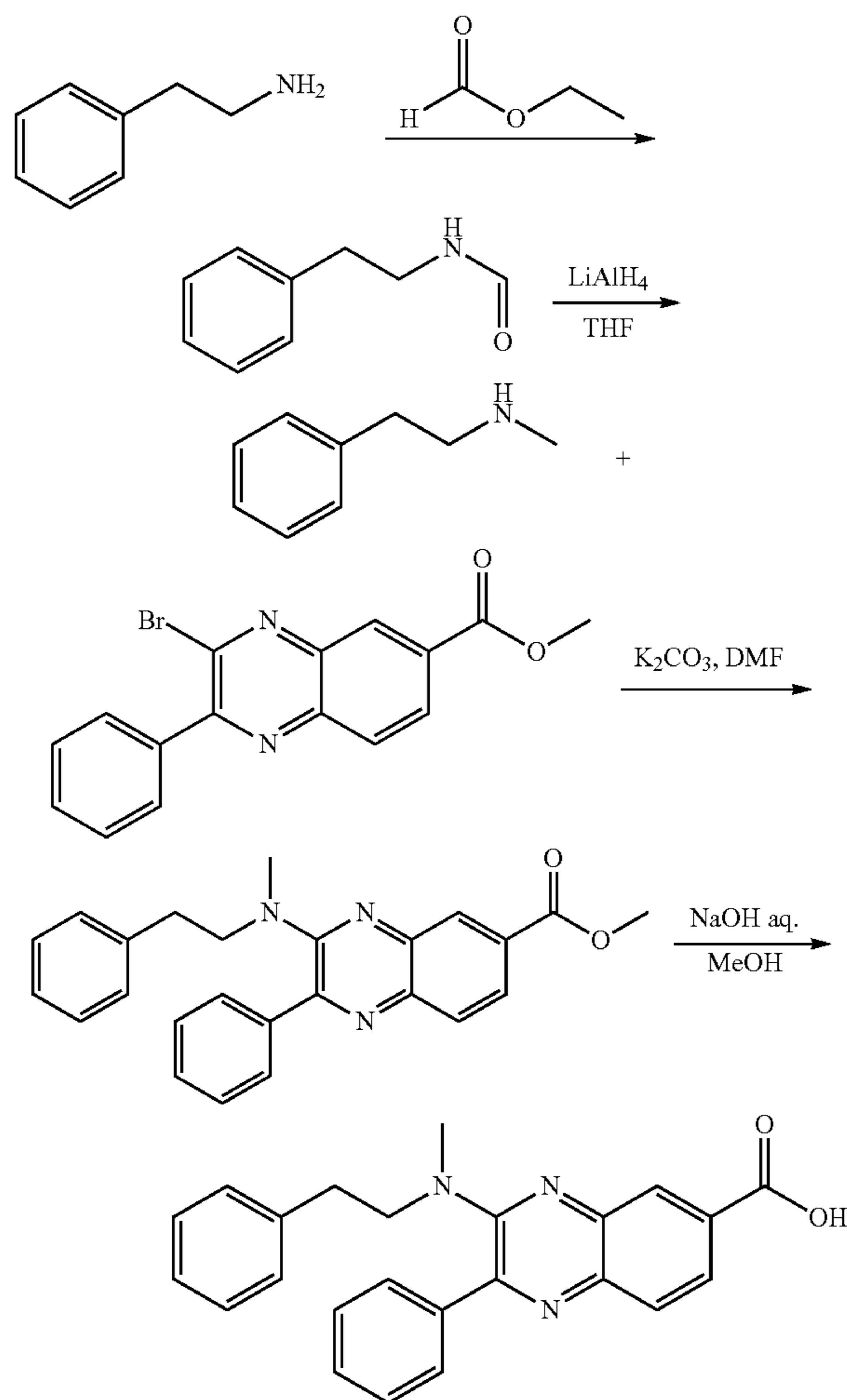
Step 1. N-Phenethylformamide
