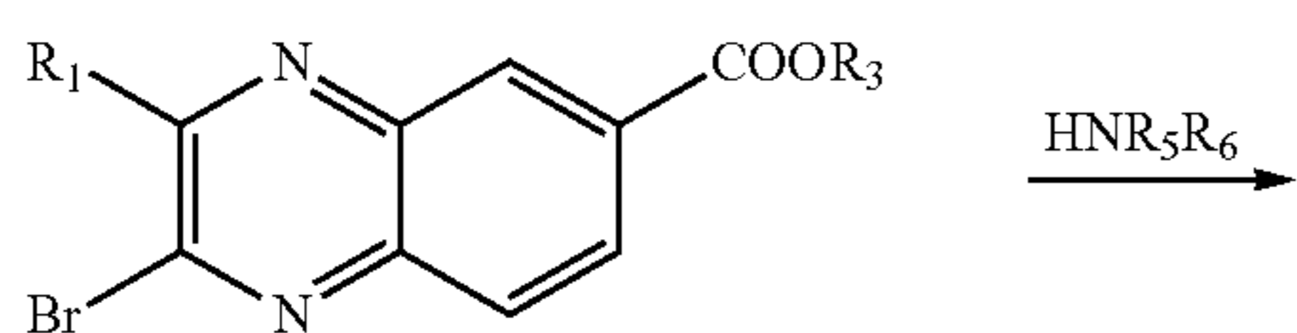
Scheme III
