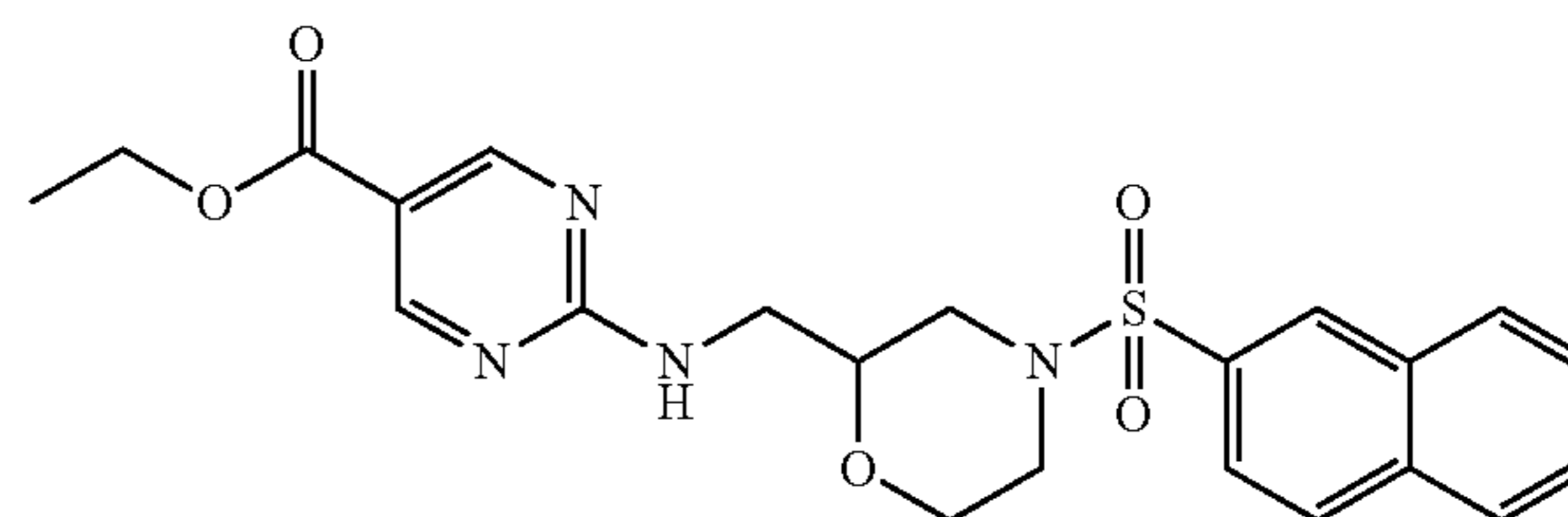
intermediate 29
