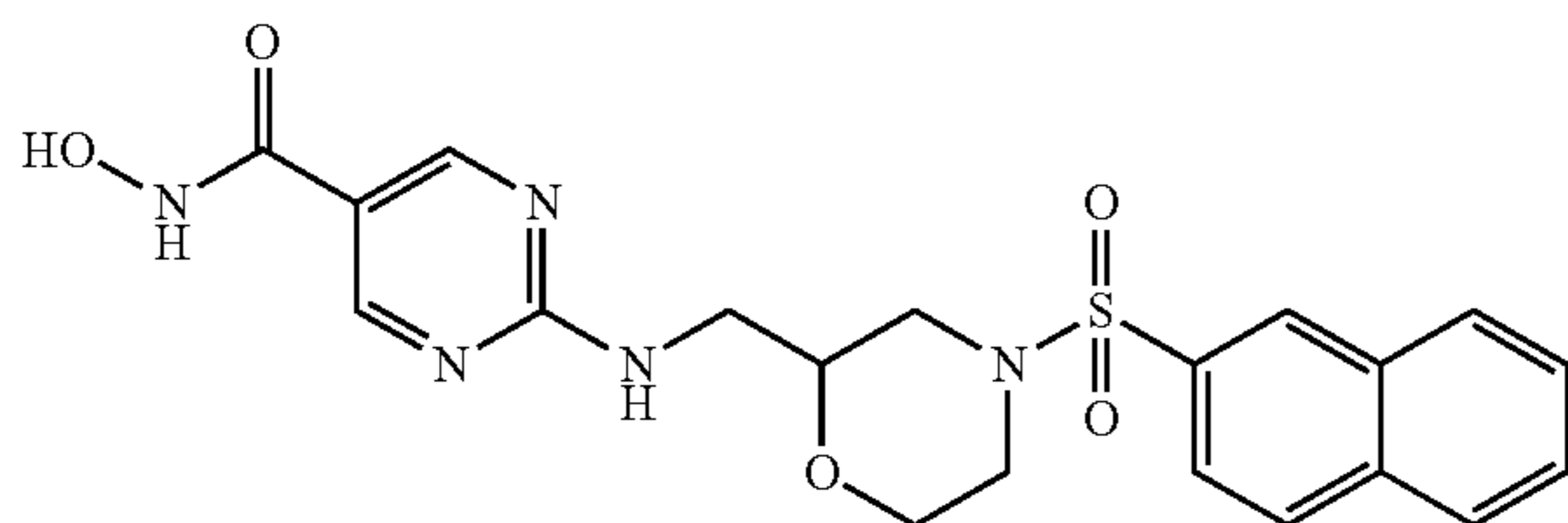
compound 9
