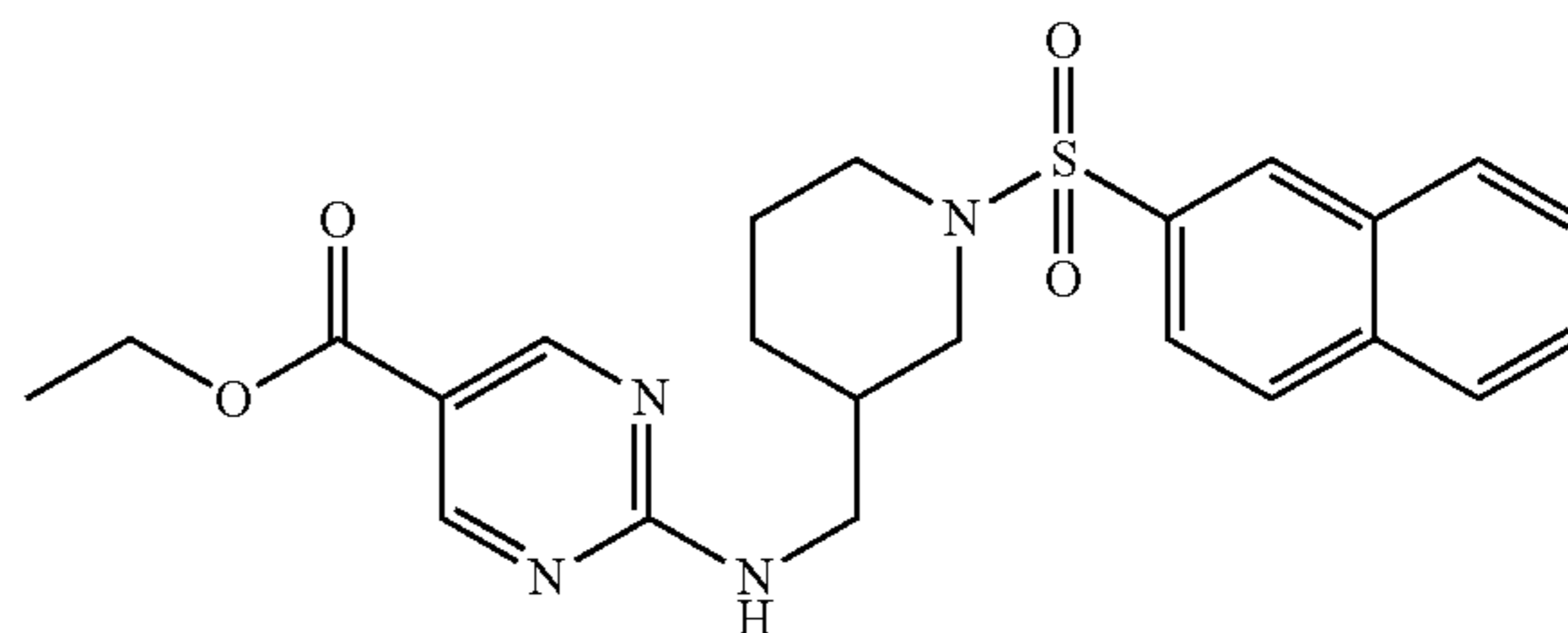
compound 6
