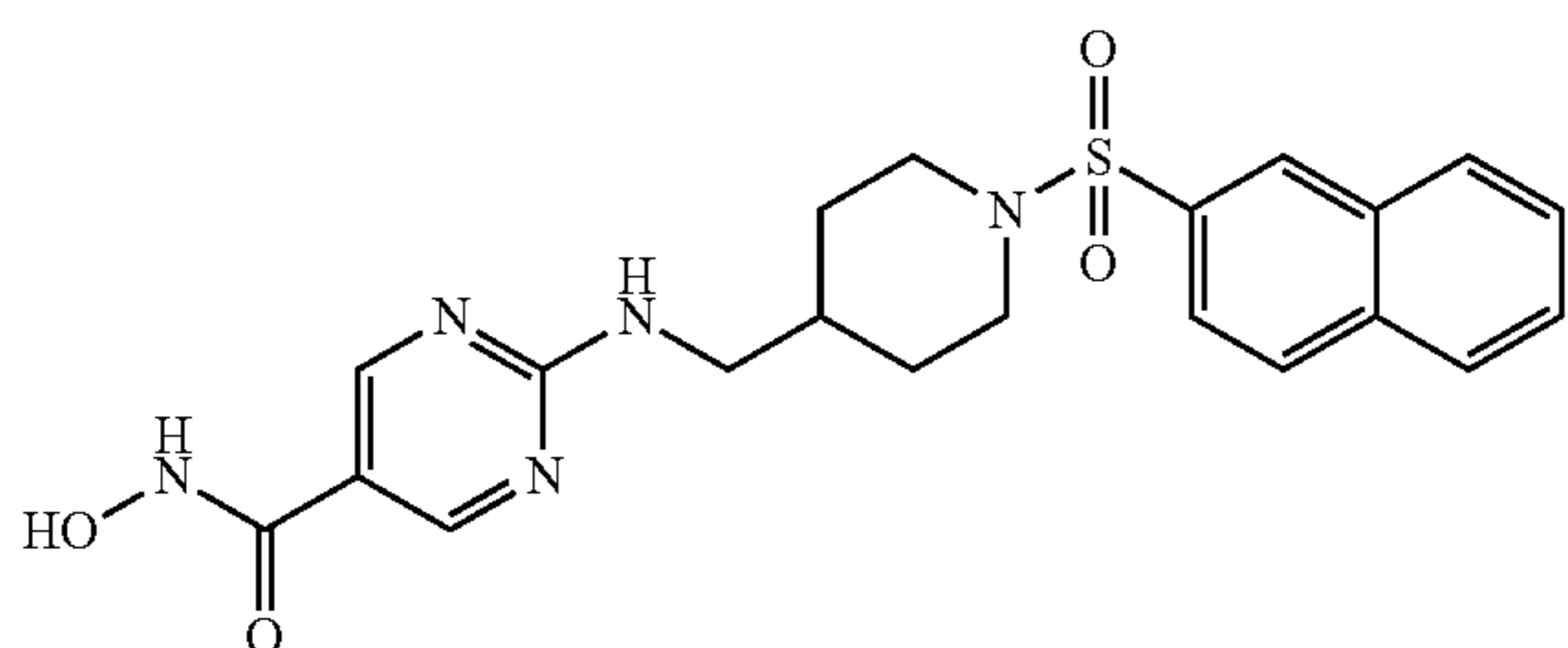
compound 7
