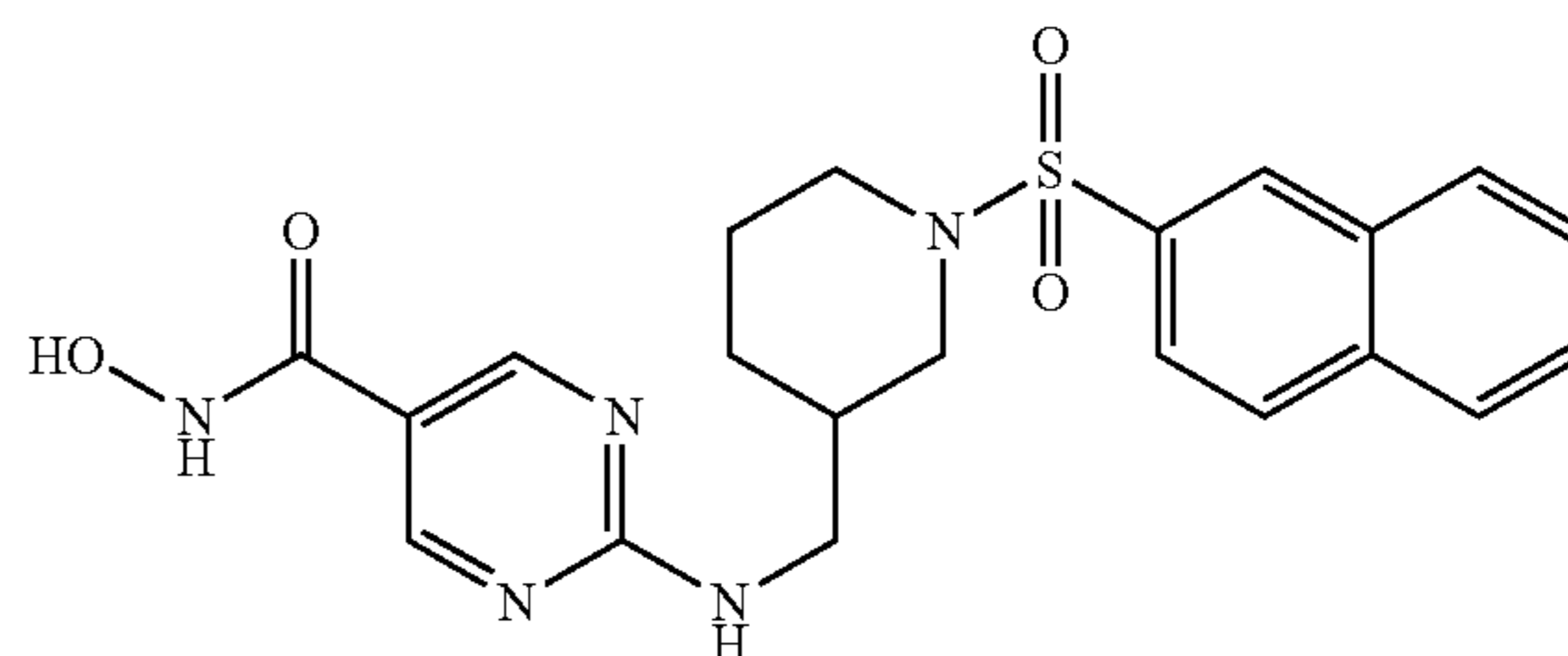
compound 8
