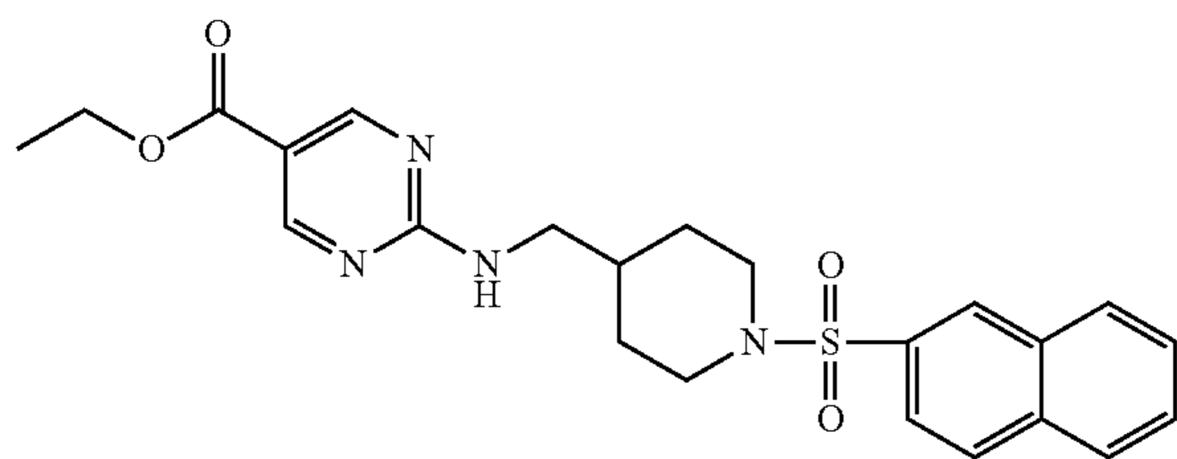
intermediate 28
