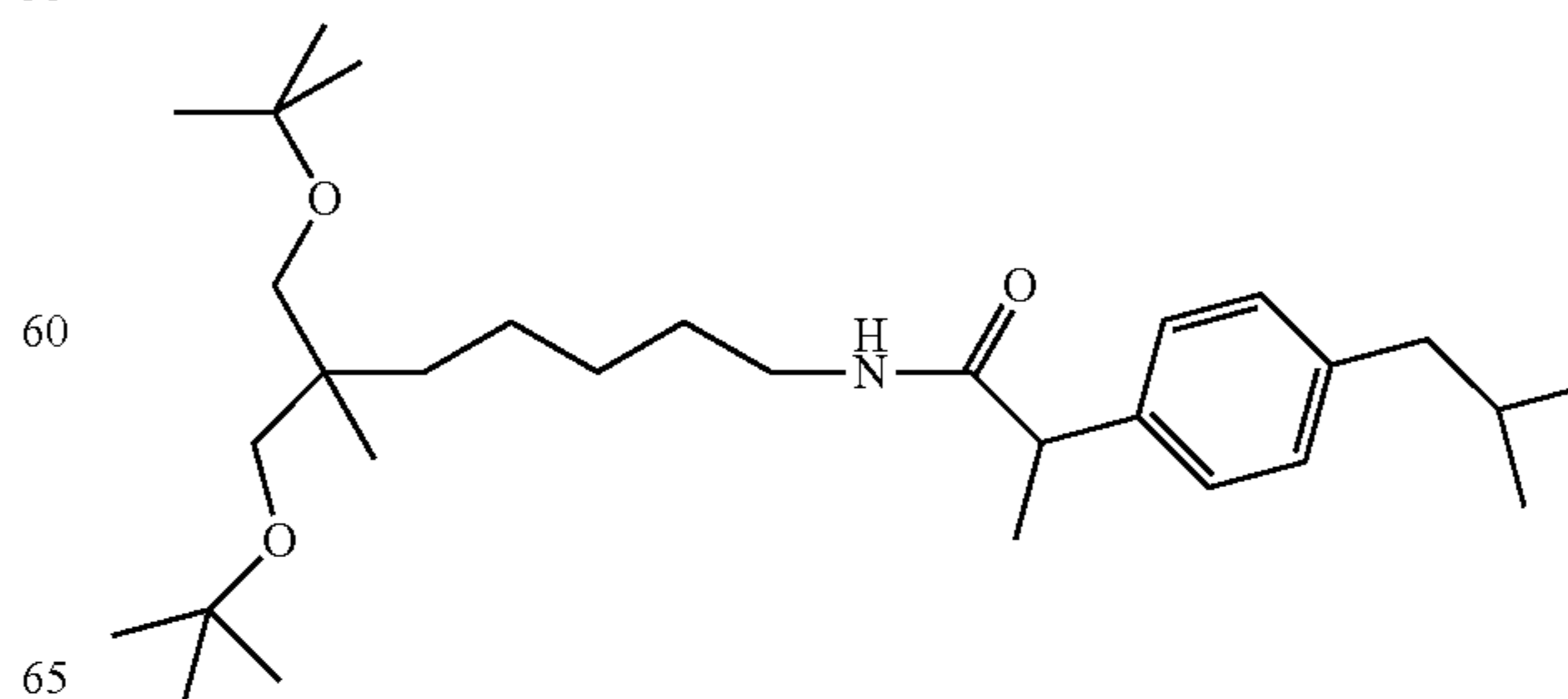
Formula (V')
