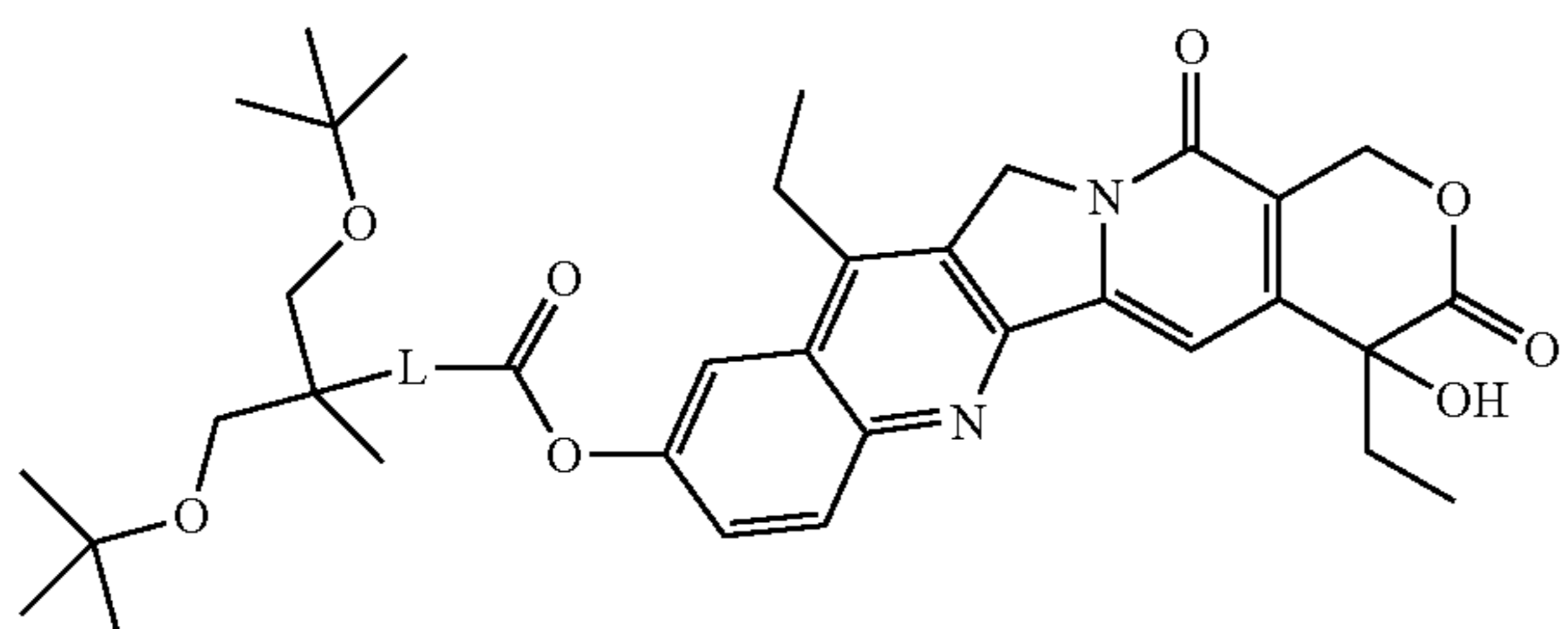
Formula (VI)
