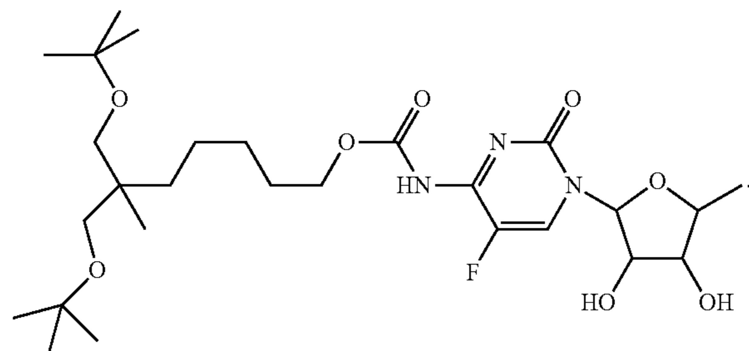
Formula (VIII)
