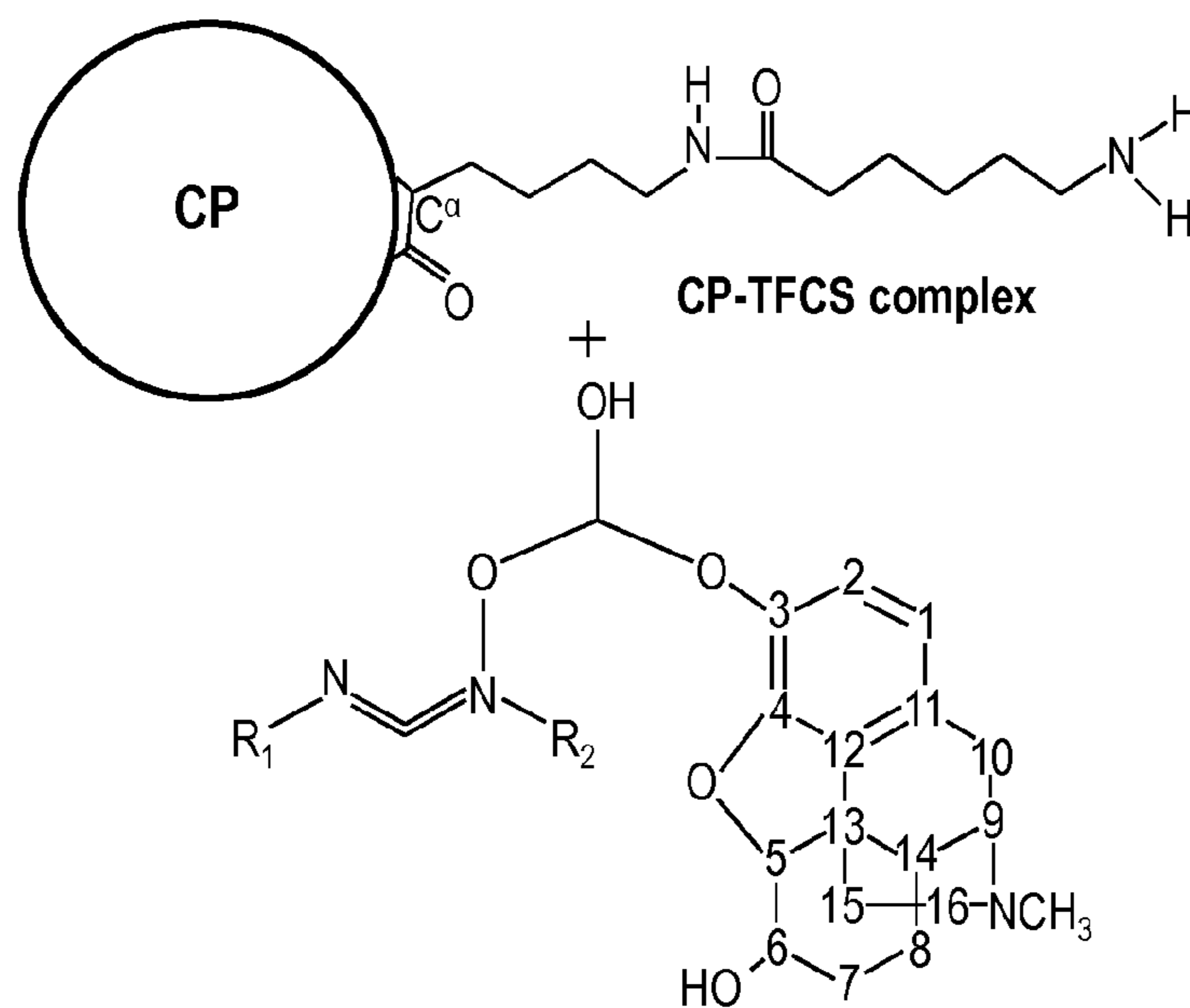
Intermediate EDC-(3-O-Carboxymethylmorphine)
