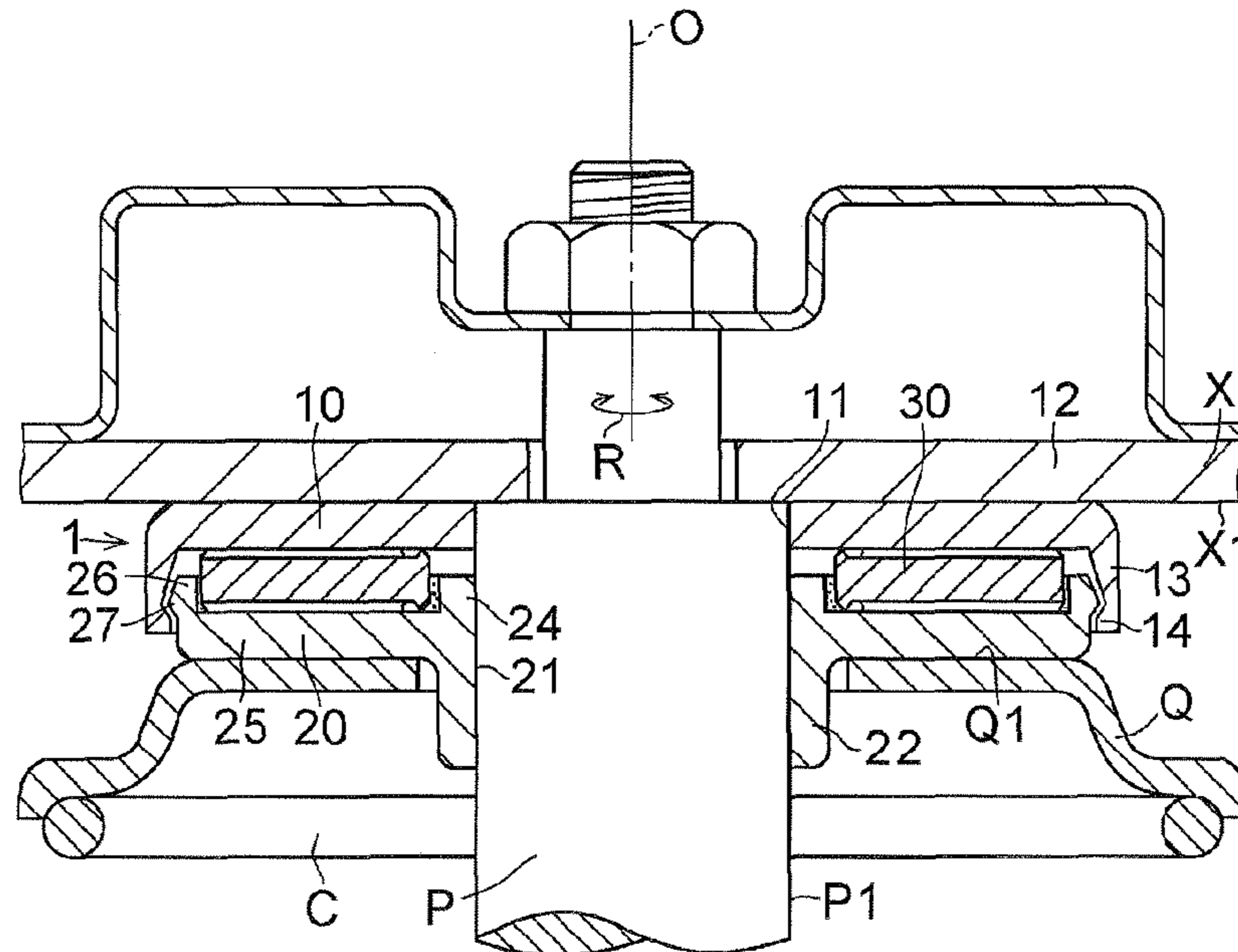
FIG. 15 (PRIOR ART)
