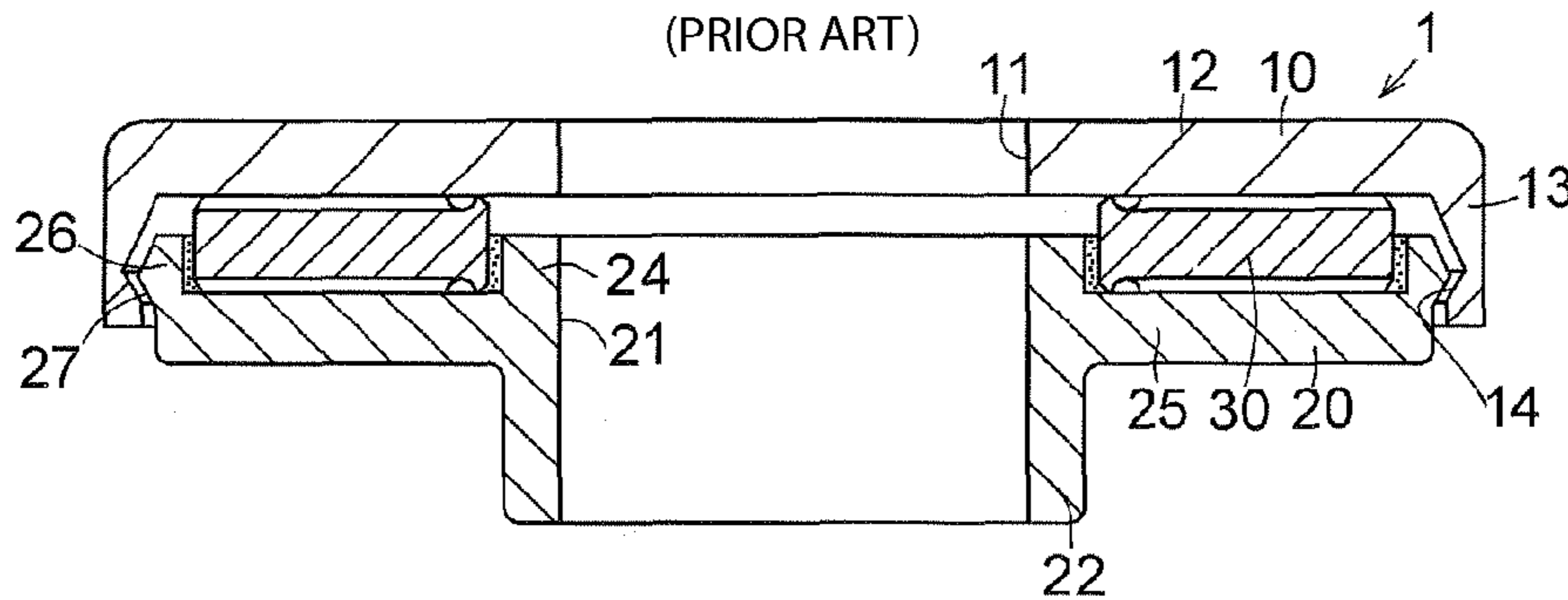
FIG. 15 (PRIOR ART)
