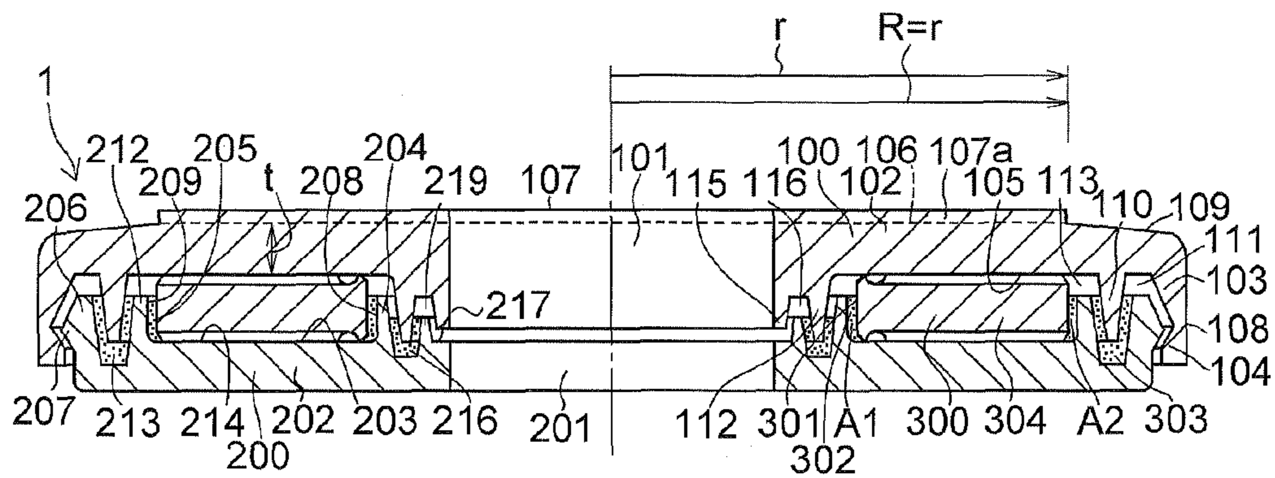
FIG. 14 (PRIOR ART)
