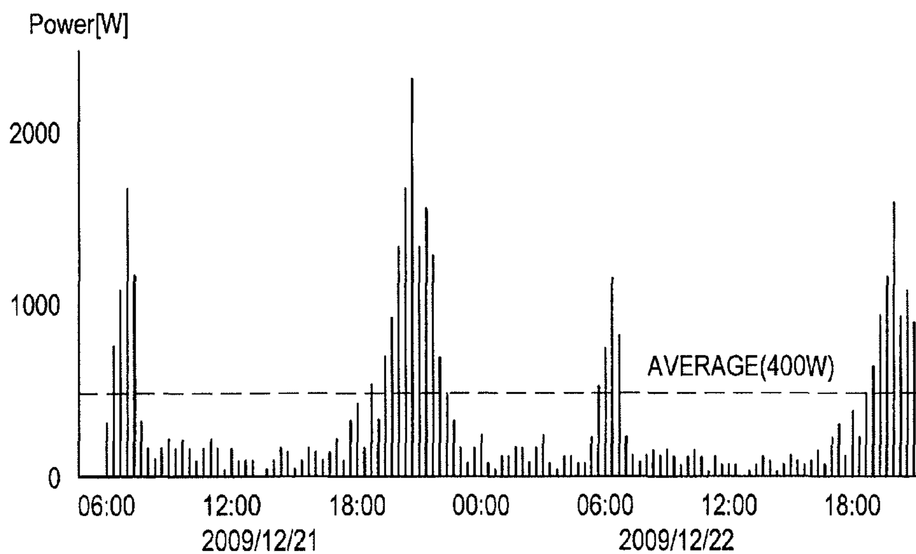
(B) EXAMPLE OF POWER CONSUMPTION PATTERN
