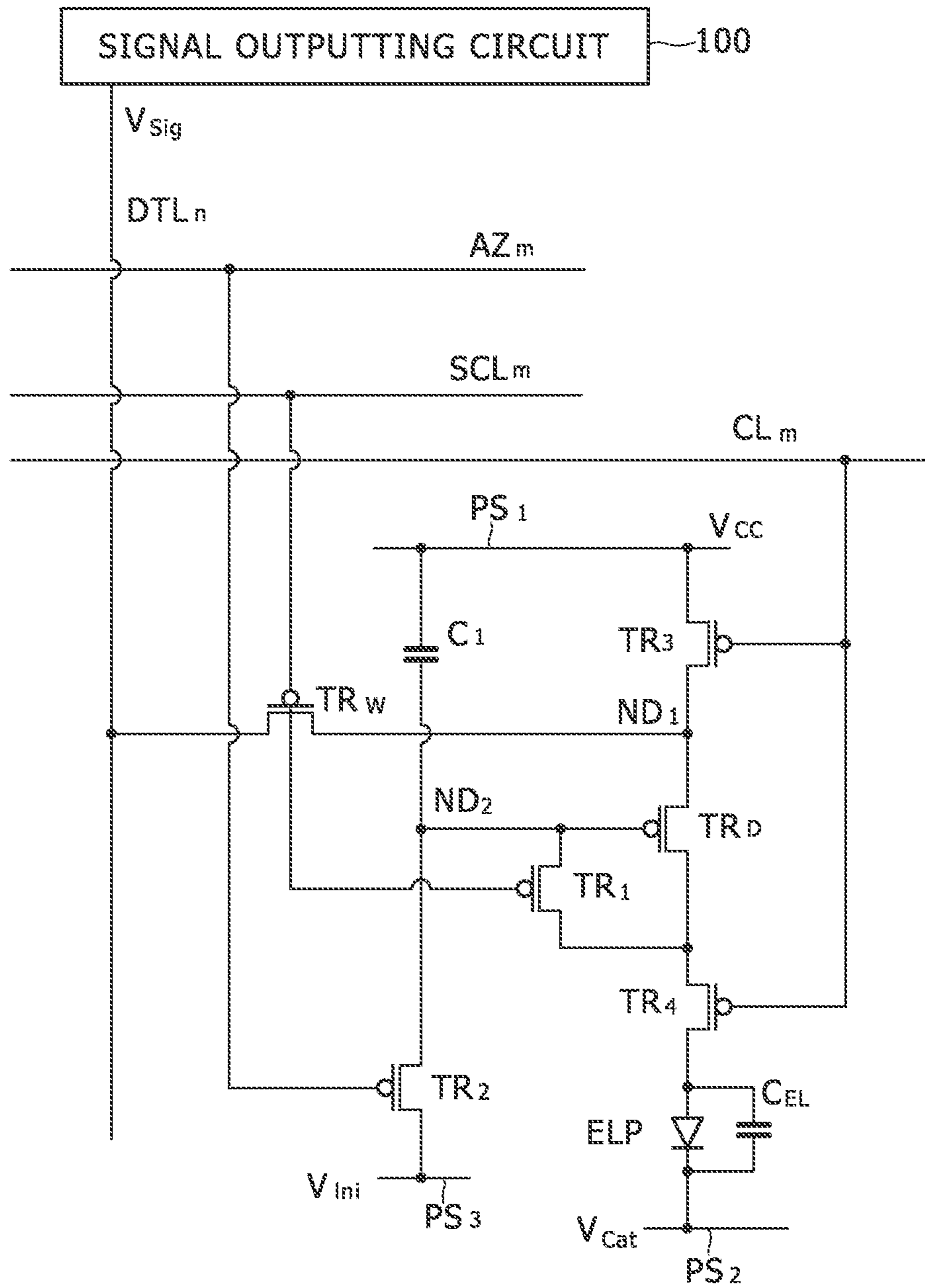
FIG. 19 (Related Art)
