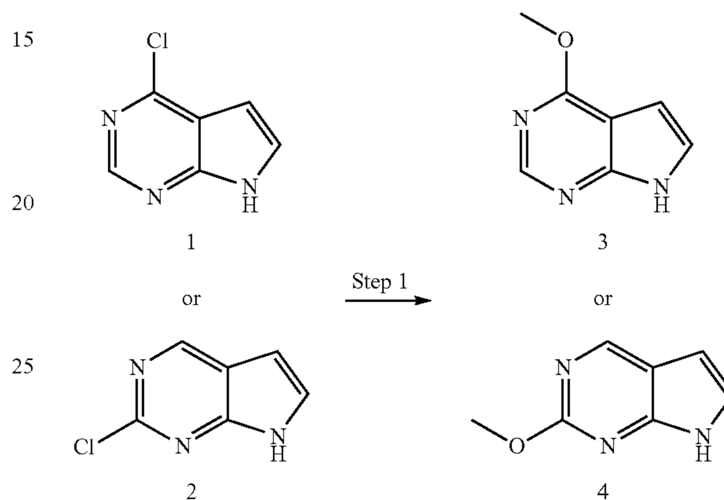
Scheme I
