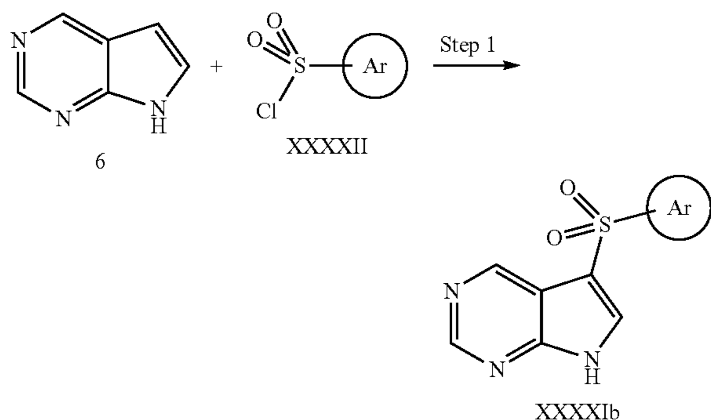
Scheme XXI
