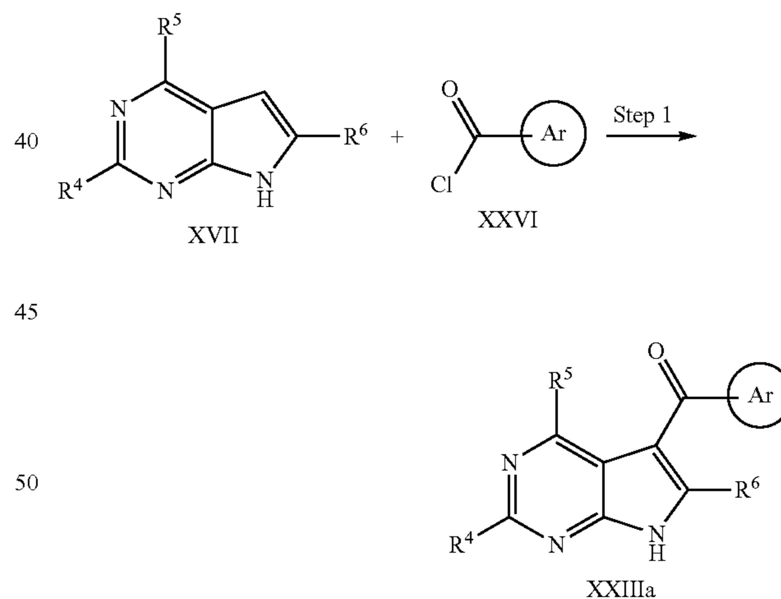
Scheme XIII
