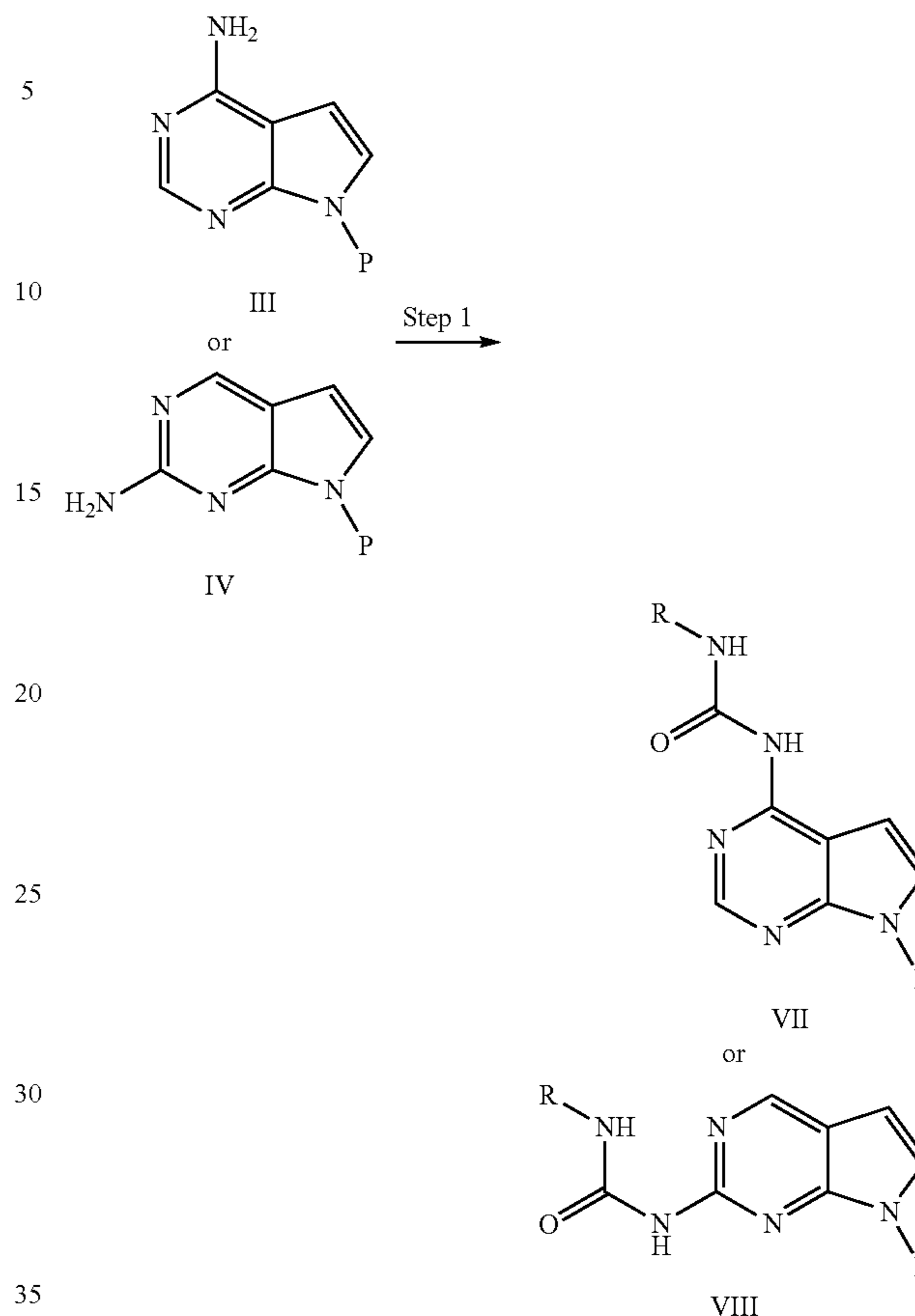
Scheme IV
