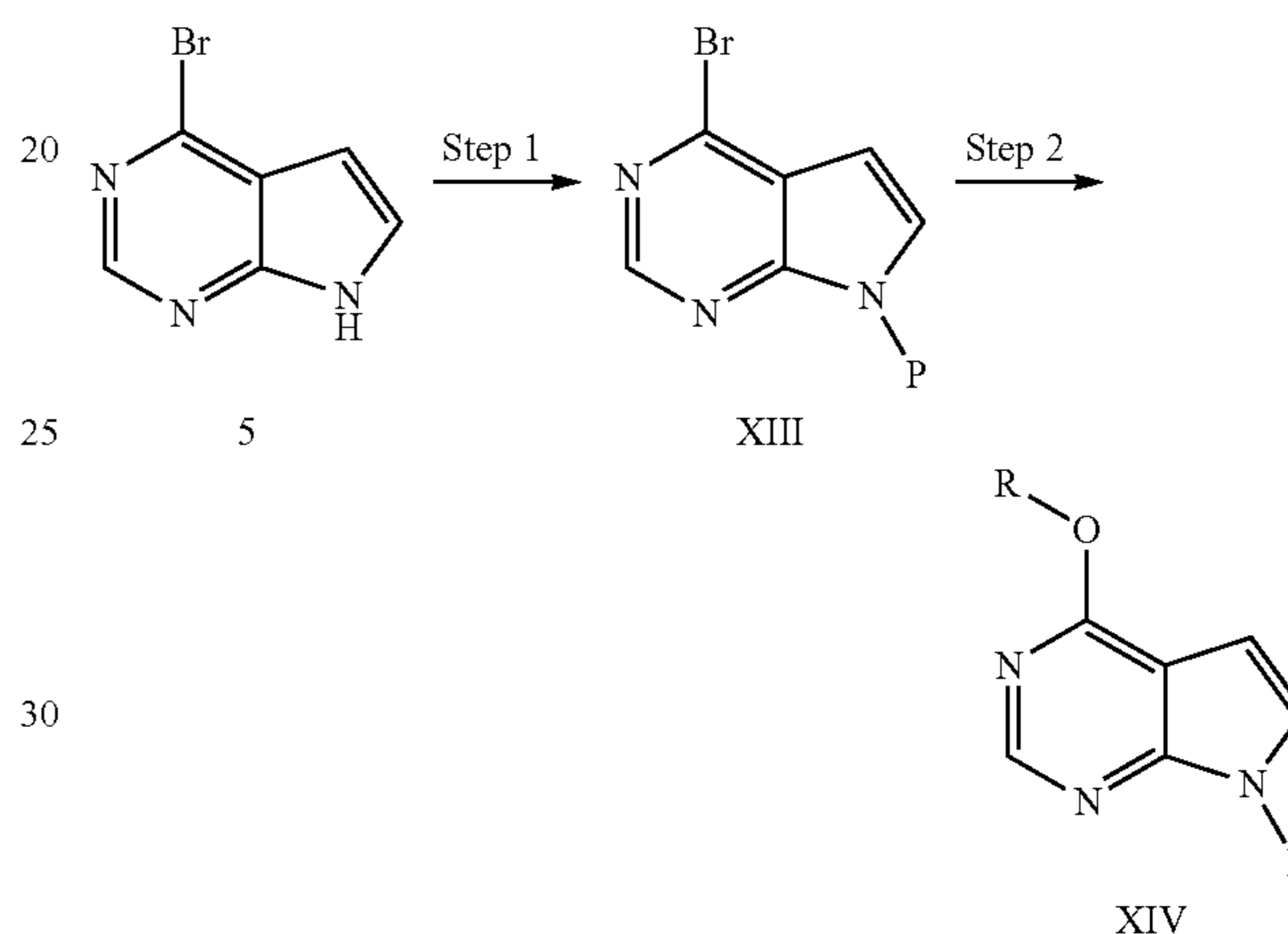
Scheme VII
