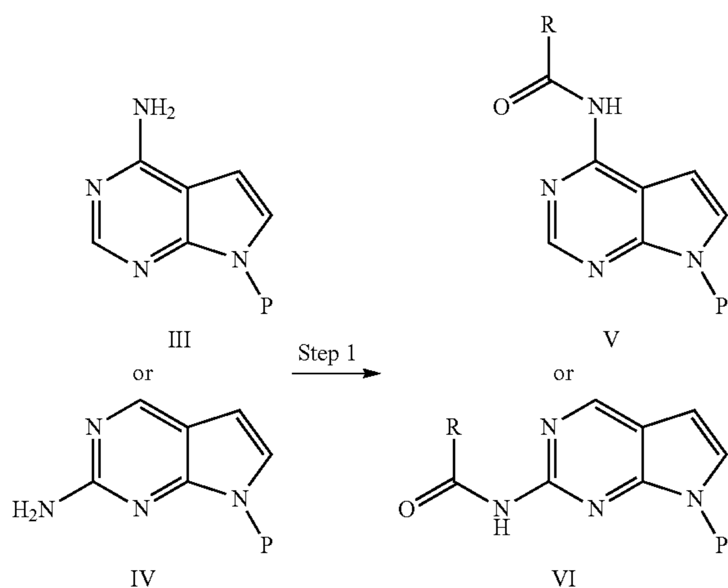
Scheme III
