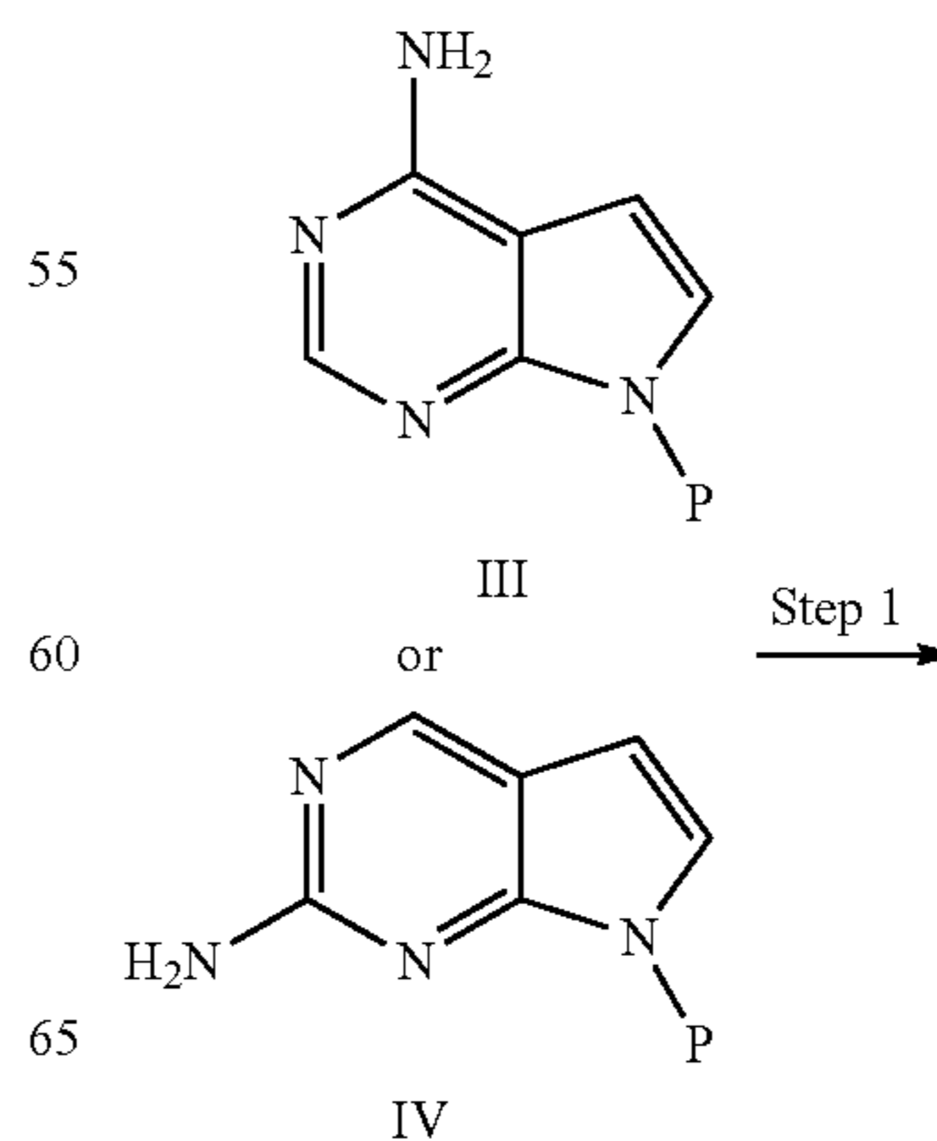
Scheme V
