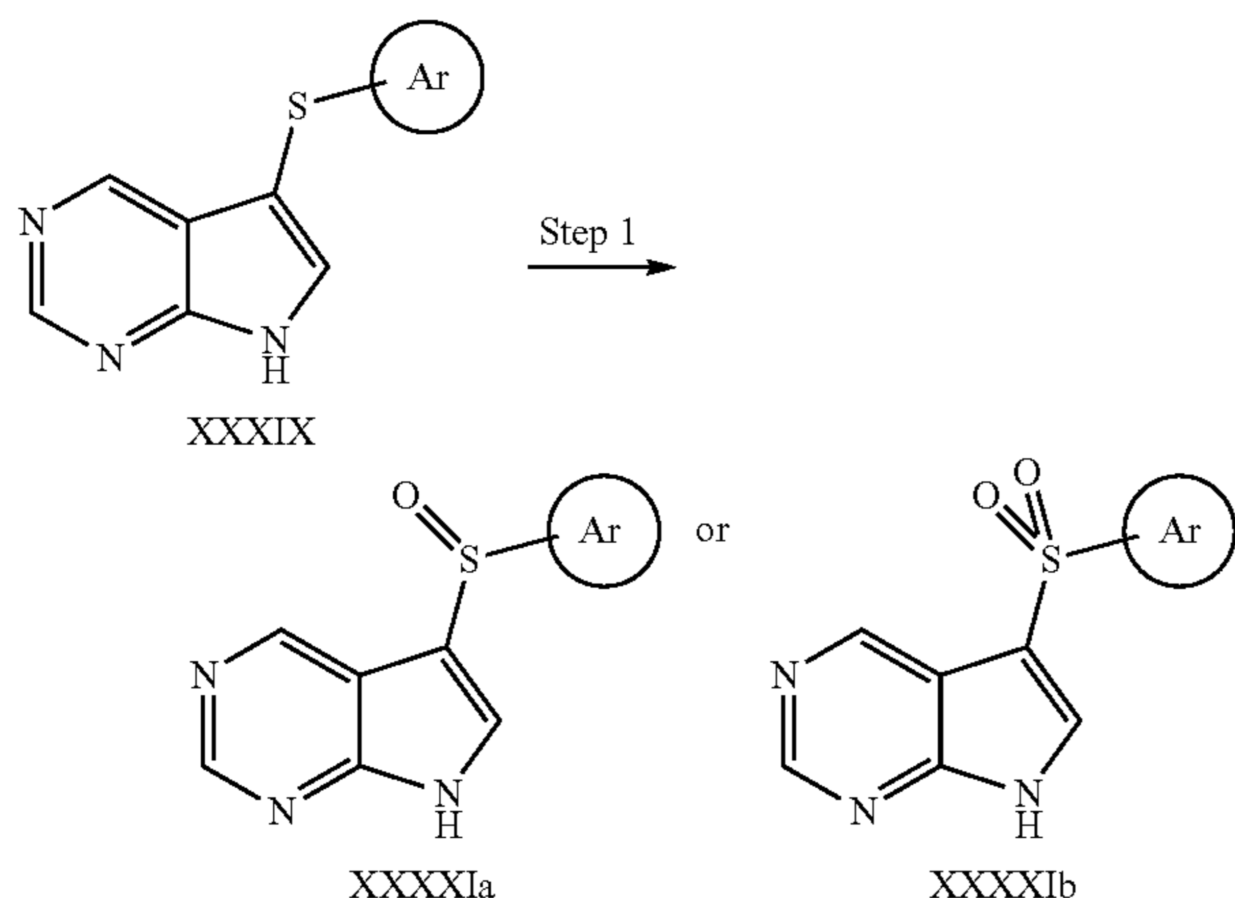
Scheme XX
