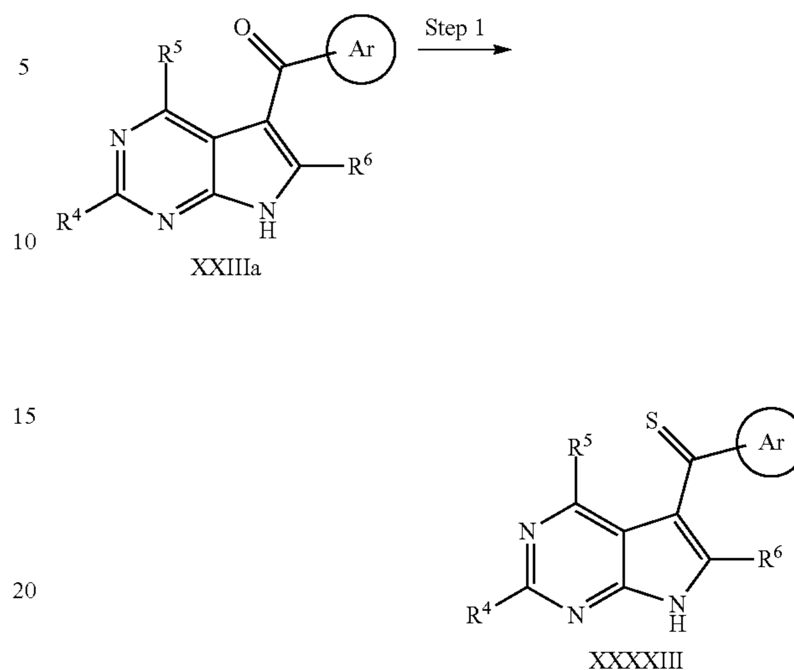
Scheme XXII
