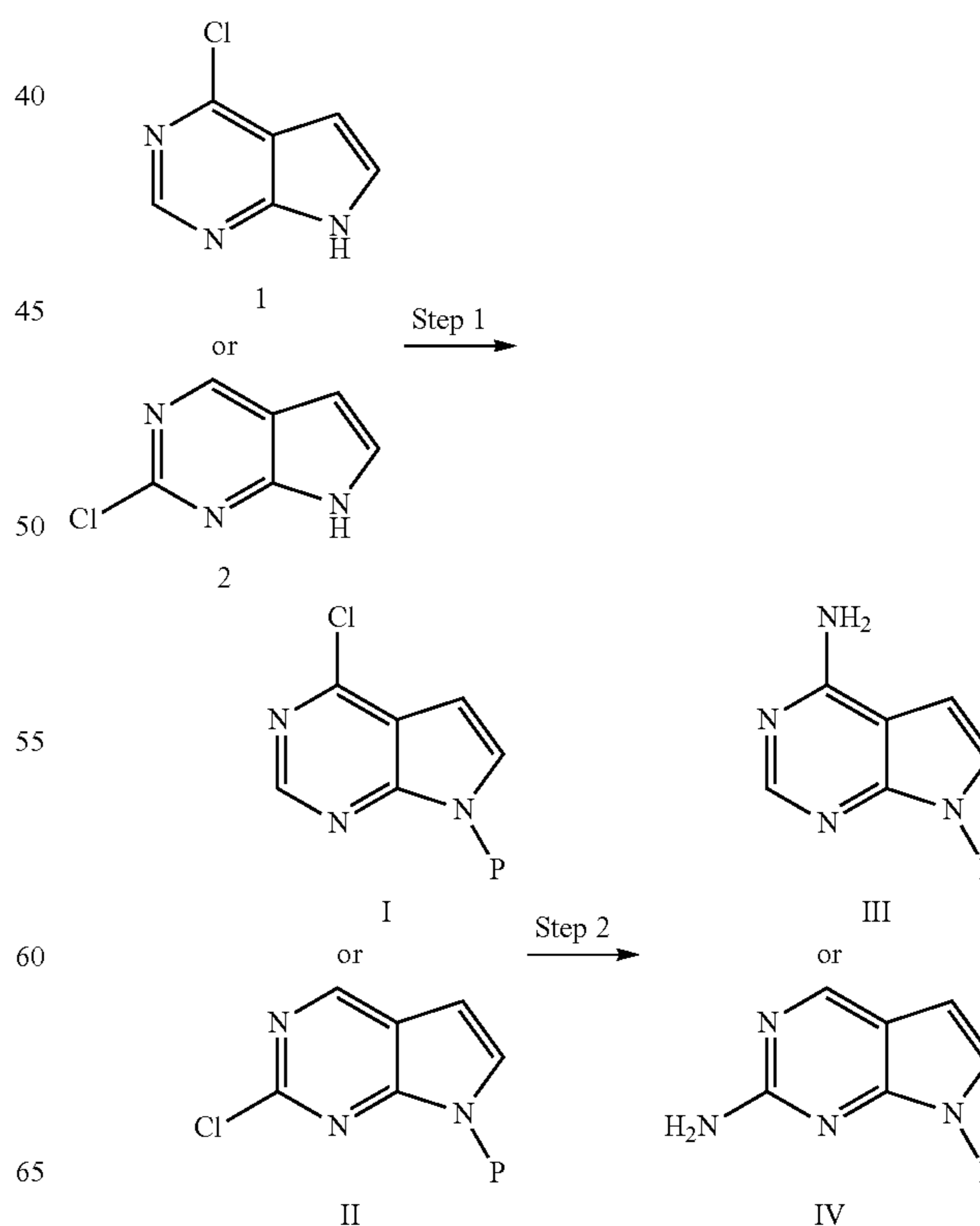
Scheme II
