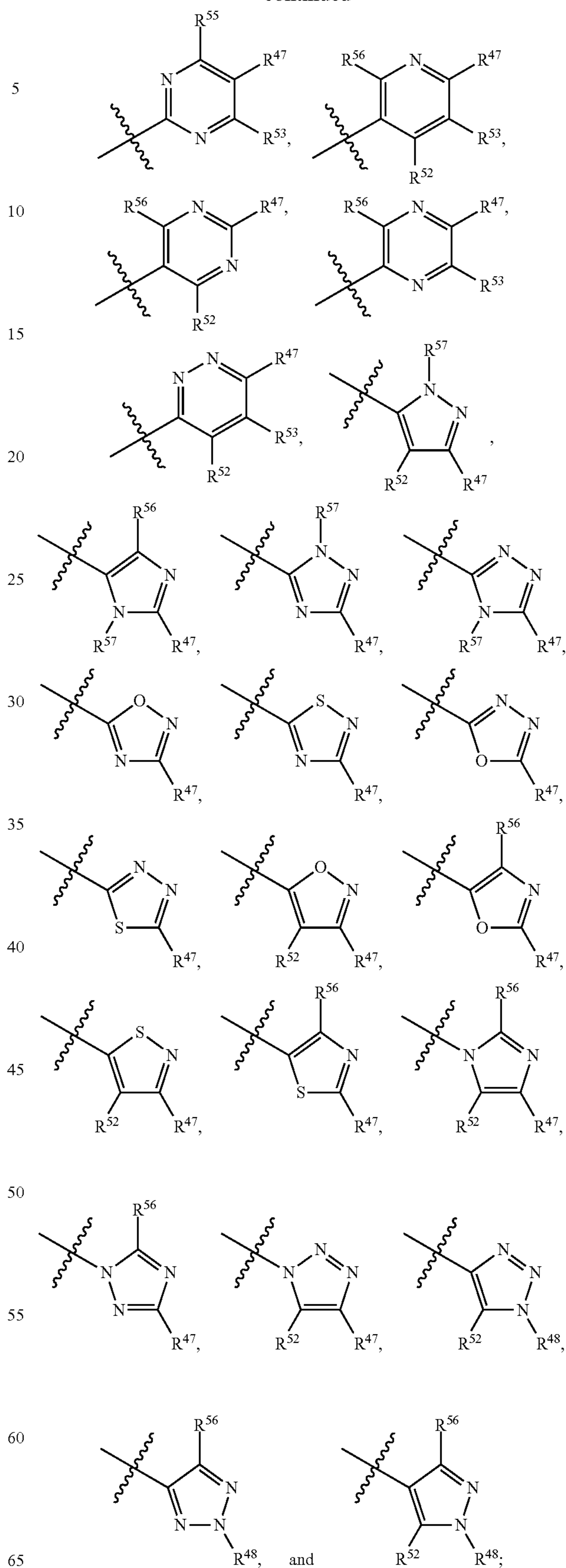
Formula Ia
