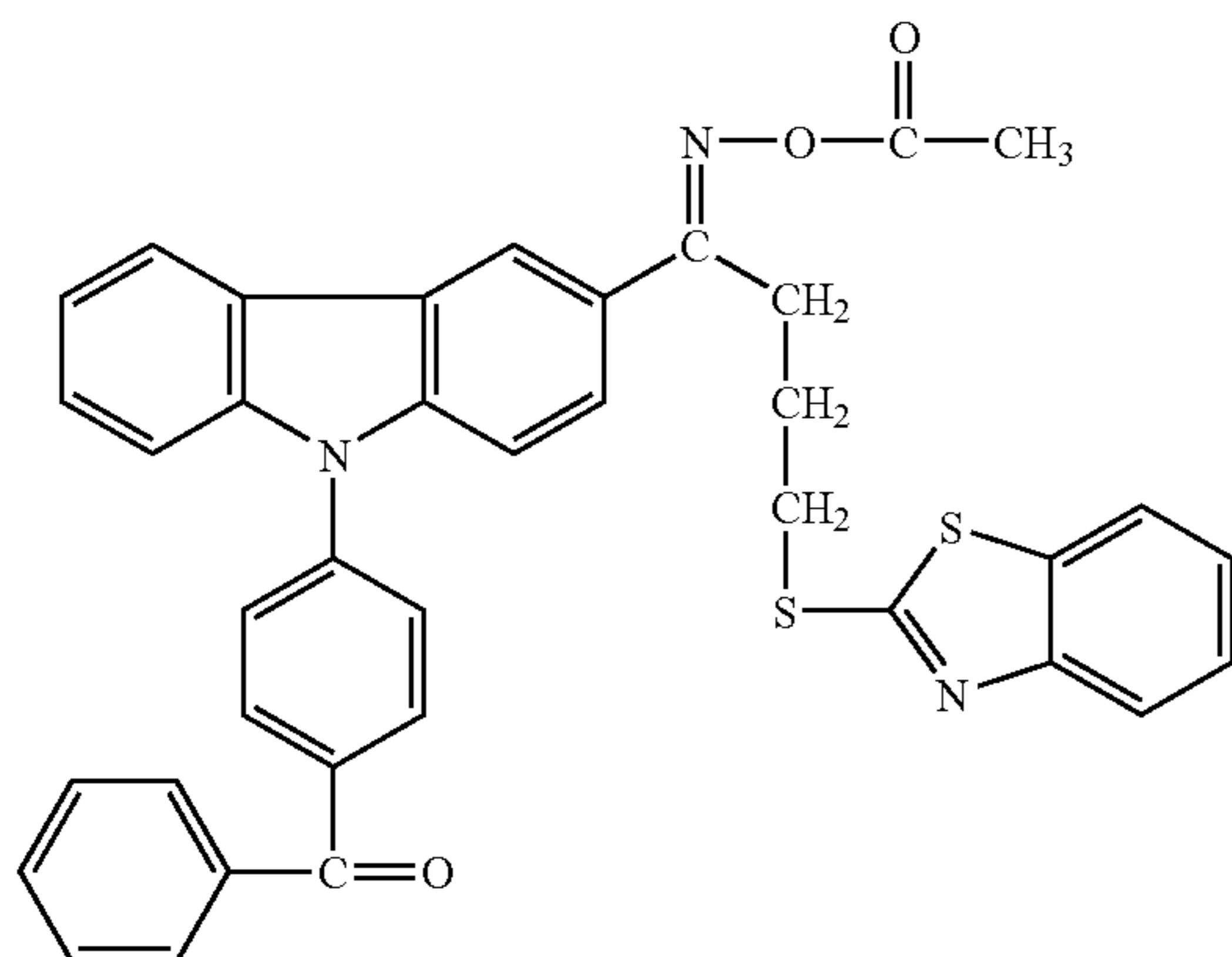
7.a (4-Carbazol-9-yl-phenyl)-phenyl-methanone
