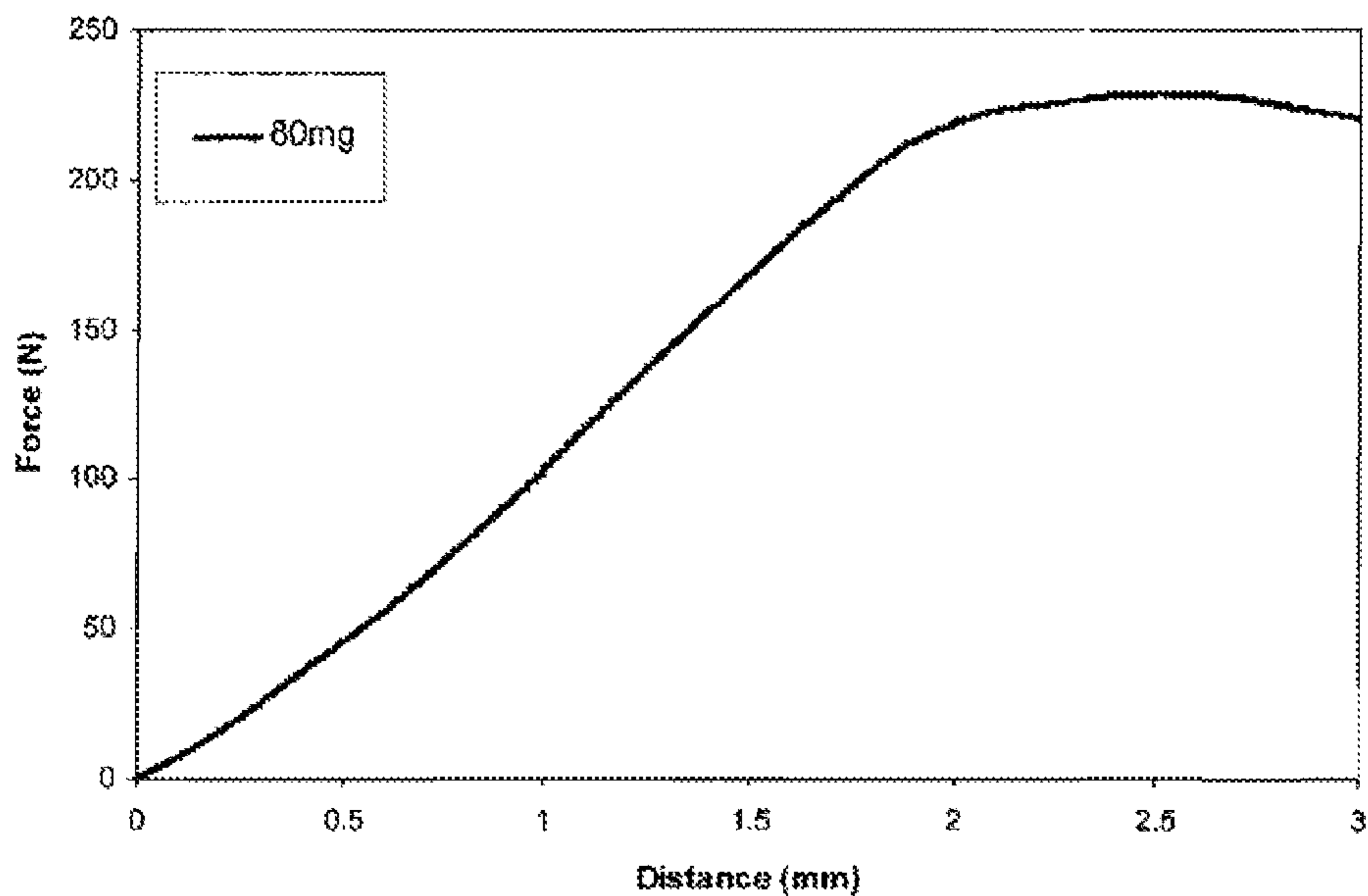
Example 20 Indentation Test of Example 16.2 tablet
