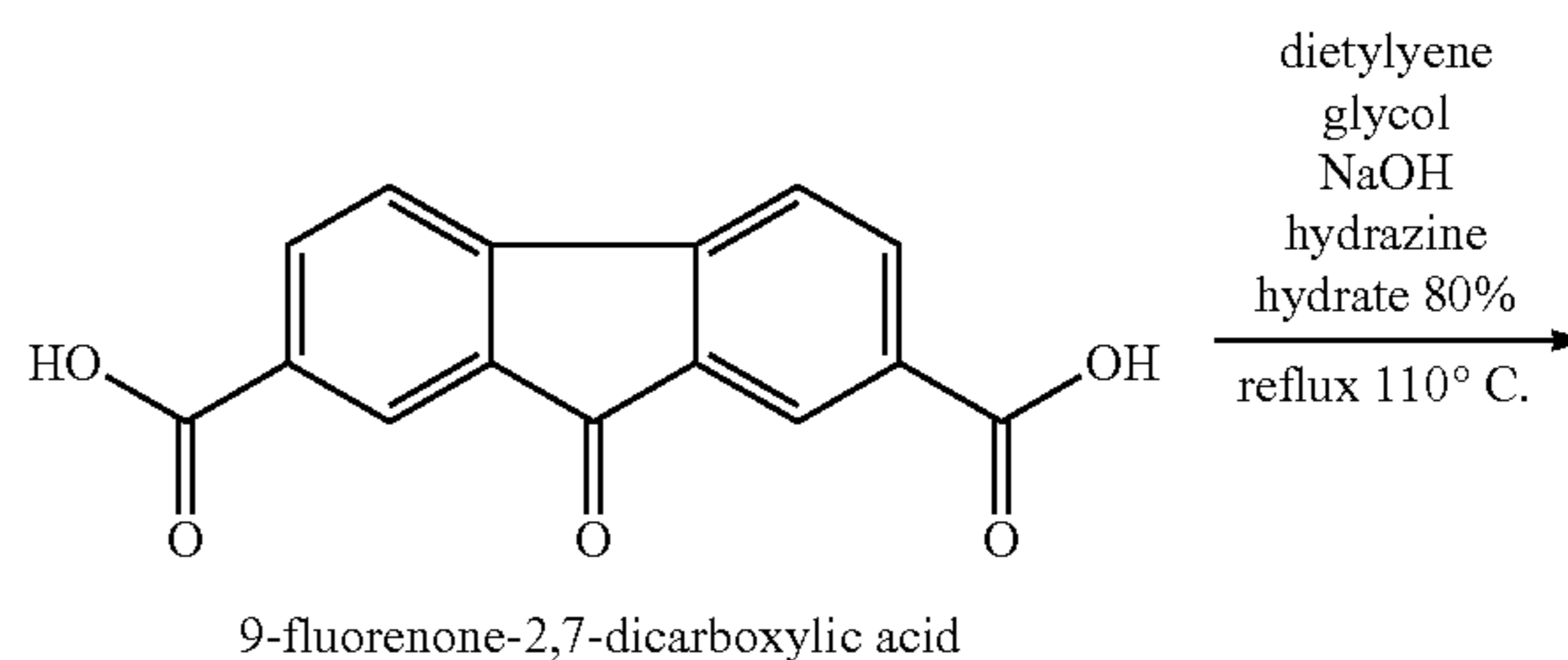
Scheme 5.
