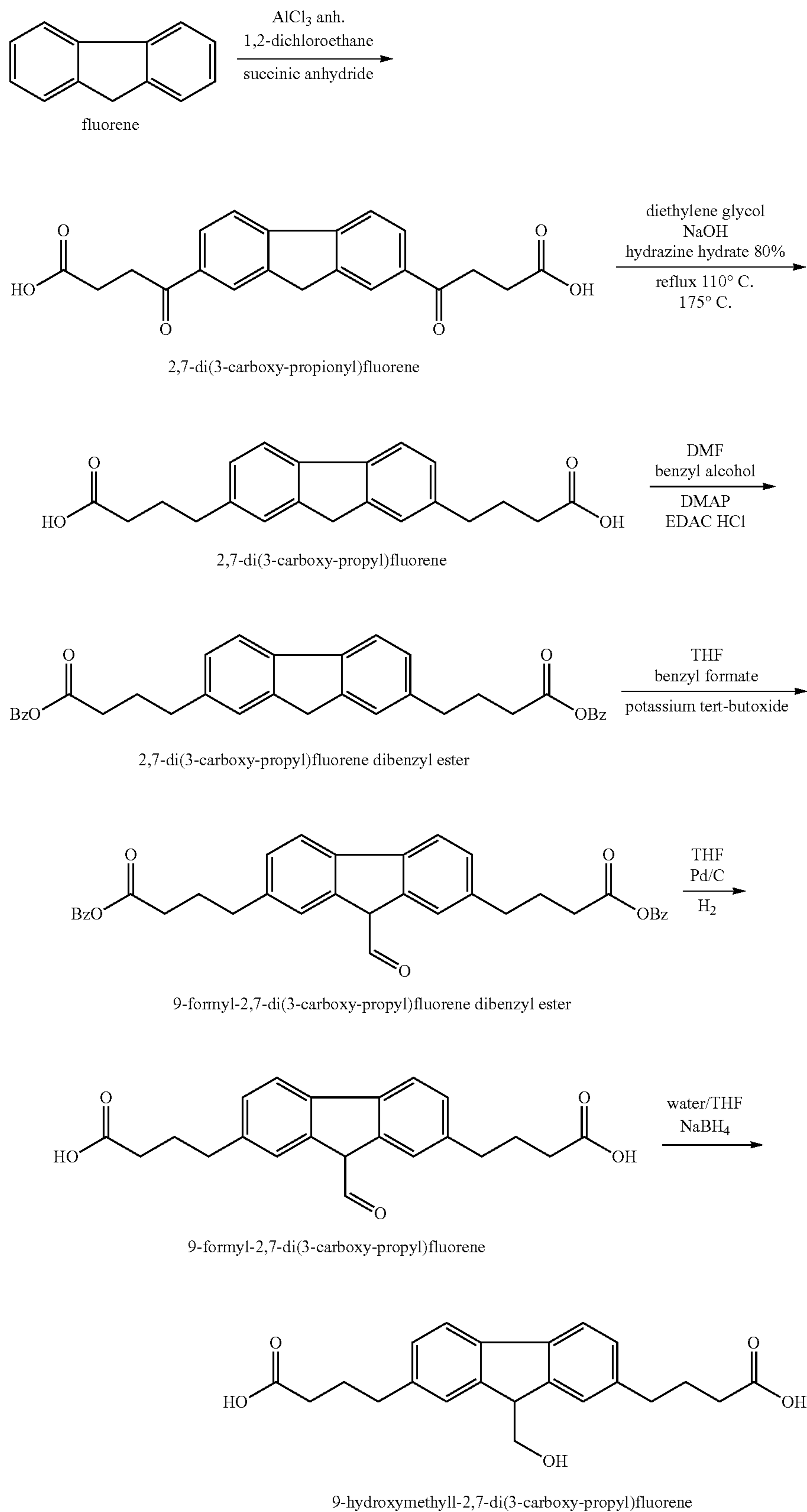
Scheme 6.
