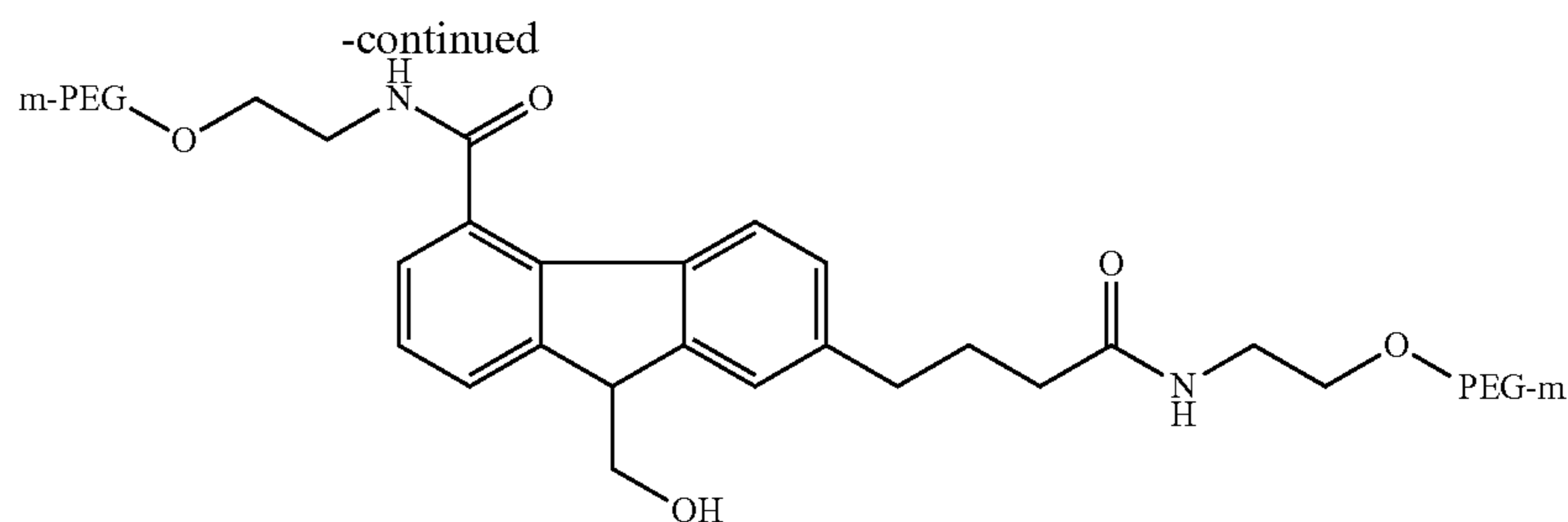
9-hydroxymethyl-4-(mPEG(10,000)-carboxyamide)-7-(3-(mPEG(10,000))carbamoyle-propyl)fluorene
