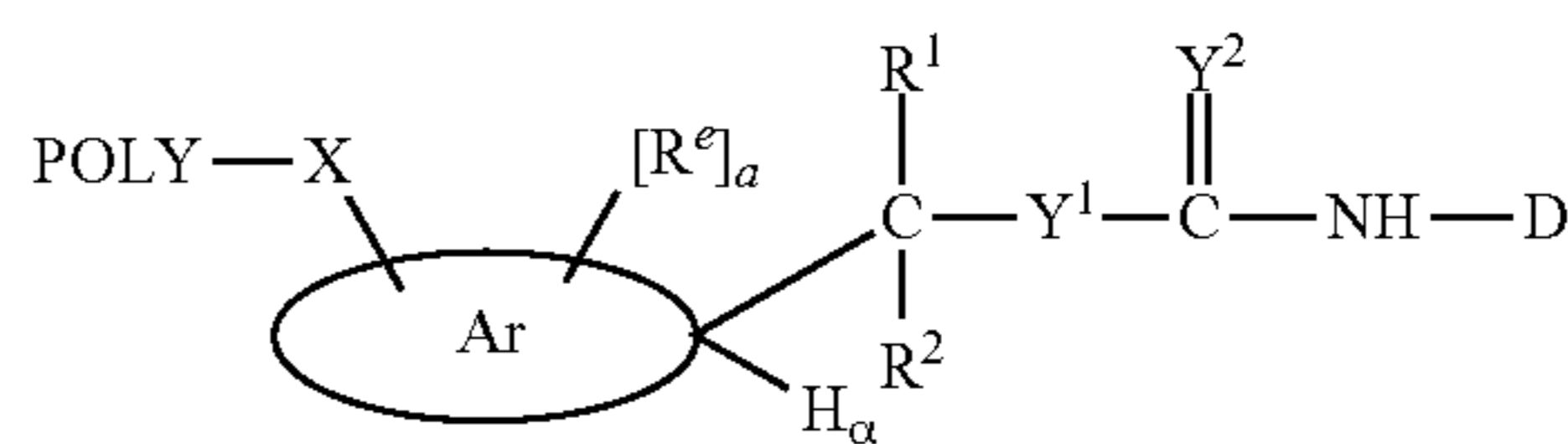
(Formula VI-C) 25
