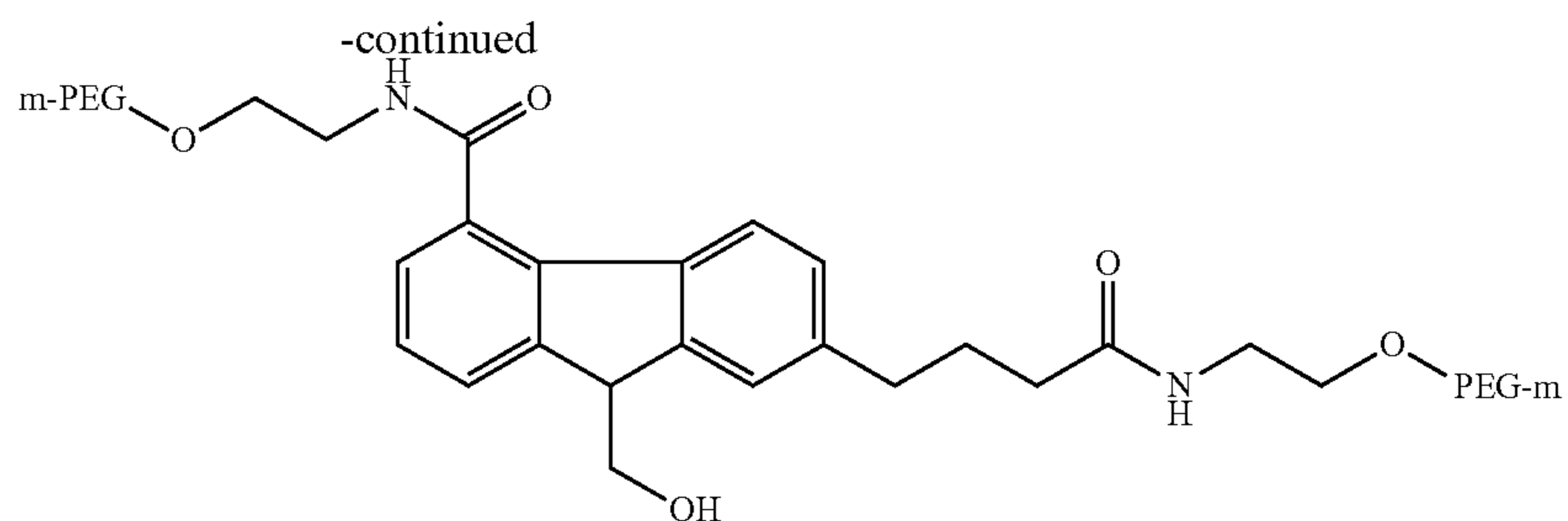
9-hydroxymethyl-4-(mPEG(10,000)-carboxyamide)-7-(3-(mPEG(10,000))carbonyl-propyl)fluorene
