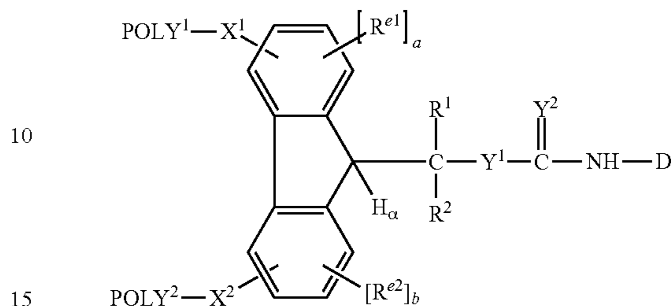
(Formula III-C)
