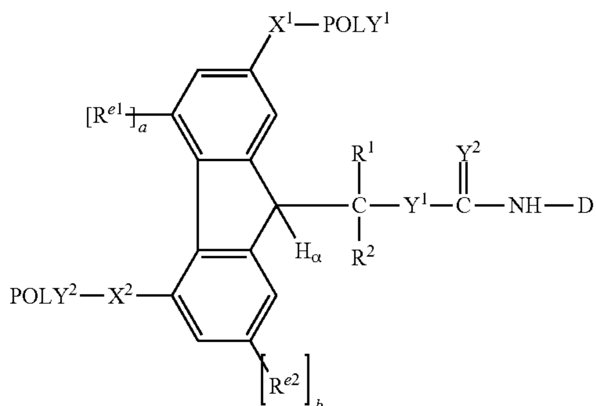
(Formula Vf-C) 15
