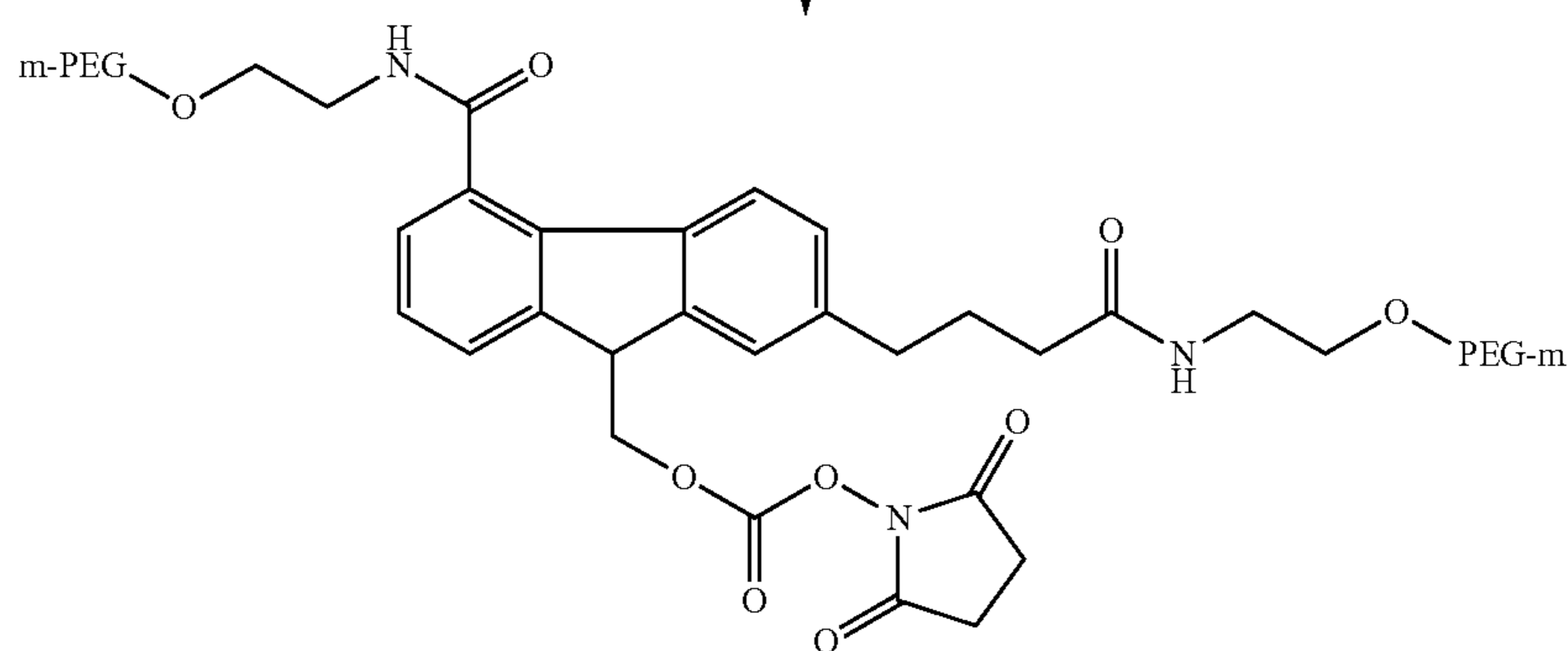
9-hydroxymethyl-4-(mPEG(10,000)-carboxyamide)-7-(3-(mPEG(10,000))carbamoyle-propyl)fluorene-N-hydroxysuccinimide
