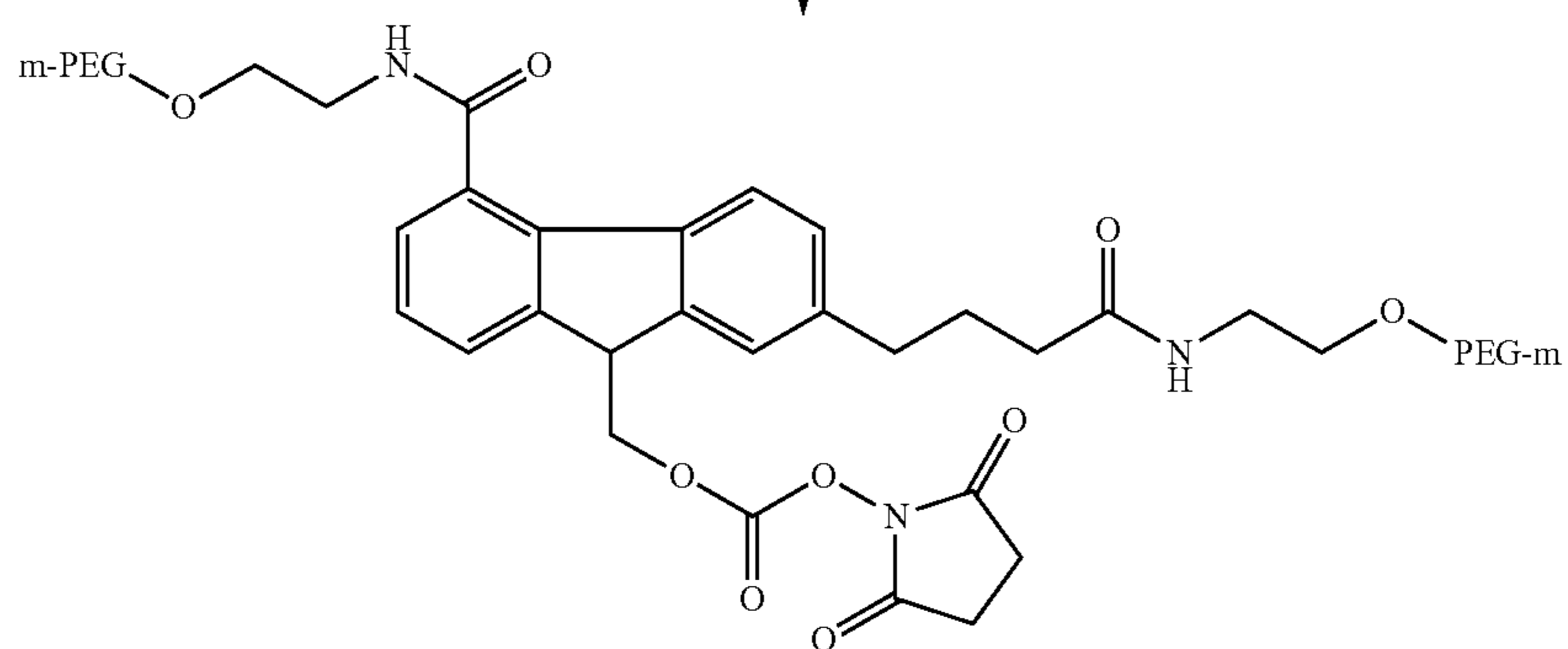
9-hydroxymethyl-4-(mPEG(10,000)-carboxyamide)-7-(3-(mPEG(10,000))carbonyl-propyl)fluorene-N-hydroxysuccinimide
