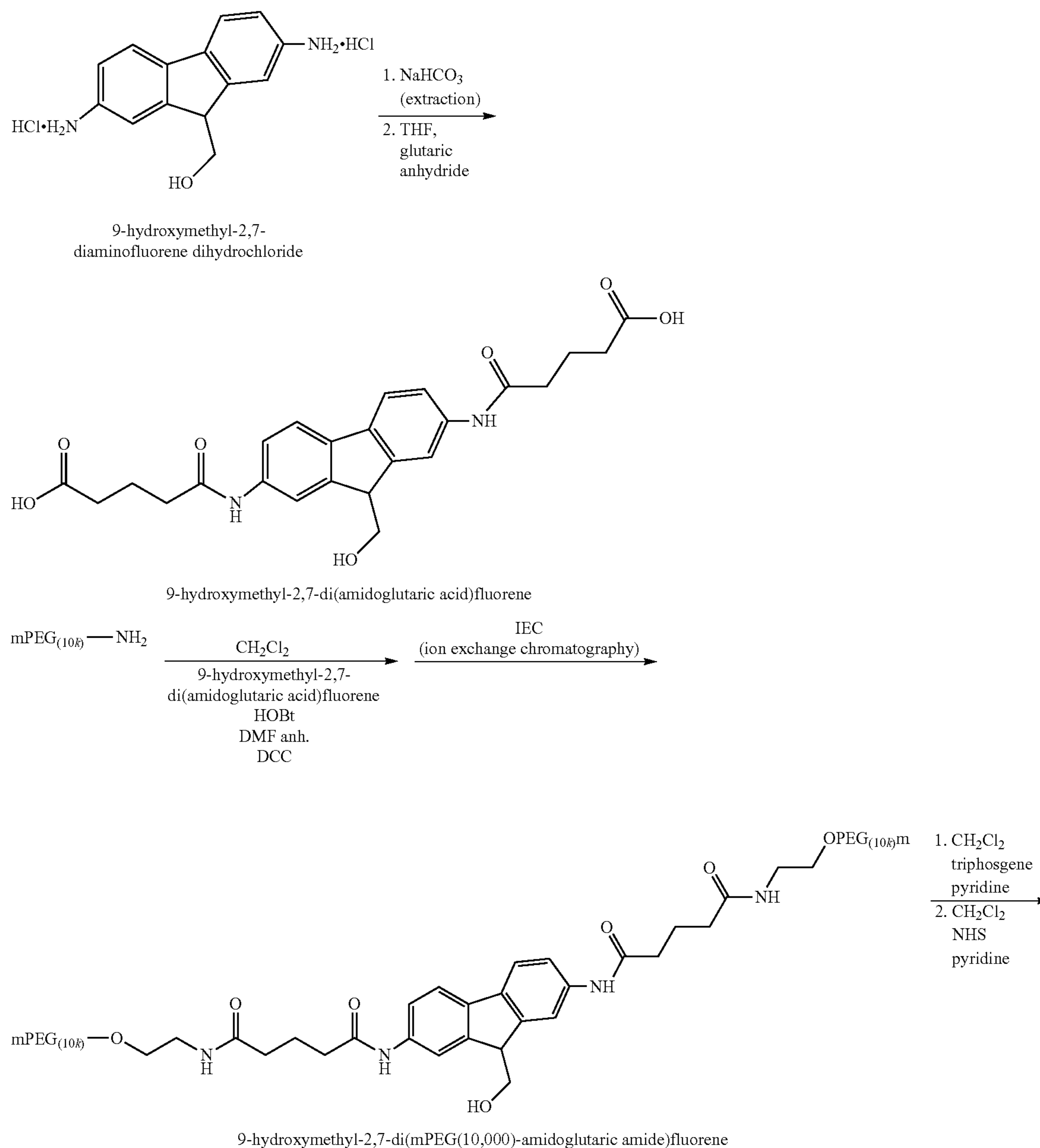
Scheme 2
