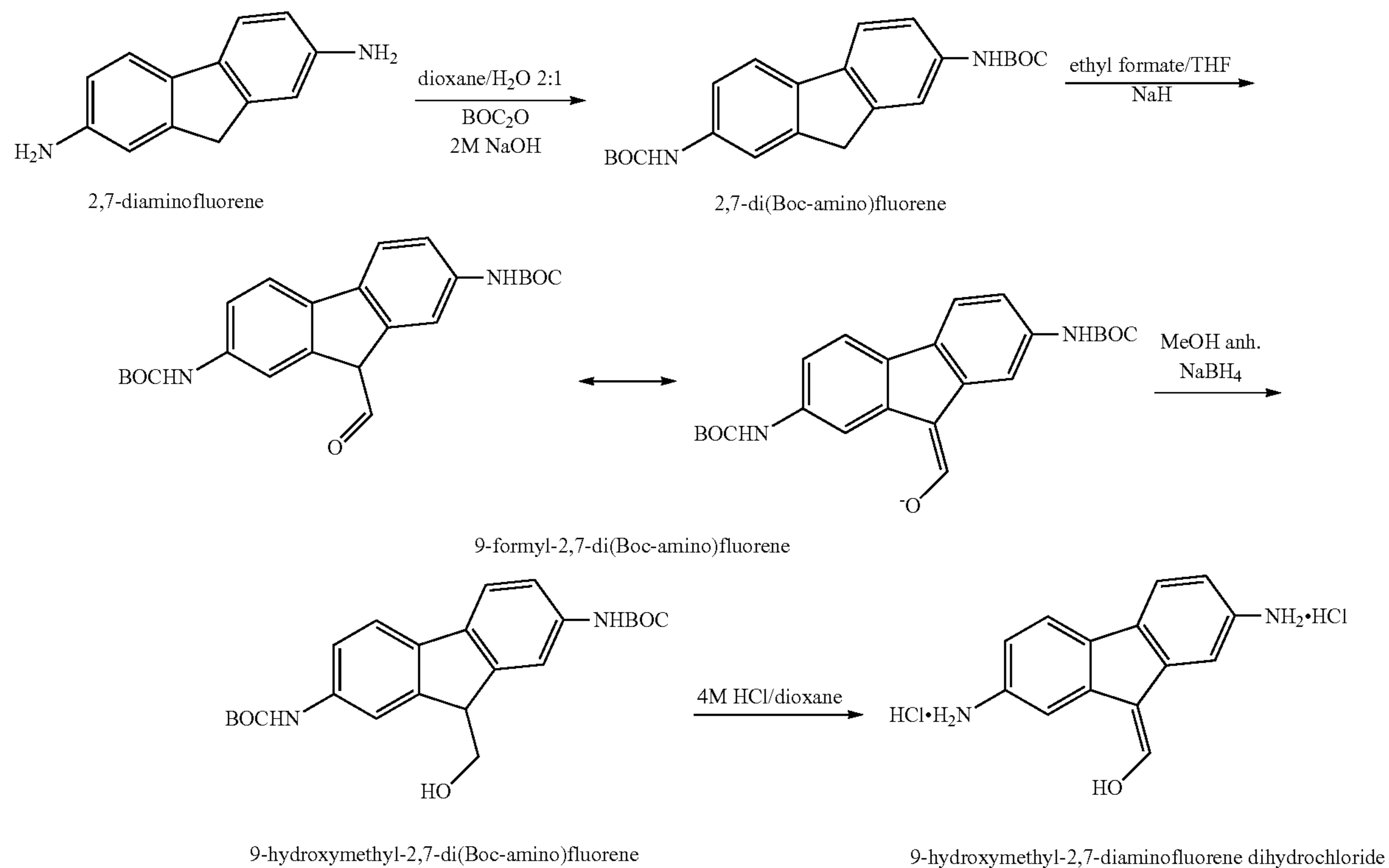
Scheme 1.
