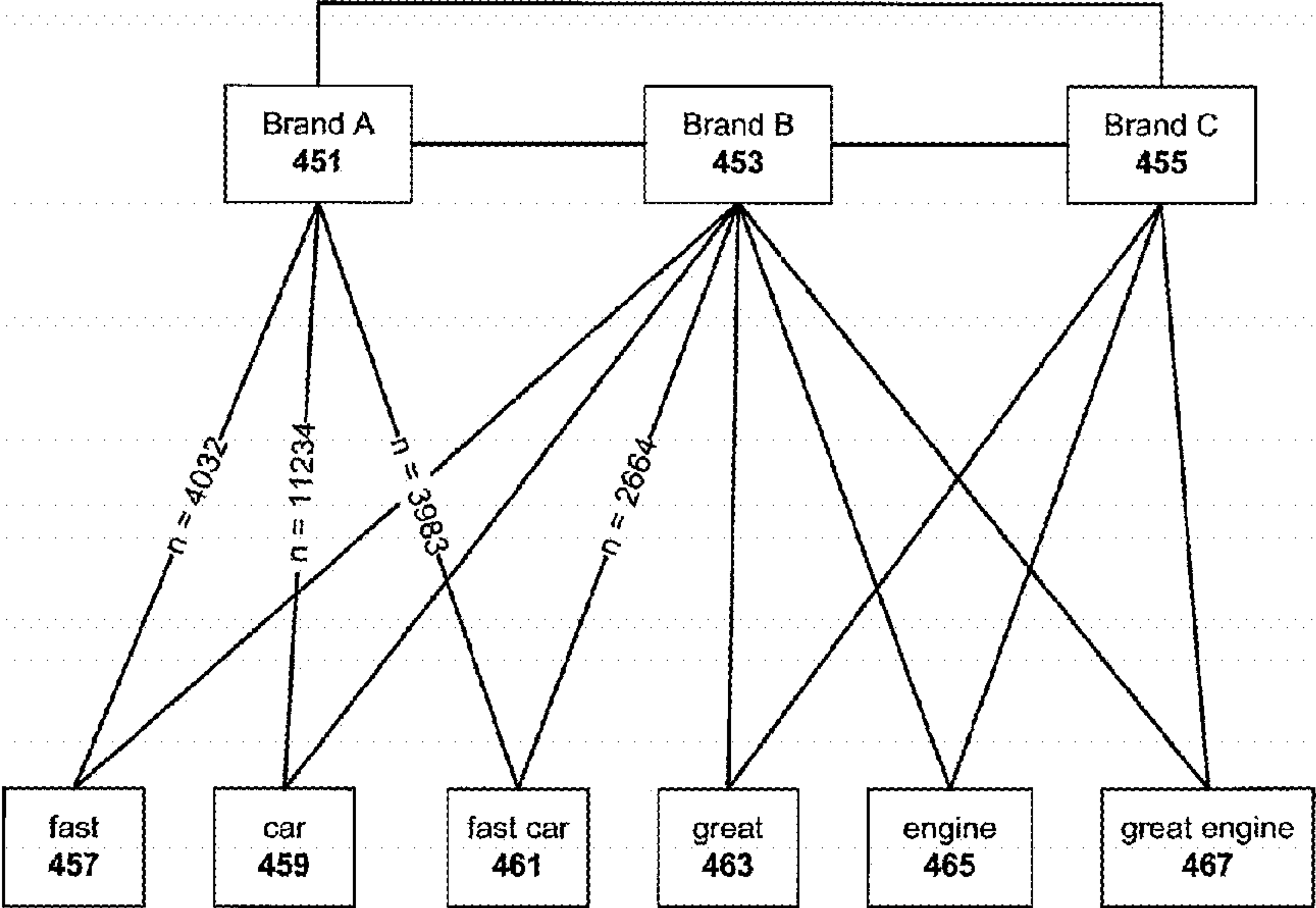
Excerpt of an Aggregated Term Graph 400D
