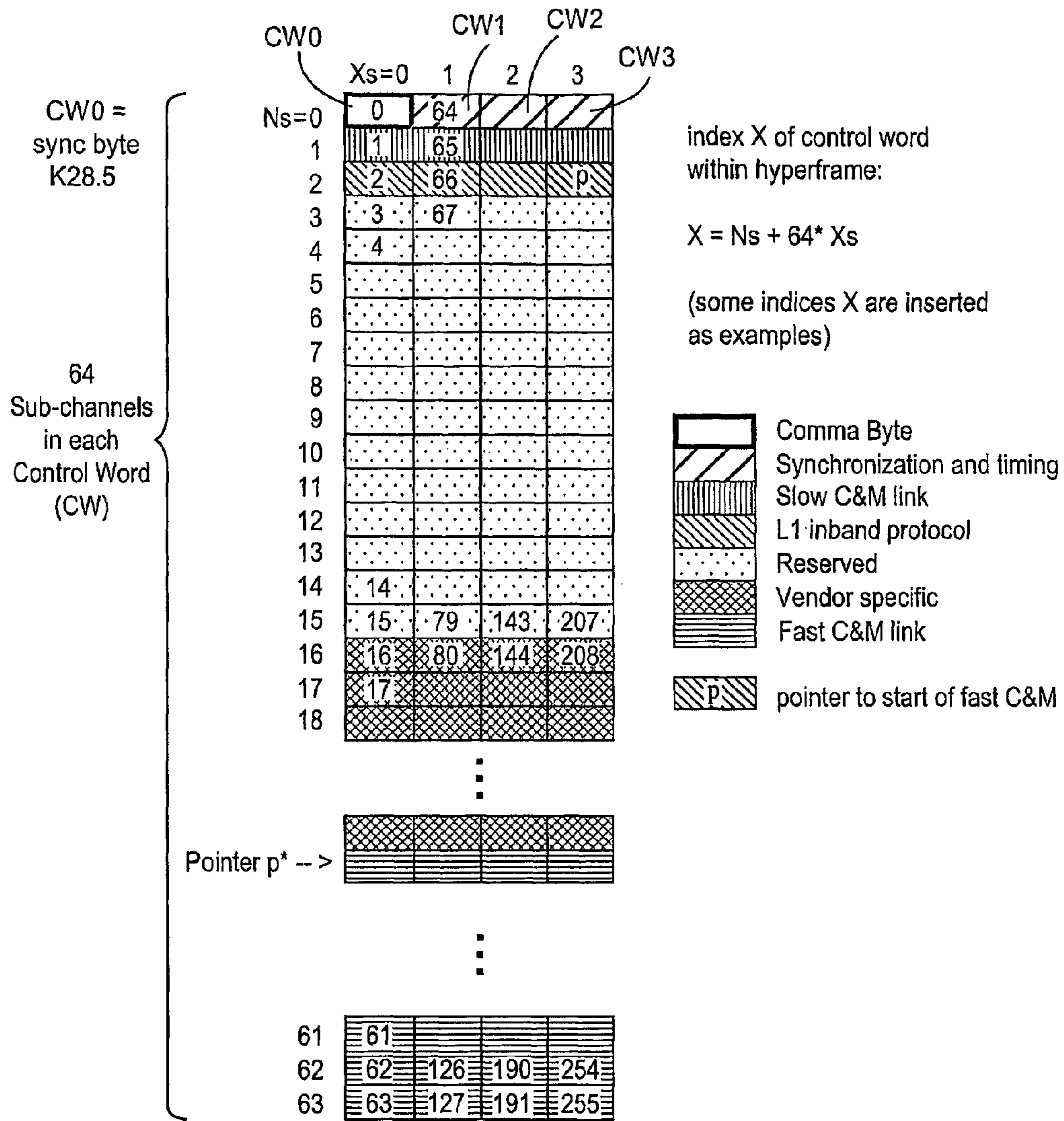
Illustration of subchannels within one hyperframe
