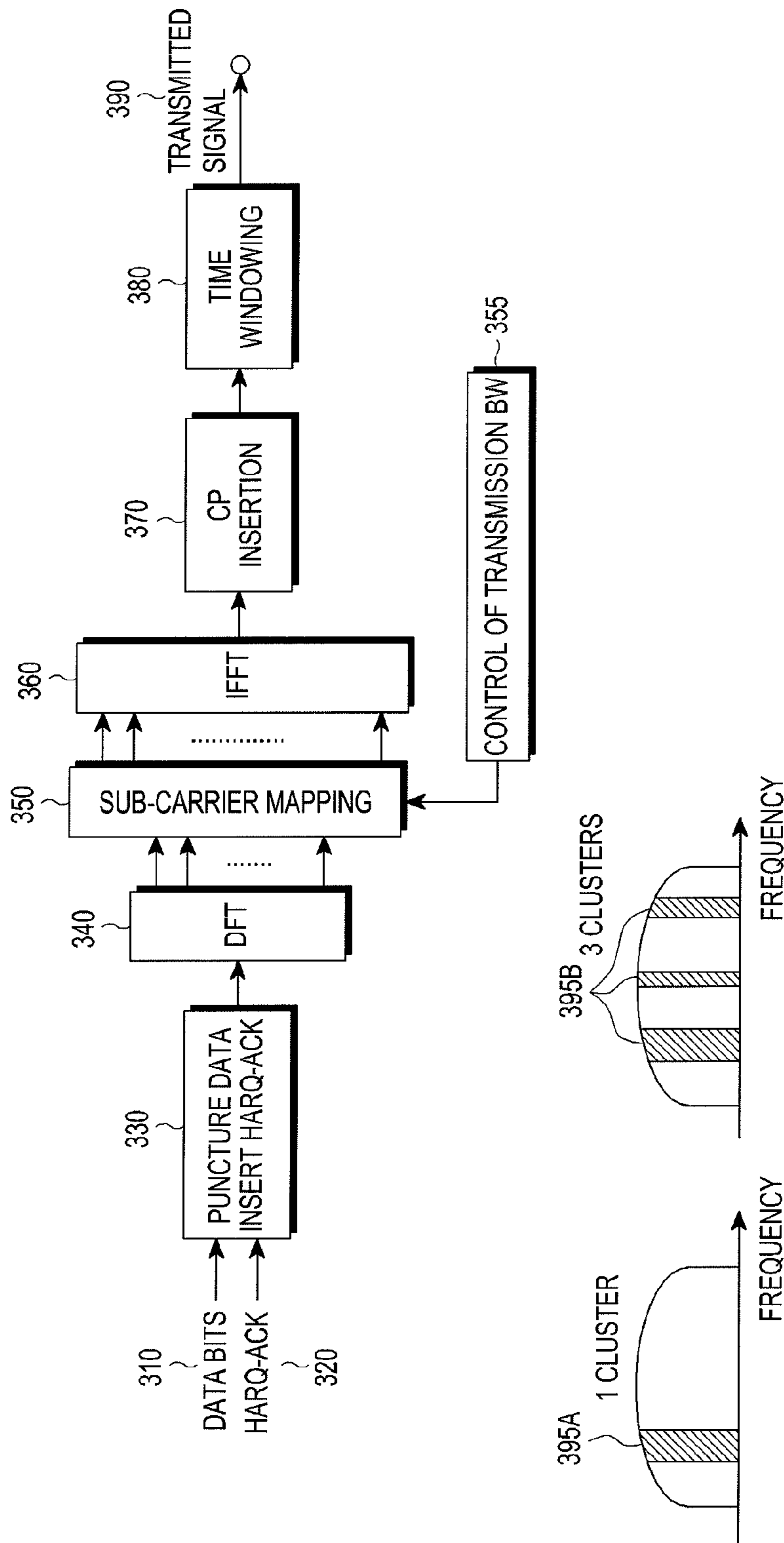
FIG. 3 (RELATED ART)
