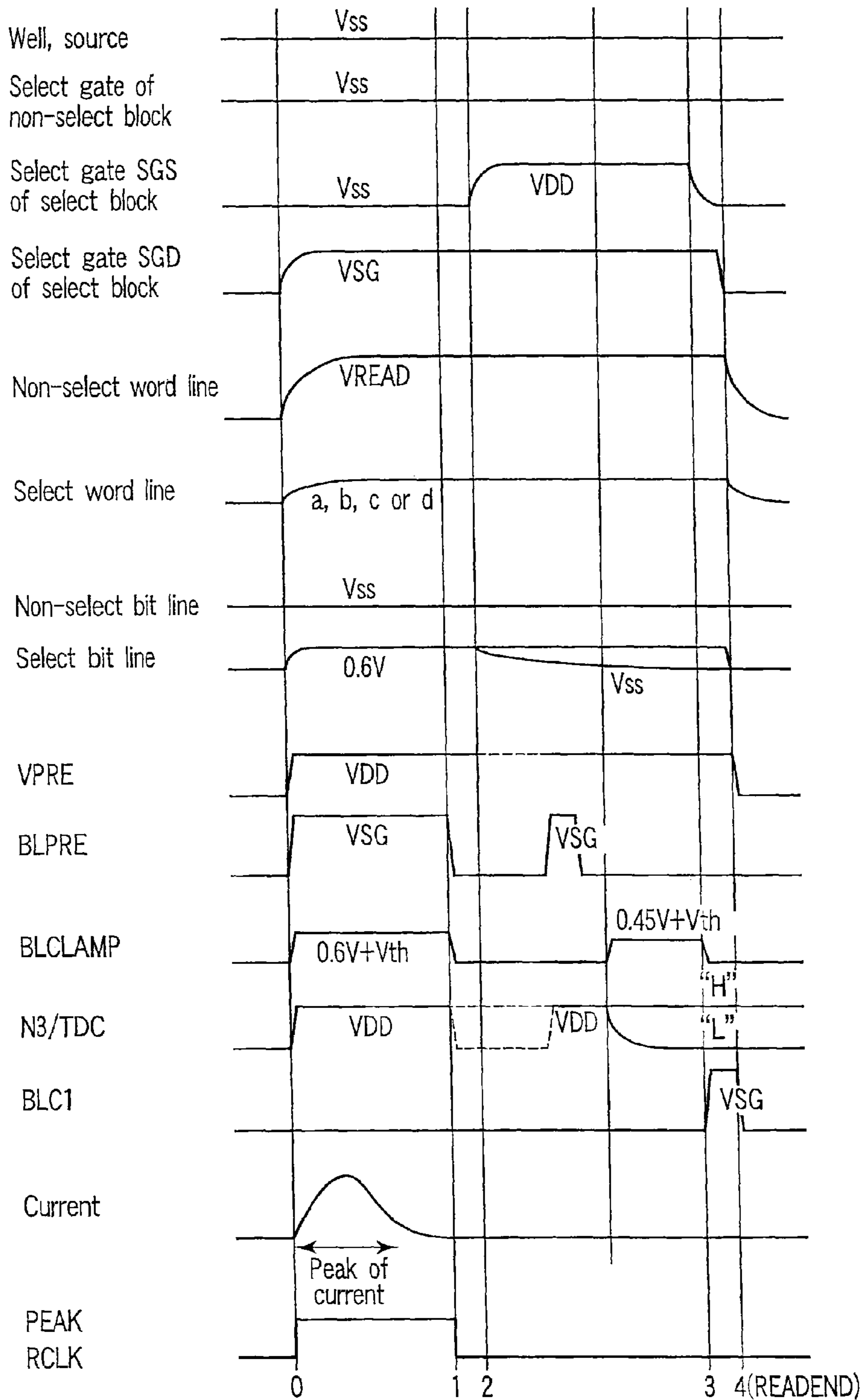
Waveform of read, verify read operation
