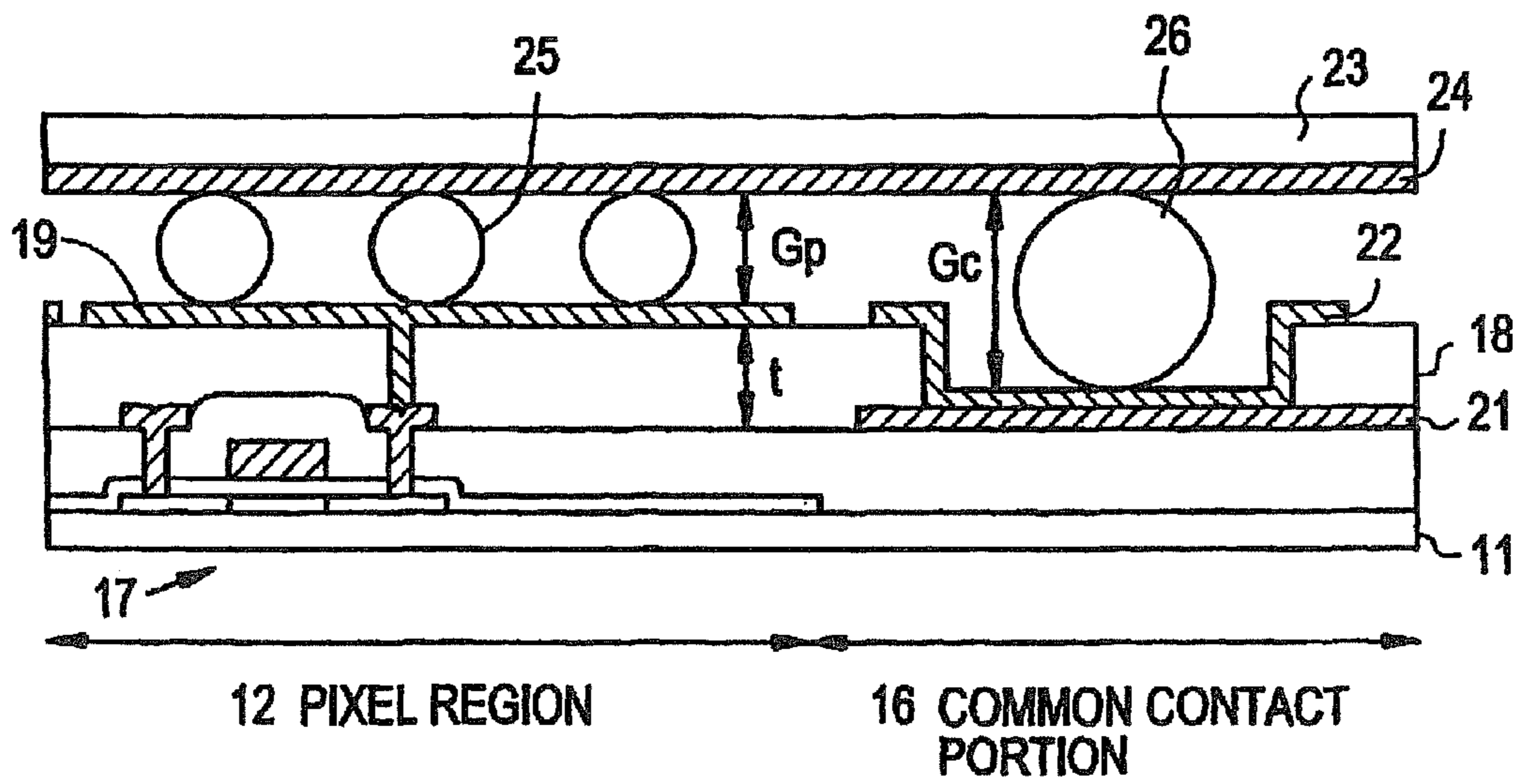
FIG. 13 PRIOR ART
