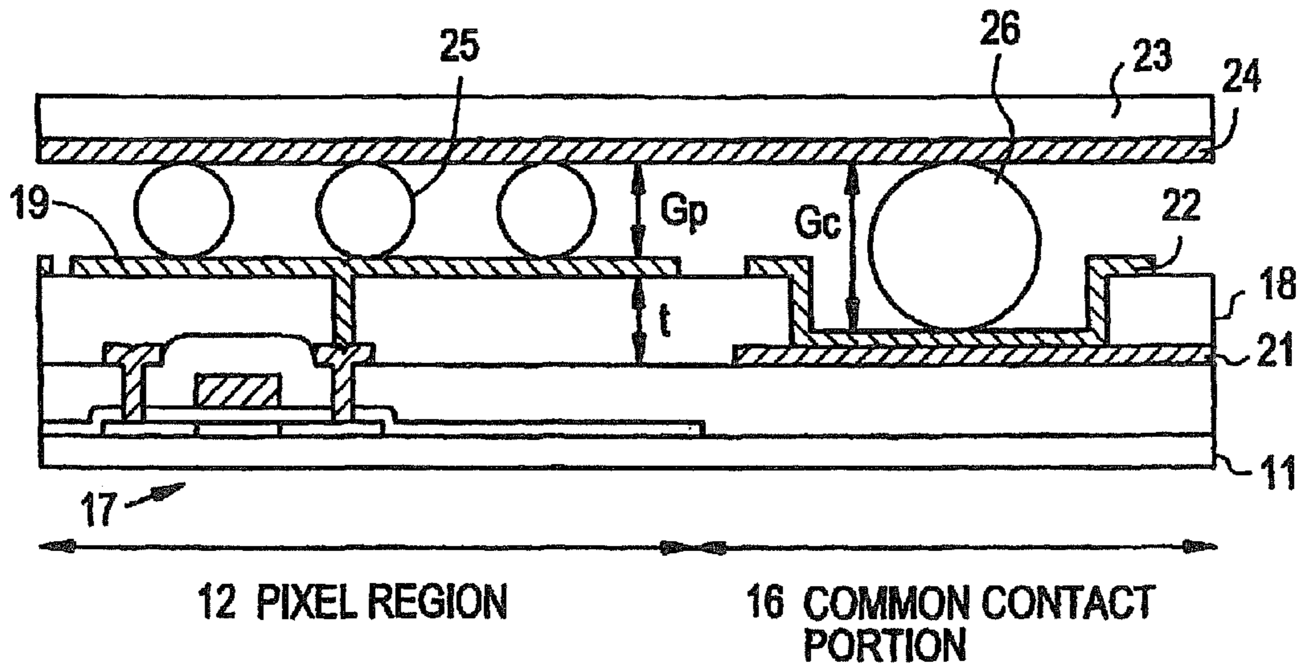
FIG. 13 PRIOR ART
