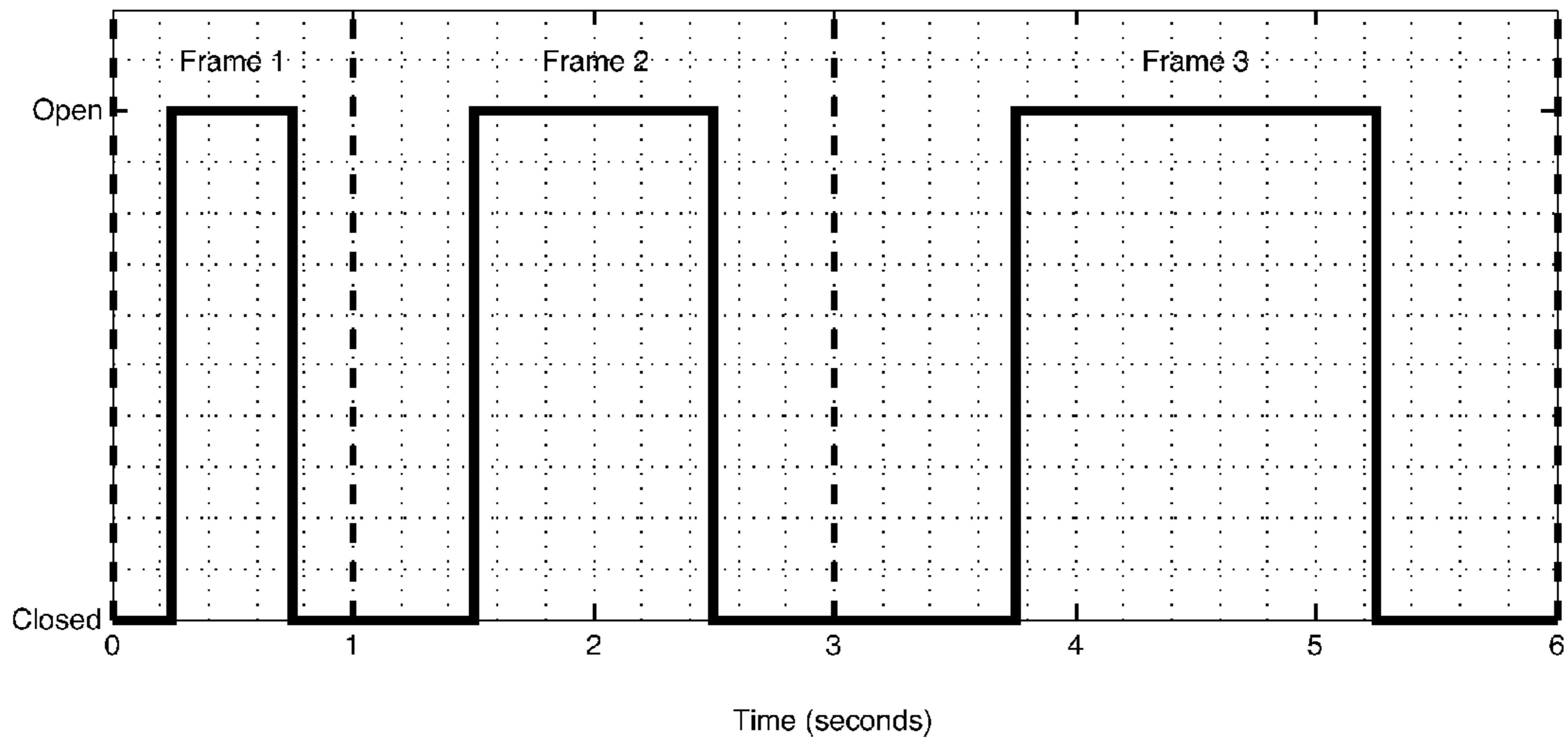
LCD Opacity
