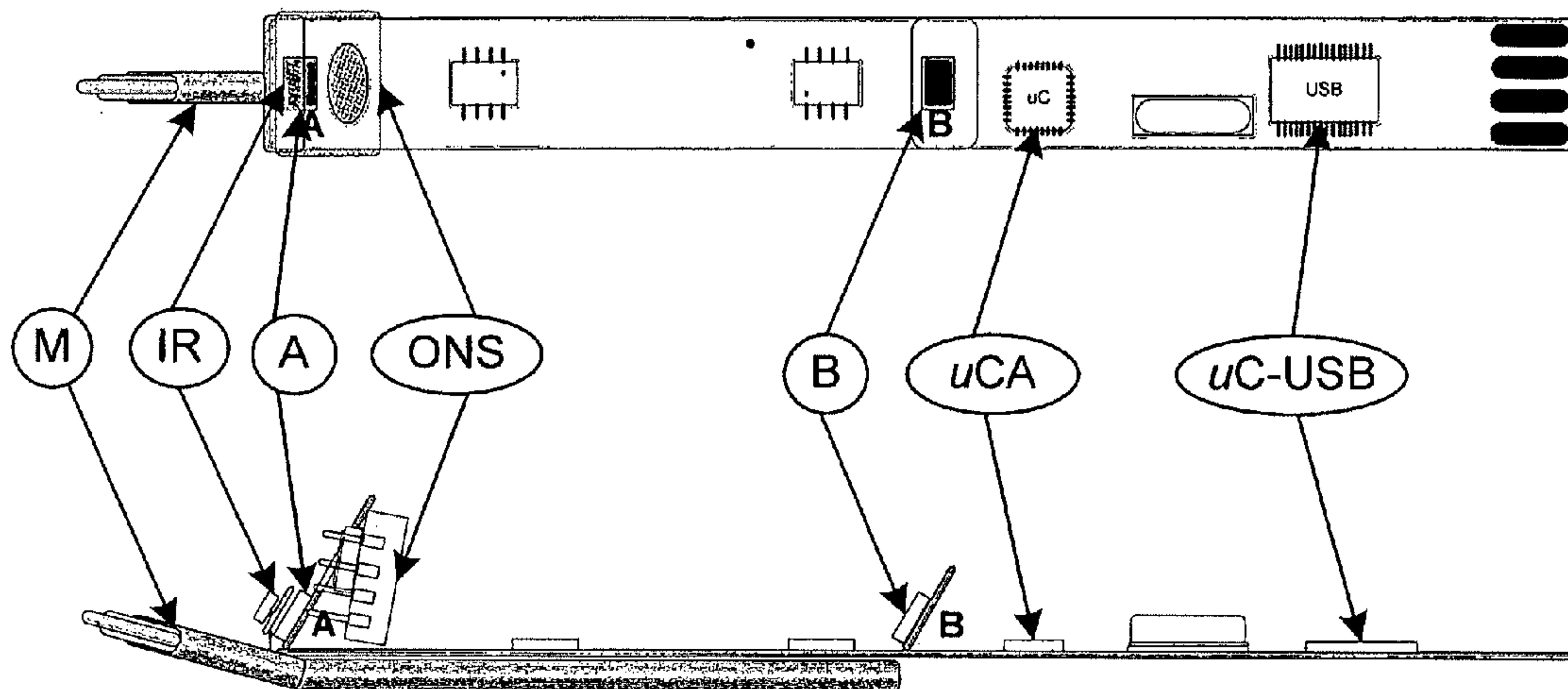
Fig. 5 -ONS, MEMS A, MEMS Topology, pen refill.
