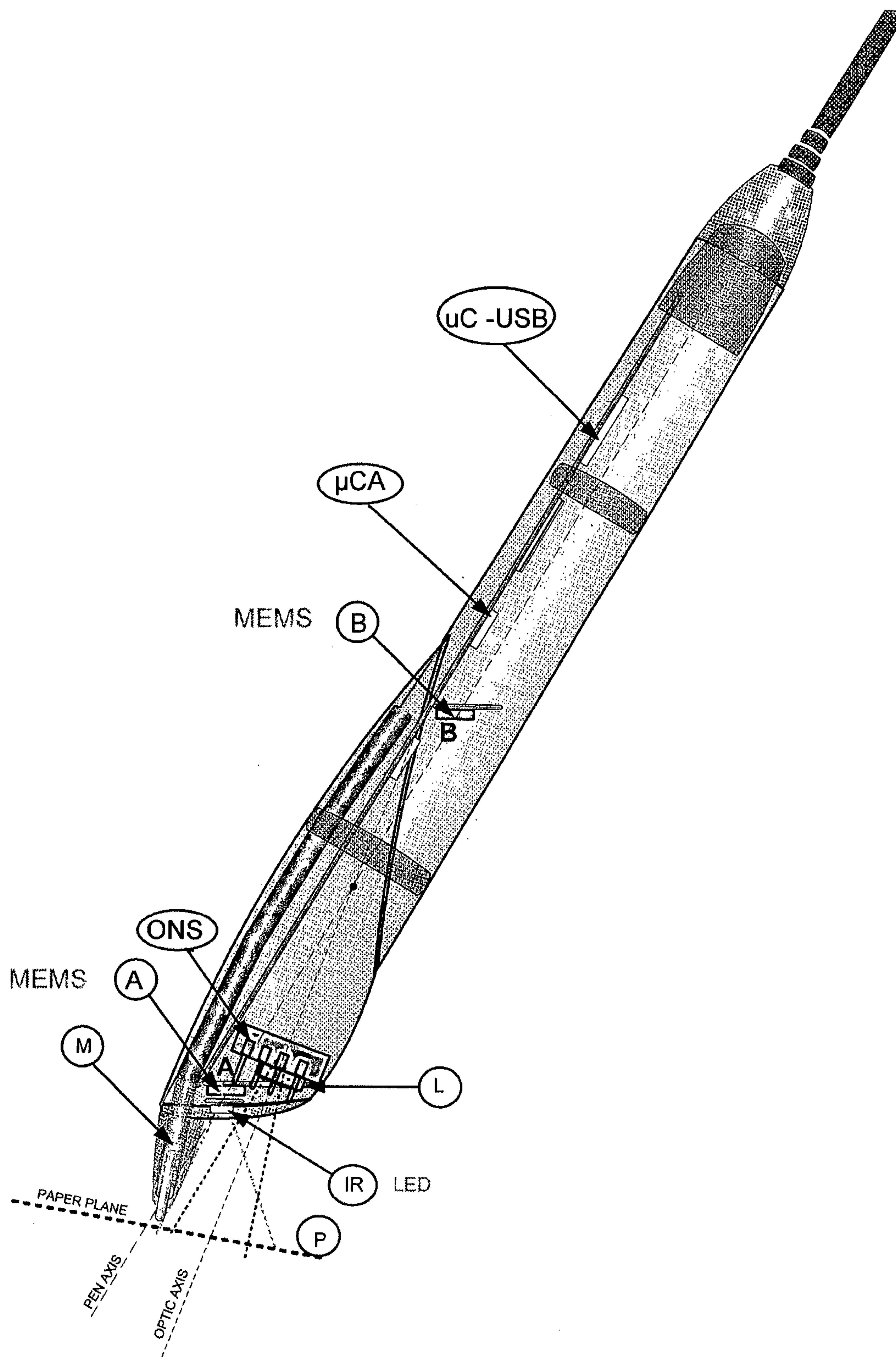
Fig. 3 – Signature capture mode diagram – pen.
