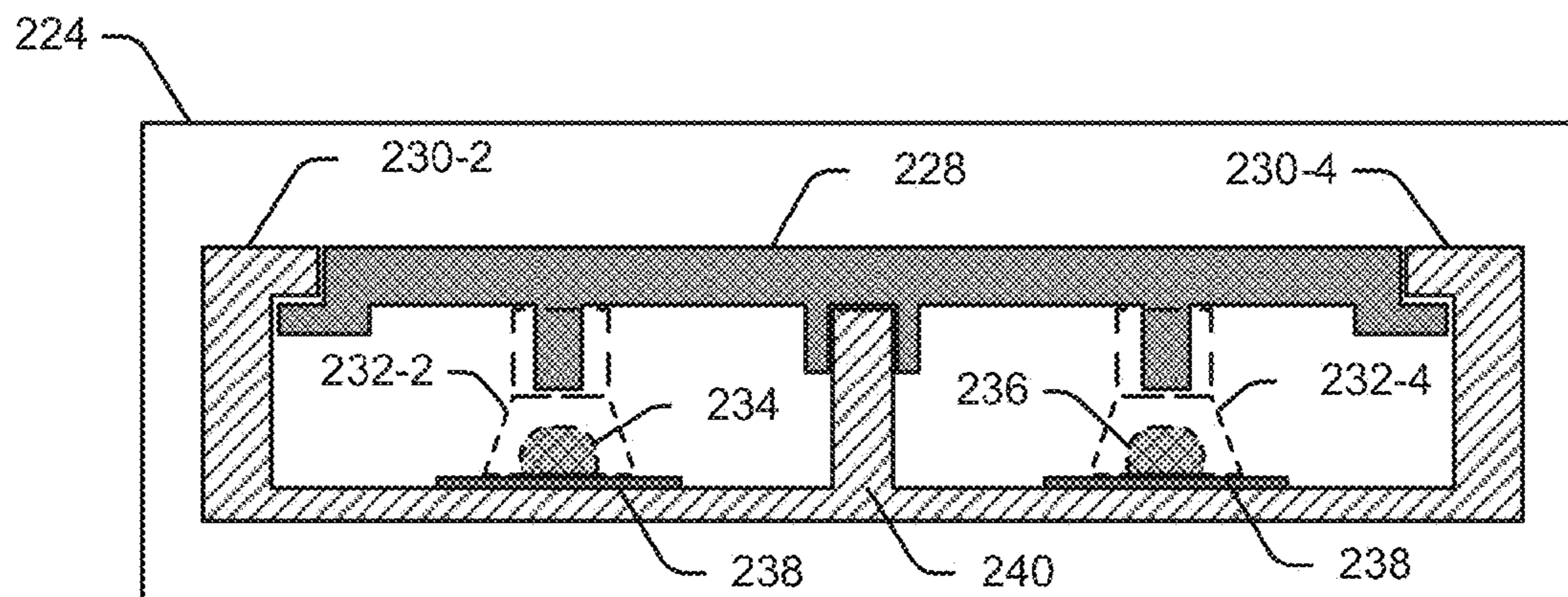
(2) Cross-sectional view 224 of a trackpad 226
