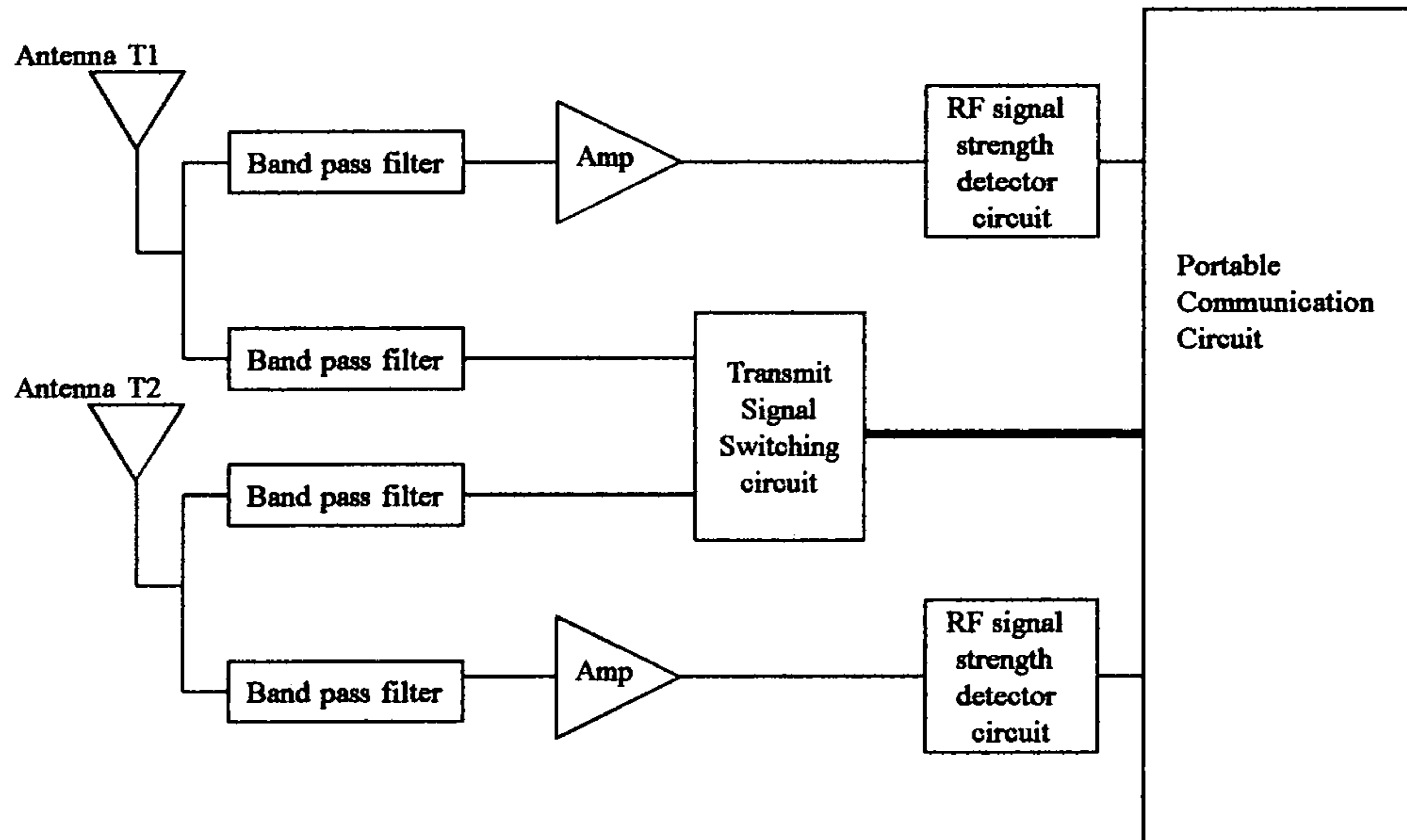
Fig 4. Two antenna Portable Communication Device block diagram
