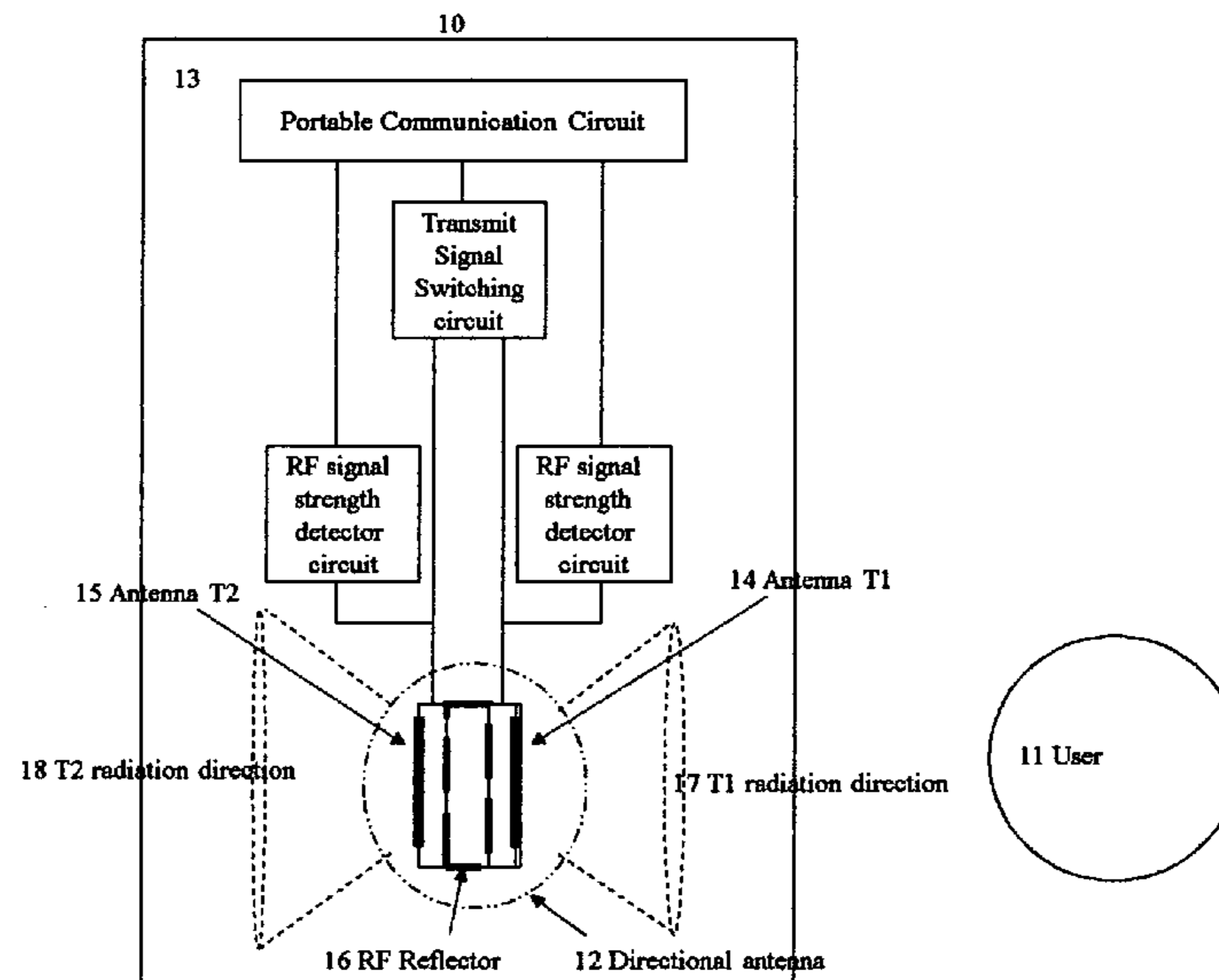
Portable communication system with one directional antenna radiating toward user
