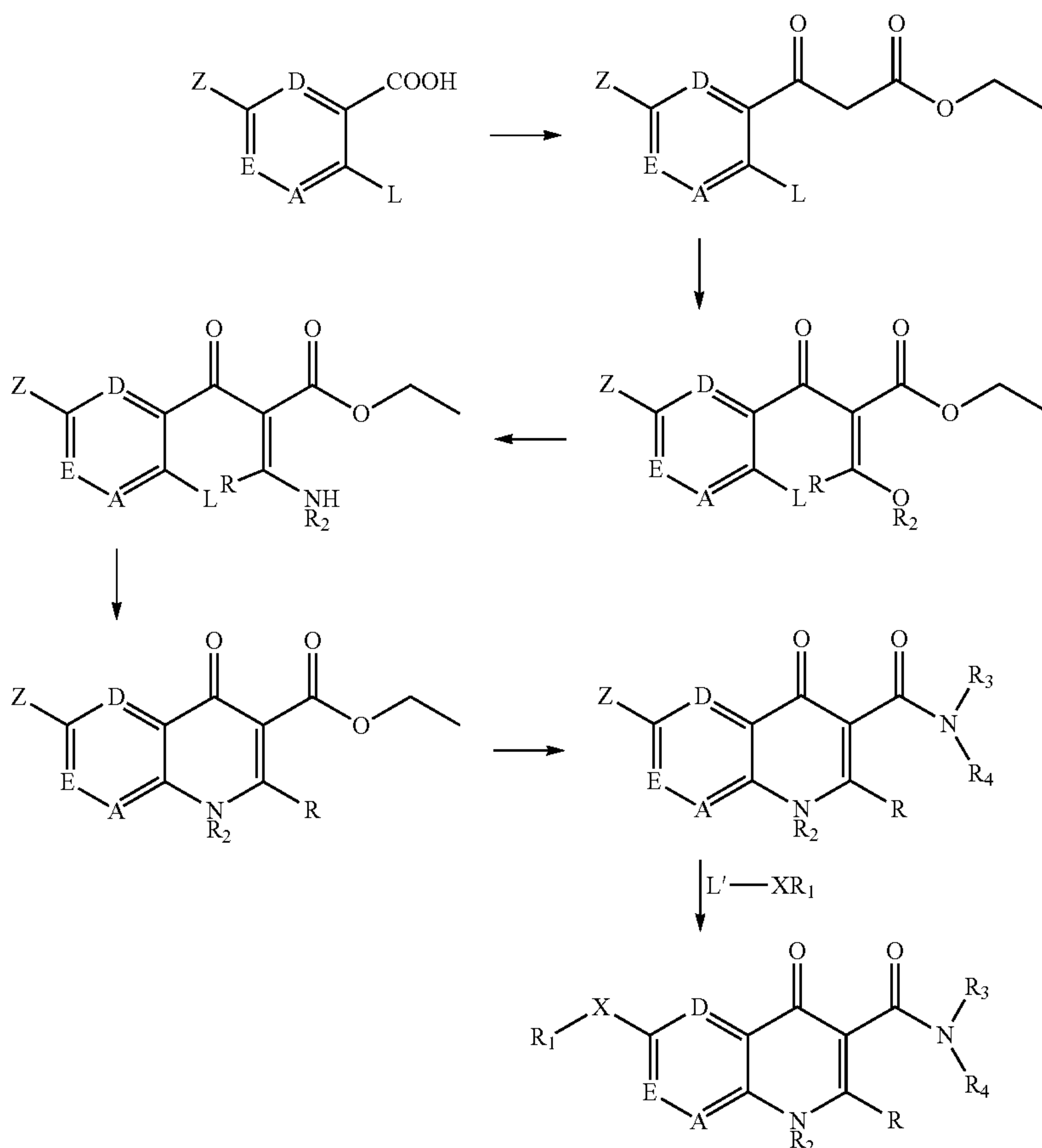
Scheme 2
