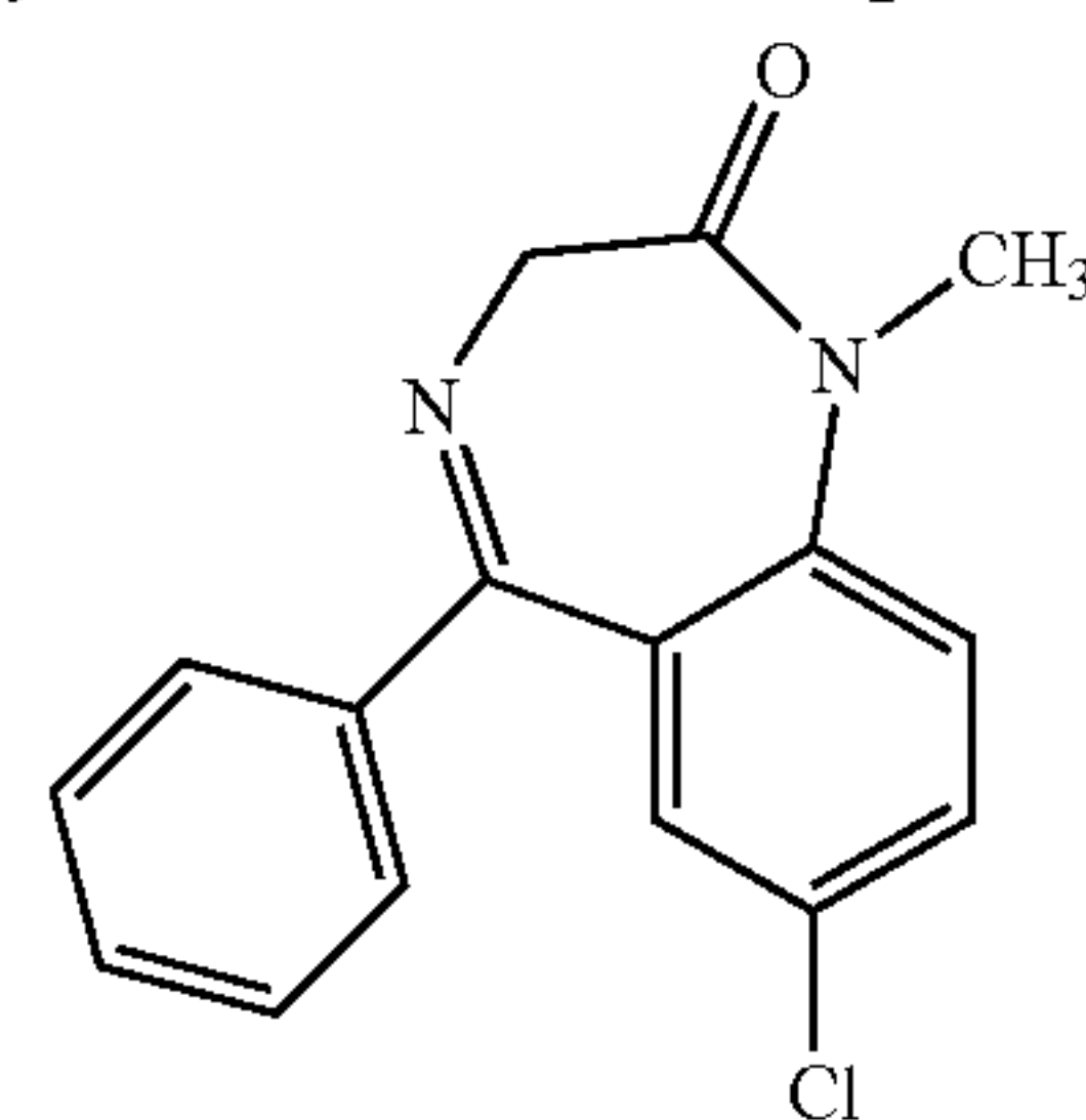
Diazepam
