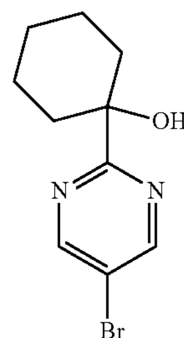
MS 257.0 & 259.0; 1:1 [\text{M} + \text{H}]^+ . 1-(5-bromopyrimidin-2-yl)cyclohexanol
