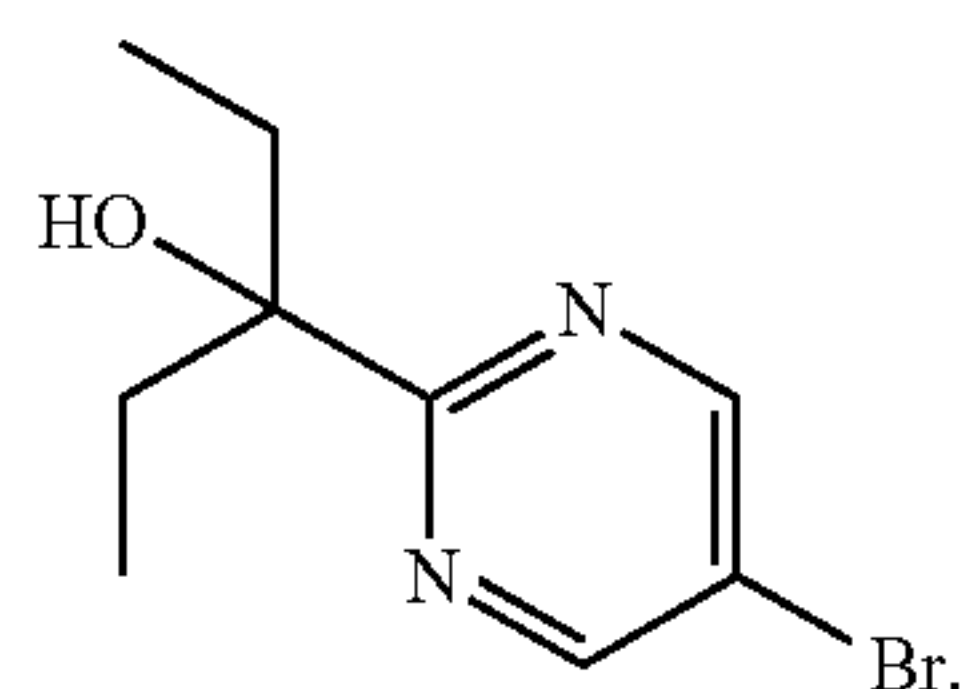
MS 244.86 [\text{M} + \text{H}]^+ 3-(5-bromopyrimidin-2-yl) pentan-3-ol
