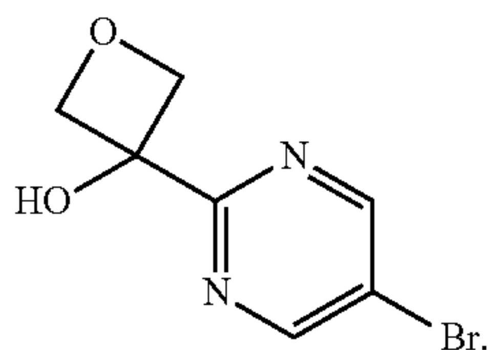
MS 230.96 & 232.94 [\text{M} + \text{H}]^+ 3-(5-bromopyrimidin-2-yl) oxetan-3-ol
