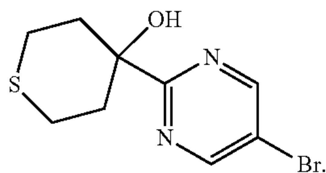
MS 276.91 [\text{M} + \text{H}]^+ 4-(5-bromopyrimidin-2-yl) tetrahydrothiopyran-4-ol
