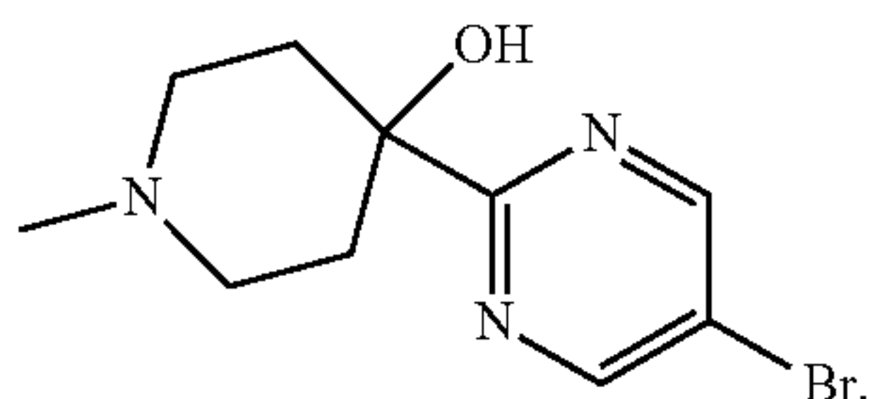
MS 270.02 [\text{M} + \text{H}]^+ 4-(5-bromopyrimidin-2-yl)- 1-methyl-piperidin-4-ol
