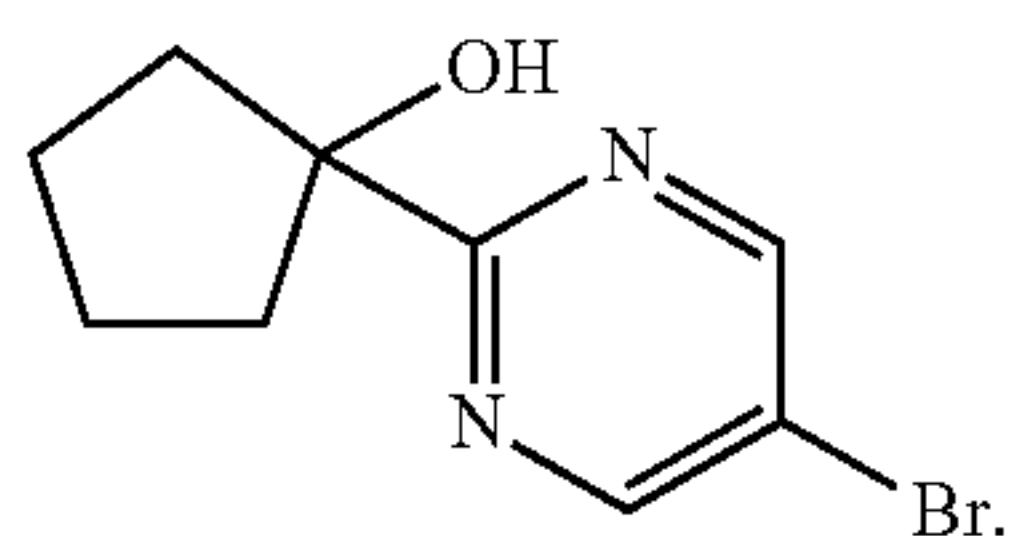
MS 242.88 [\text{M} + \text{H}]^+ 1-(5-bromopyrimidin-2-yl) cyclopentanol
