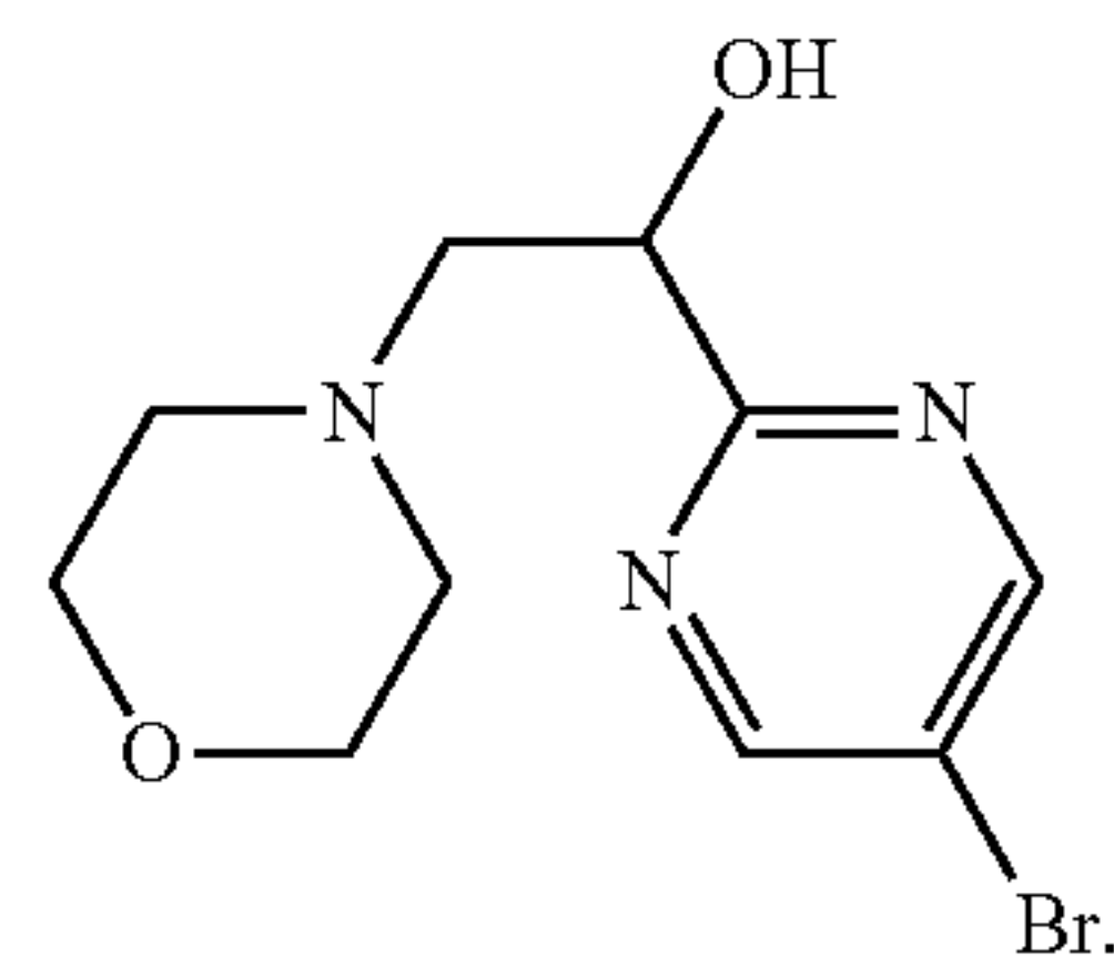
MS 288.05 & 290.01 [\text{M} + \text{H}]^+ 1-(5-bromopyrimidin-2-yl)- 2-morpholino-ethanol
