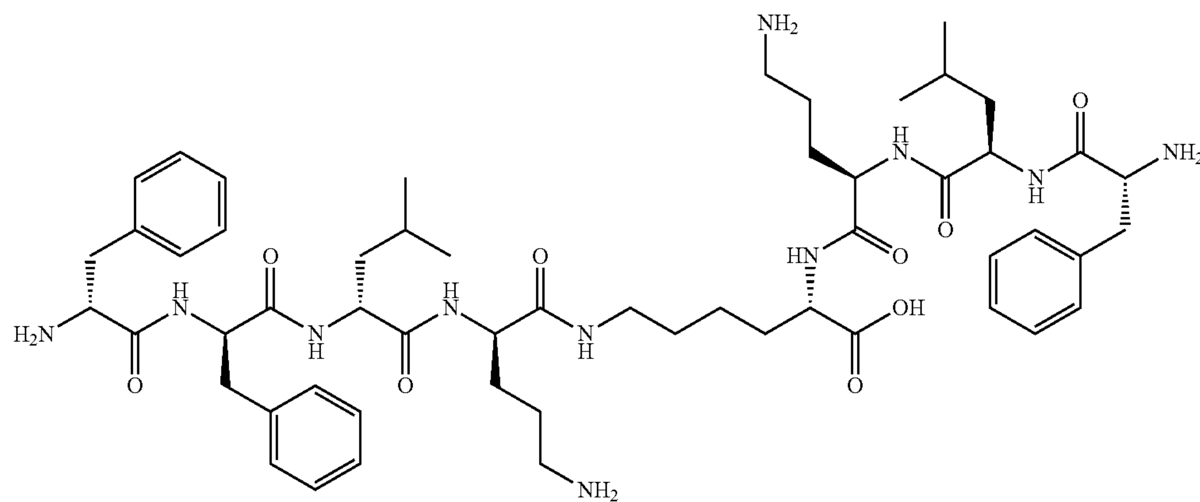
Compound (79): D-Phe-D-Phe-D-Leu-D-Orn-εLys-OH
